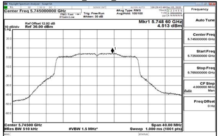
802.11ax_20MHz_5745MHz-106-53
