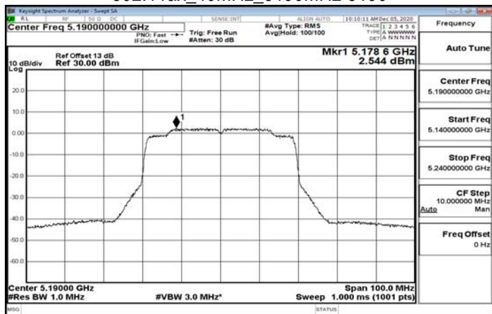
802.11ax_40MHz_5190MHz-5190
