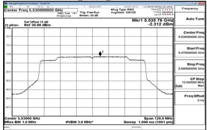
802.11ax_80MHz_5530MHz-5530
