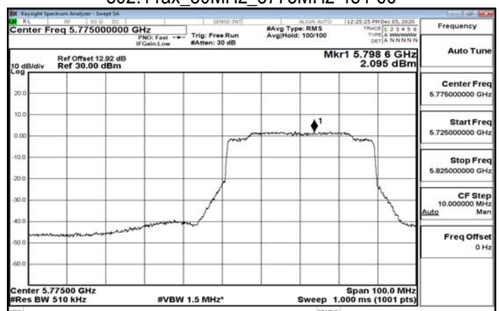
802.11ax_80MHz_5775MHz-484-66
