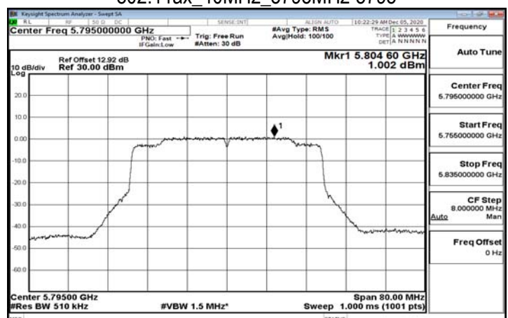
802.11ax_40MHz_5795MHz-5795
