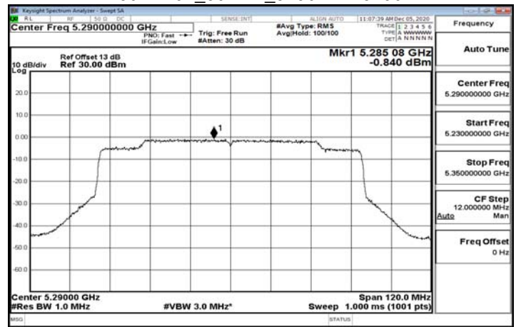
802.11ax_80MHz_5290MHz-484-66
