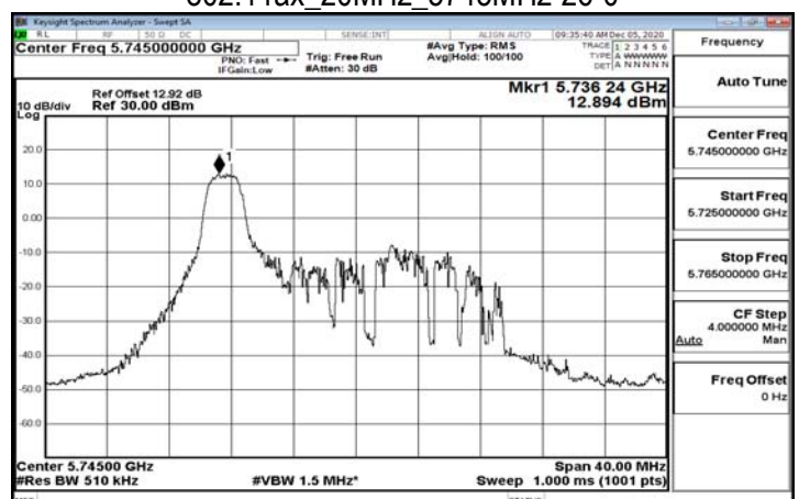
802.11ax_20MHz_5745MHz-26-0
