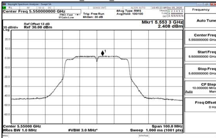
802.11n_40MHz_5550MHz-5550
