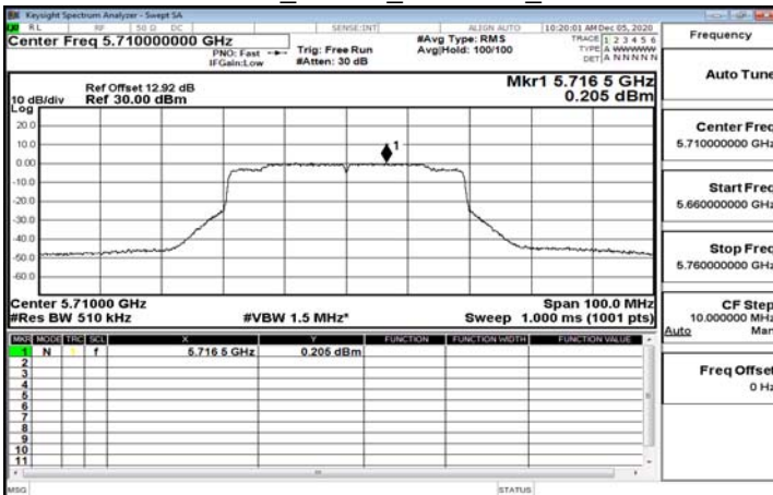
802.11ax_40MHz_5710MHz_UNII 3
