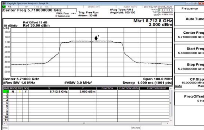
802.11ax_40MHz_5710MHz_UNII 3
