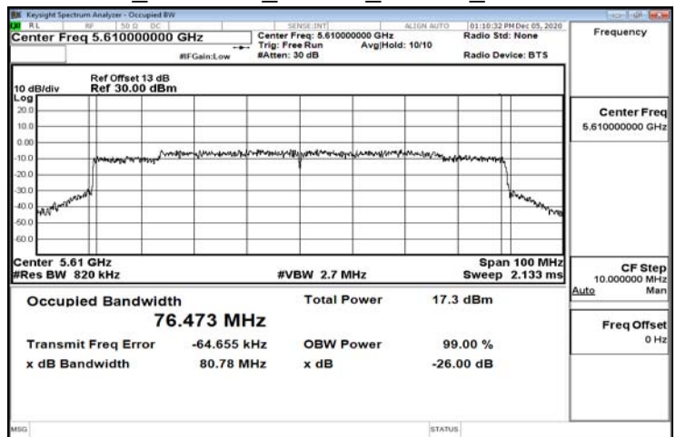
FCC_802.11ax_80MHz_Chain0_5610MHz
