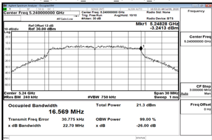
FCC_802.11a_20MHz_Chain0_5240MHz
