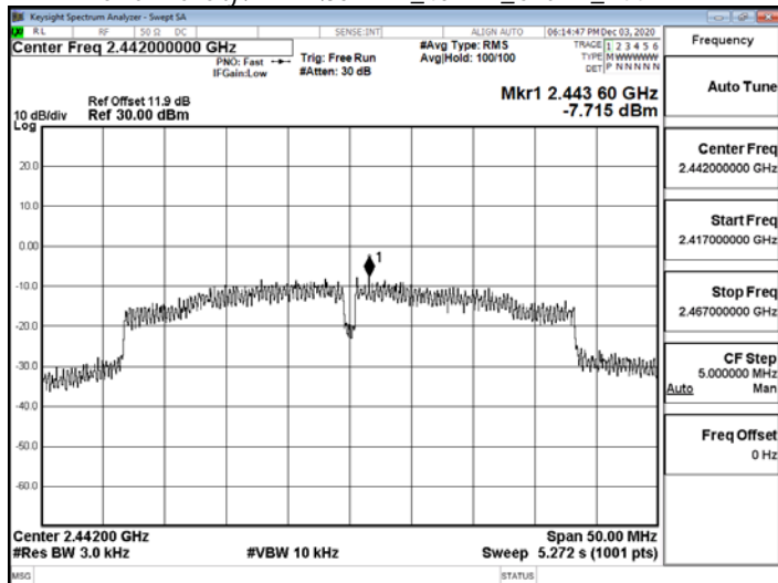
Power DensityWLAN\802.11n_40MHz_Chain1_2442MHz
