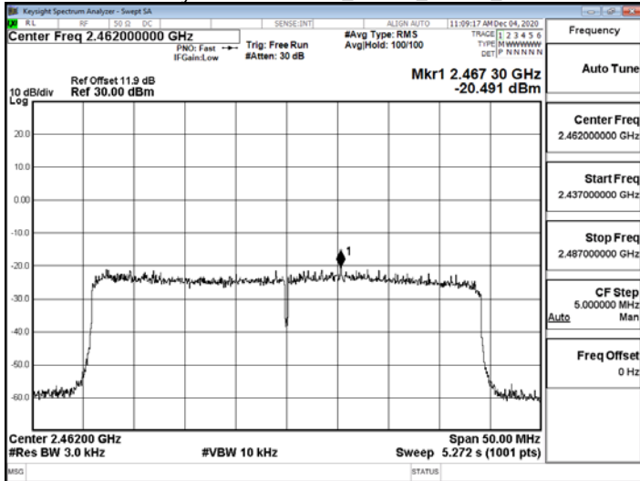
Power Density\WLAN\802.11ax_40MHz_Chain0_2462MHz_RU242_62
