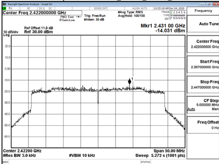
Power Density\WLAN\802.11ax_40MHz_Chain1_2422MHz
