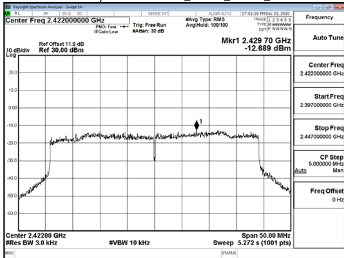
Power Density\WLAN\802.11ax_40MHz_Chain1_2422MHz_RU242_61
