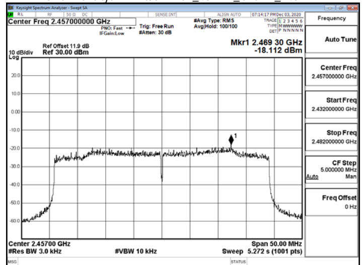
Power Density\WLAN\802.11ax_40MHz_Chain1_2457MHz
