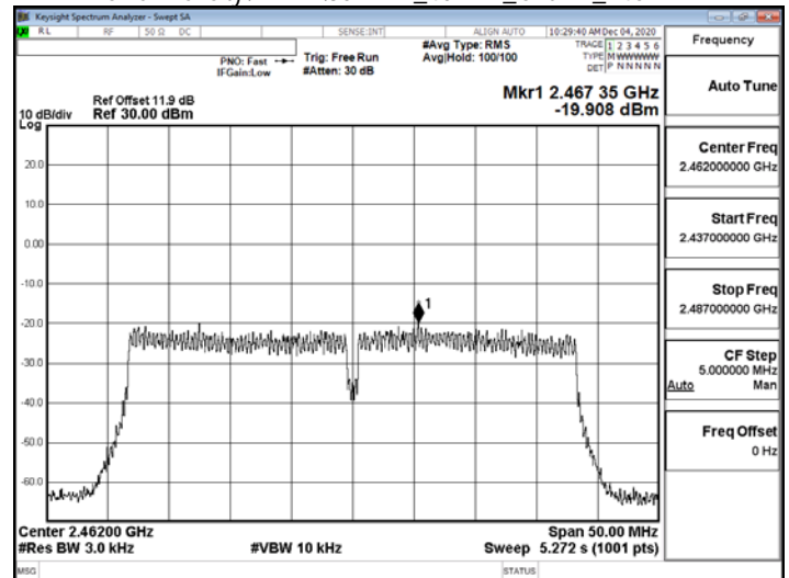
Power DensityWLAN\802.11n_40MHz_Chain1_2462MHz
