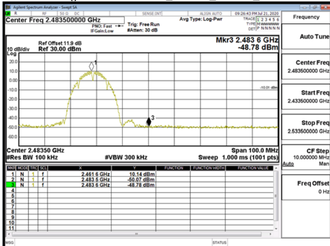
Band EdgeWLAN\802.11b_20MHz_Chain0_2467MHz
