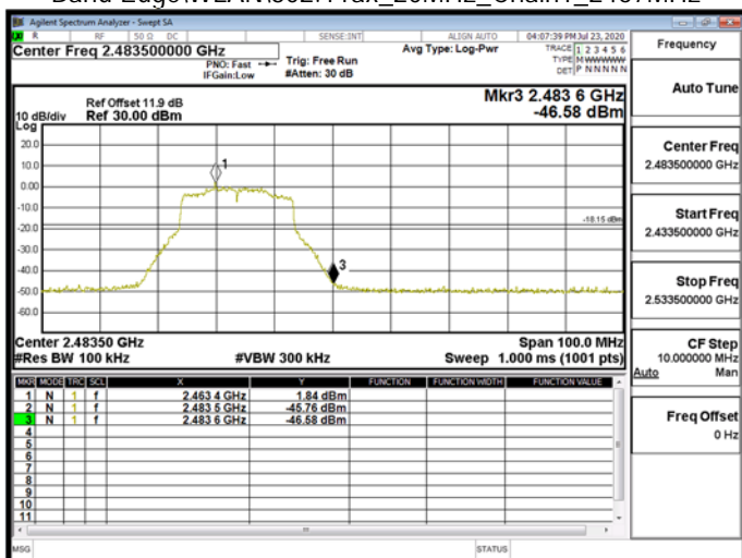
Band Edge\WLAN\802.11ax_20MHz_Chain1_2467MHz
