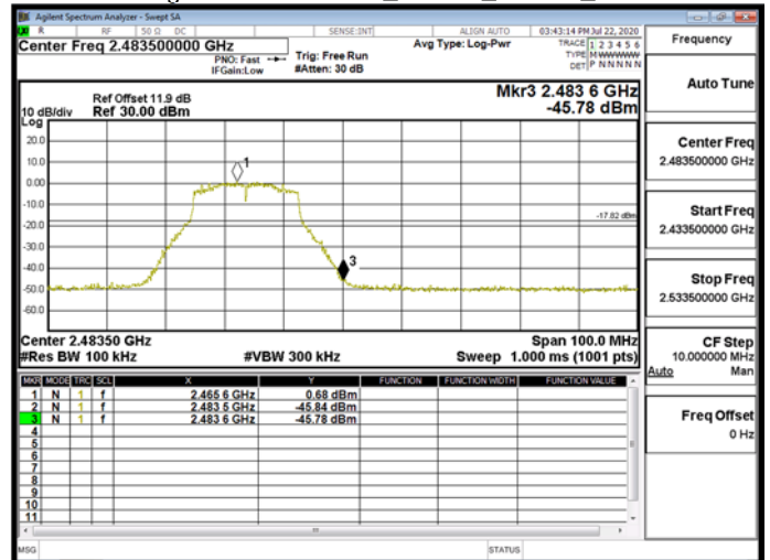
Band EdgeWLAN\802.11n_20MHz_Chain0_2472MHz
