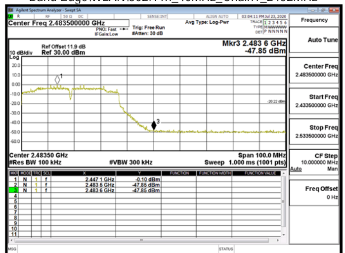
Band Edge\WLAN\802.11n_40MHz_Chain1_2452MHz
