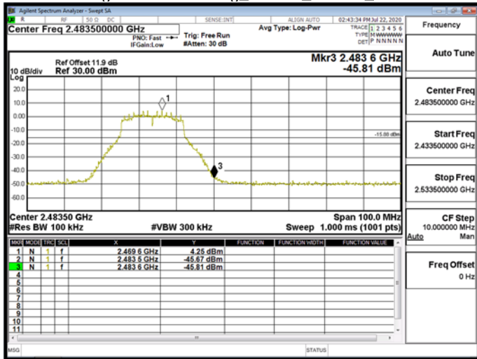
Band EdgeWLAN\802.11g_20MHz_Chain0_2472MHz
