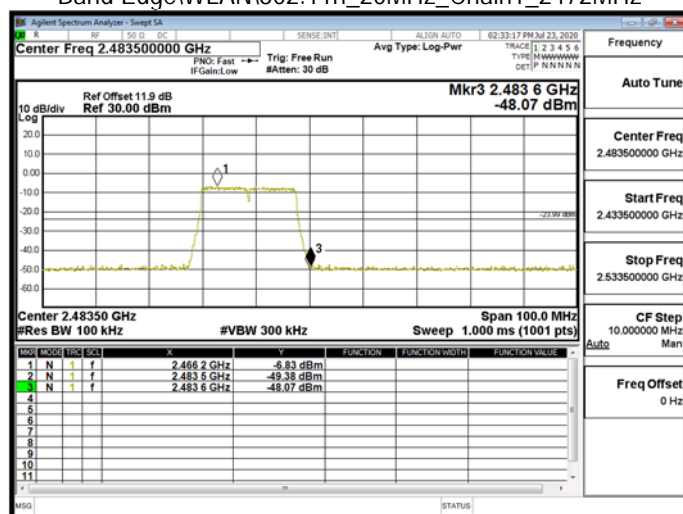
Band EdgeWLAN\802.11n_20MHz_Chain1_2472MHz
