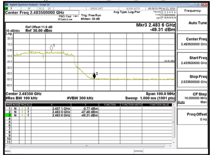
Band Edge\WLAN\802.11ax_40MHz_Chain0_2457MHz
