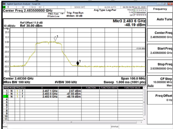
Band Edge\WLAN\802.11ax_20MHz_Chain0_2467MHz
