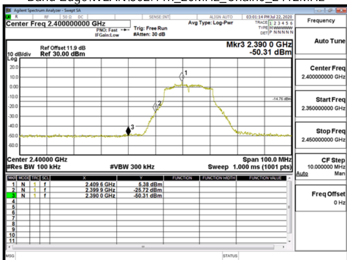
Band EdgeWLAN\802.11n_20MHz_Chain0_2412MHz
