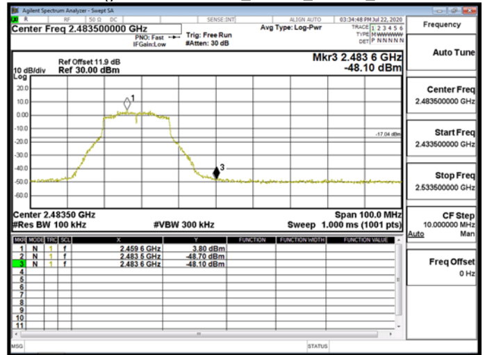
Band EdgeWLAN\802.11n_20MHz_Chain0_2467MHz
