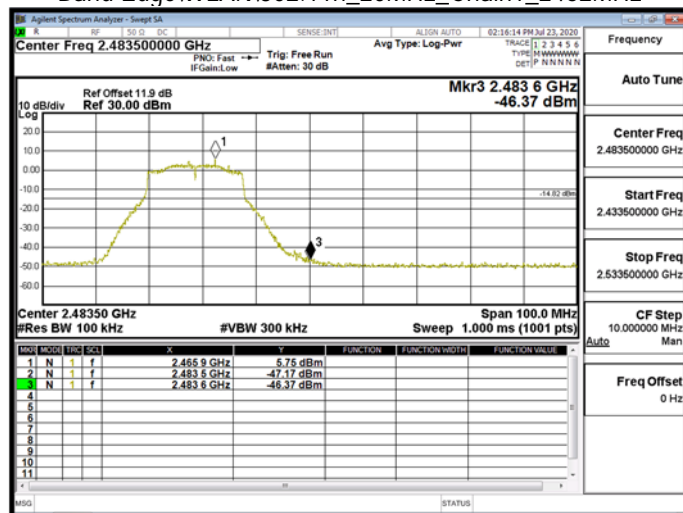
Band EdgeWLAN\802.11n_20MHz_Chain1_2467MHz
