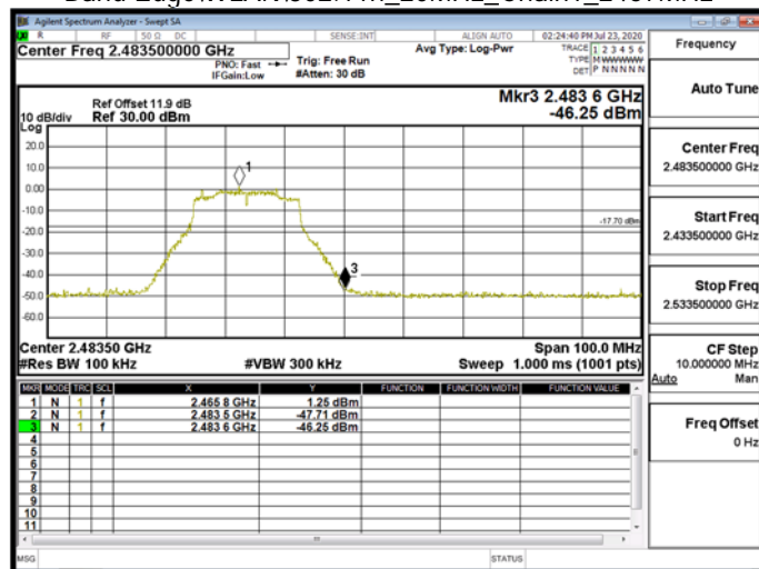
Band EdgeWLAN\802.11n_20MHz_Chain1_2472MHz
