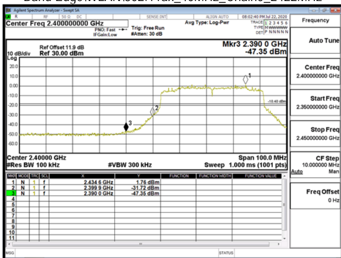
Band Edge\WLAN\802.11ax_40MHz_Chain0_2422MHz
