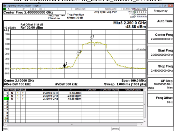
Band EdgeWLAN\802.11n_20MHz_Chain1_2412MHz
