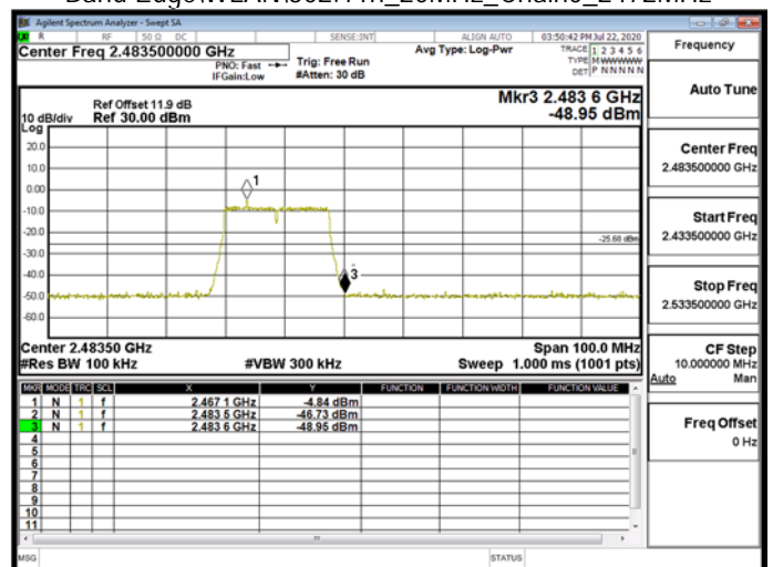
Band EdgeWLAN\802.11n_20MHz_Chain0_2472MHz
