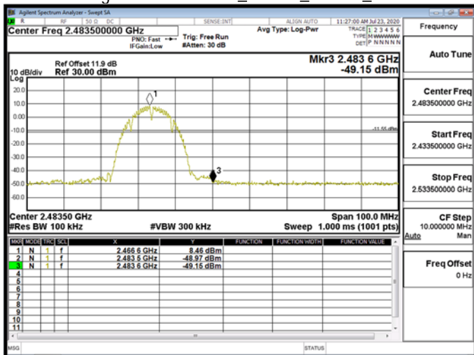
Band EdgeWLAN\802.11b_20MHz_Chain1_2467MHz
