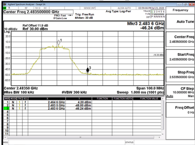
Band Edge\WLAN\802.11ax_20MHz_Chain1_2467MHz
