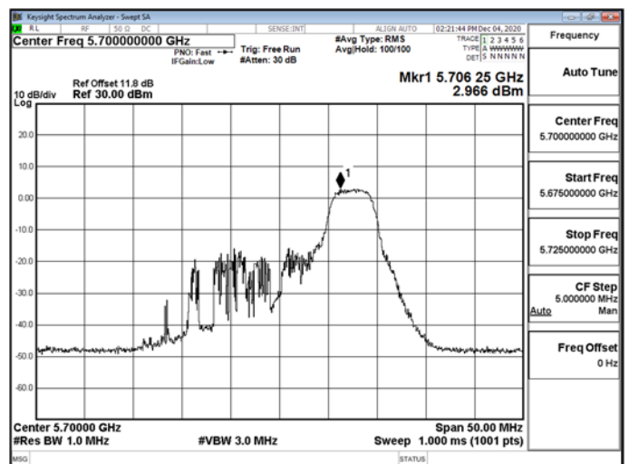
802.11ax_20MHz_RU_52_40_CH1_5700MHz-5700
