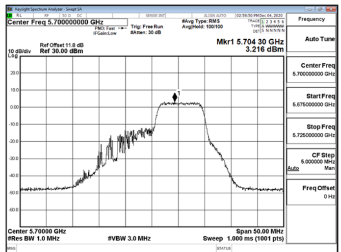
802.11ax_20MHz_RU_106_54_CH0_5700MHz-5700
