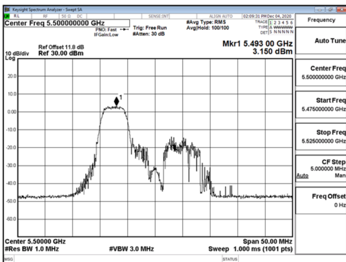
802.11ax_20MHz_RU_52_37_CH0_5500MHz-5500
