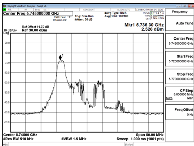
802.11ax_20MHz_RU_26_0_CH1_5745MHz-5745
