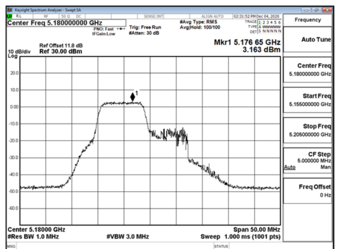
802.11ax_20MHz_RU_106_53_CH0_5180MHz-5180
