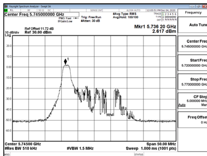
802.11ax_20MHz_RU_26_0_CH0_5745MHz-5745
