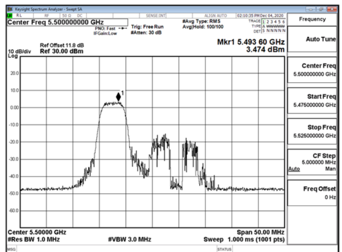
802.11ax_20MHz_RU_52_37_CH1_5500MHz-5500
