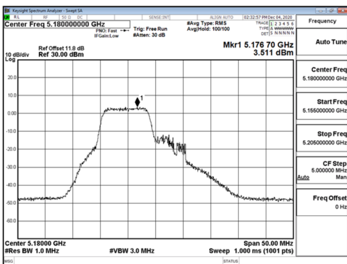
802.11ax_20MHz_RU_106_53_CH1_5180MHz-5180
