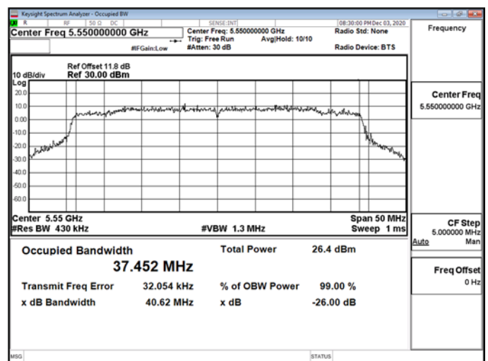
802.11ax_40MHz_Chain0_5550MHz
