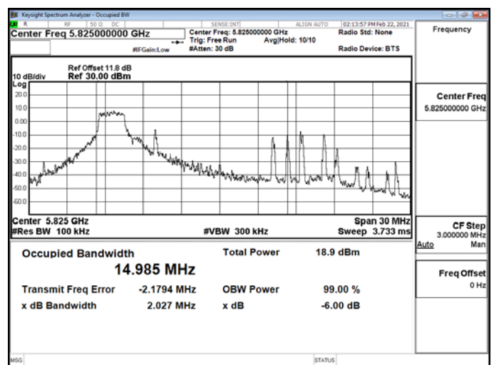
802.11ax_20MHz_Chain0_5825MHz_R26_0
