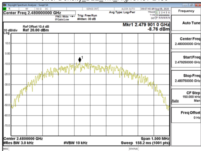
Power Density_BLE_1M_HighCH39-2480
