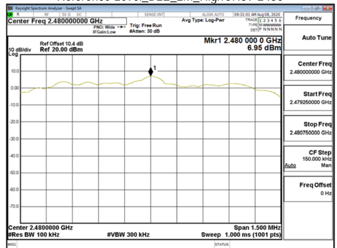
Reference Level_BLE_2M_HighCH39-2480
