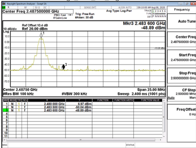
Band Edge_BLE_1M_HighCH39-2480
