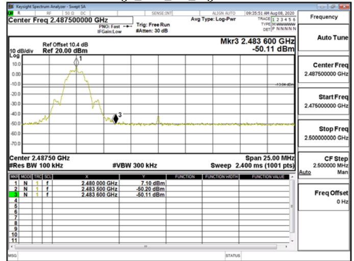
Band Edge_BLE_2M_HighCH39-2480
