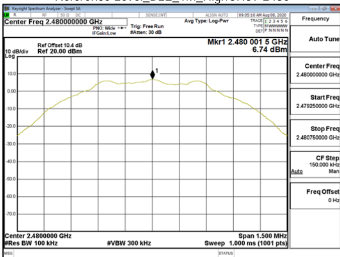
Reference Level_BLE_1M_HighCH39-2480
