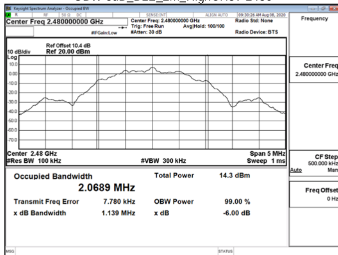
OBW 6dB_BLE_2M_HighCH39-2480
