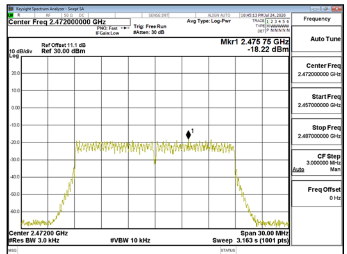
Power Density\WLAN\802.11n_20MHz_Chain1_2472MHz
