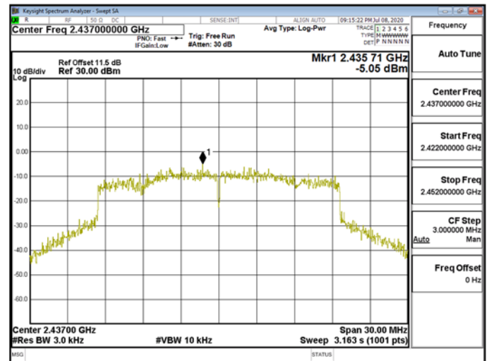
Power DensityWLAN\802.11ax_20MHz_Chain1_2437MHz
