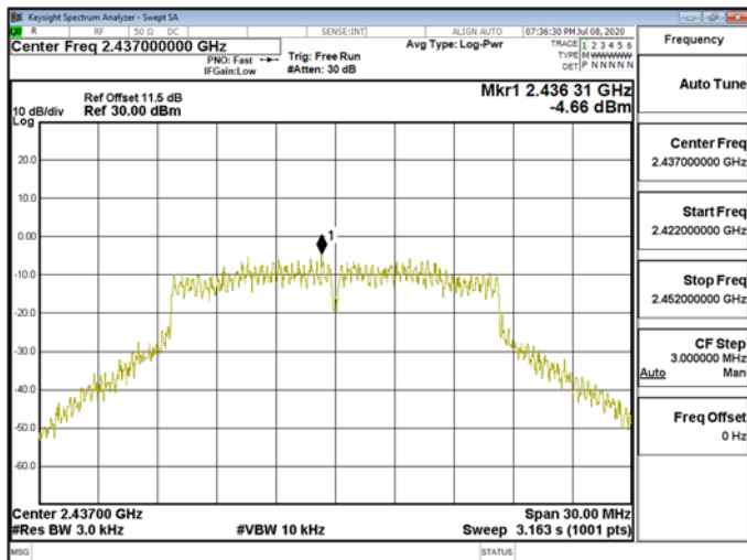
Power Density\WLAN\802.11g_20MHz_Chain1_2437MHz
