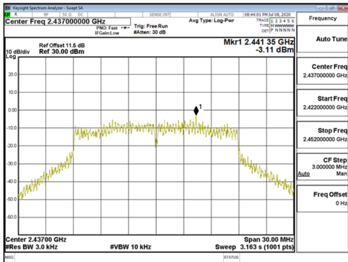
Power Density\WLAN\802.11n_20MHz_Chain1_2437MHz
