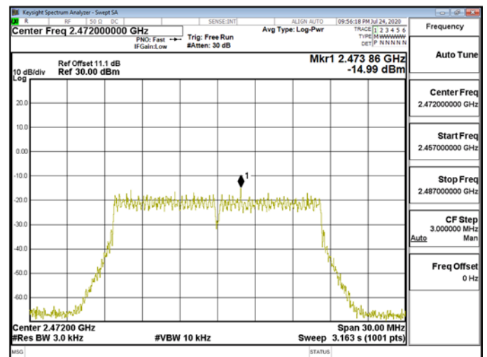
Power Density\WLAN\802.11g_20MHz_Chain1_2472MHz
