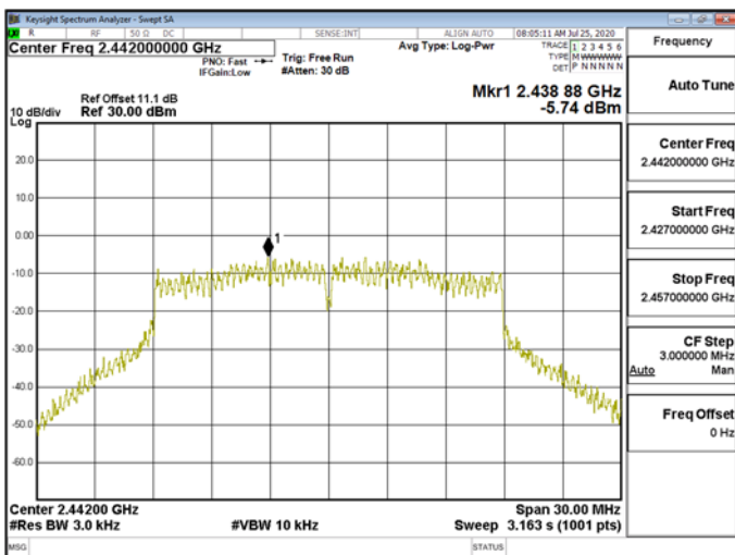
Power Density\WLAN\802.11n_20MHz_Chain1_2442MHz
