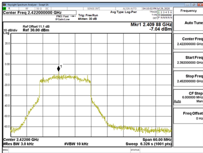
Power DensityWLAN\802.11ax_40MHz_Chain1_2422MHz_RU242_61
