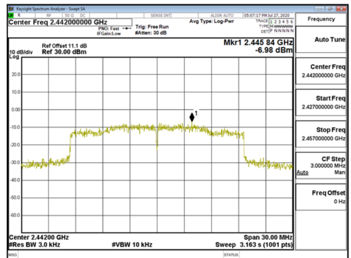
Power Density\WLAN\802.11ax_20MHz_Chain0_2442MHz
