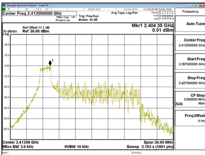
Power DensityWLAN\802.11ax_20MHz_Chain1_2412MHz_RU26_0
