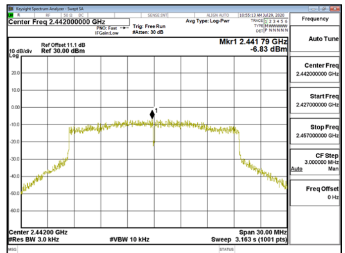
Power DensityWLAN\802.11ax_20MHz_Chain1_2442MHz
