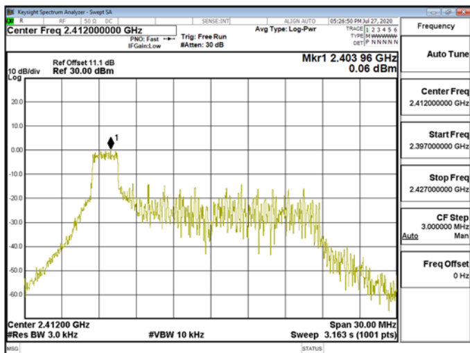
Power DensityWLAN\802.11ax_20MHz_Chain1_2412MHz_RU26_0
