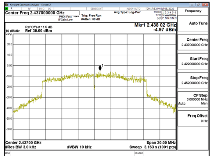
Power Density\WLAN\802.11ax_20MHz_Chain0_2437MHz
