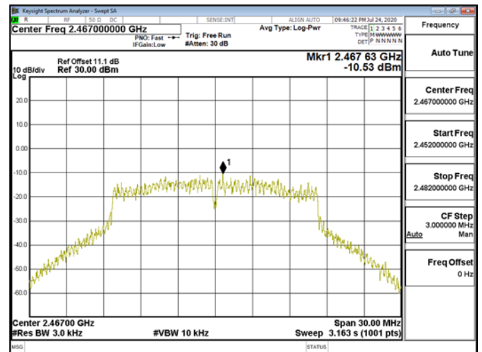
Power Density\WLAN\802.11g_20MHz_Chain1_2467MHz
