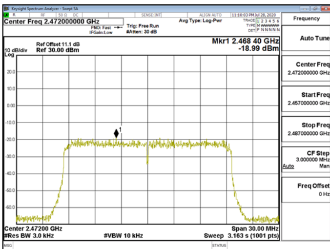
Power Density\WLAN\802.11ax_20MHz_Chain1_2472MHz
