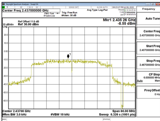
Power DensityWLAN\802.11ax_40MHz_Chain1_2437MHz
