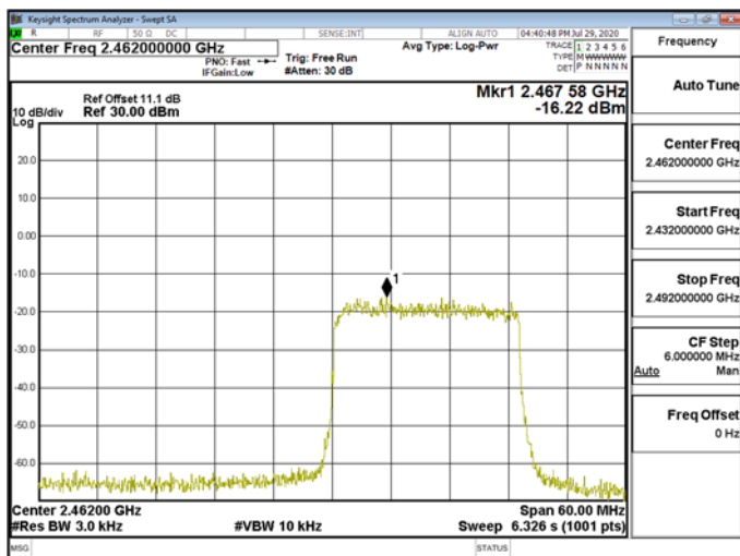
Power DensityWLAN\802.11ax_40MHz_Chain1_2462MHz_RU242_62
