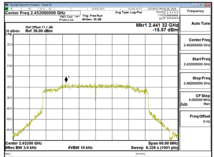
Power DensityWLAN\802.11ax_40MHz_Chain1_2452MHz
