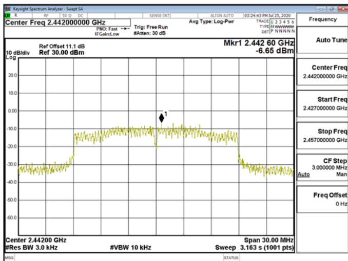
Power Density\WLAN\802.11n_20MHz_Chain1_2442MHz
