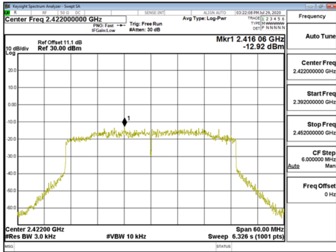
Power DensityWLAN\802.11ax_40MHz_Chain1_2422MHz_RU242_61
