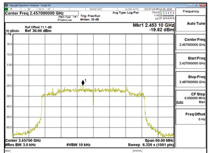
Power DensityWLAN\802.11ax_40MHz_Chain1_2457MHz
