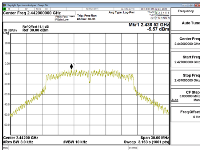
Power Density\WLAN\802.11g_20MHz_Chain1_2442MHz
