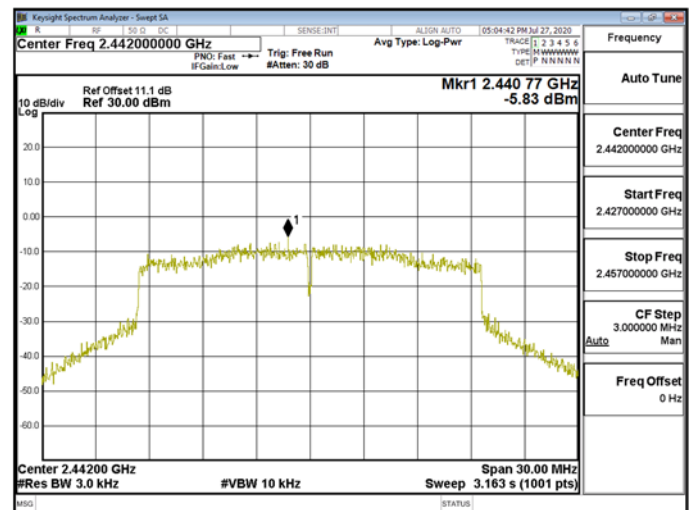
Power DensityWLAN\802.11ax_20MHz_Chain1_2442MHz
