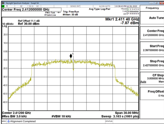
Power DensityWLAN\802.11ax_20MHz_Chain1_2412MHz_RU106_53
