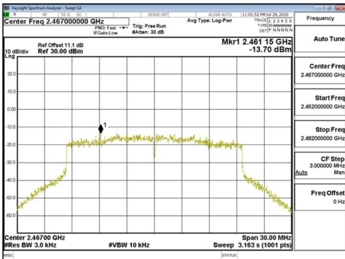
Power Density\WLAN\802.11ax_20MHz_Chain1_2467MHz
