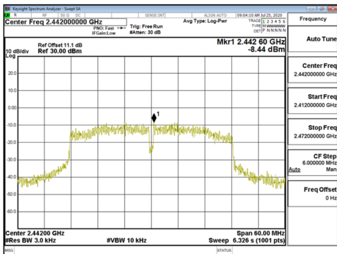
Power Density\WLAN\802.11n_40MHz_Chain1_2442MHz
