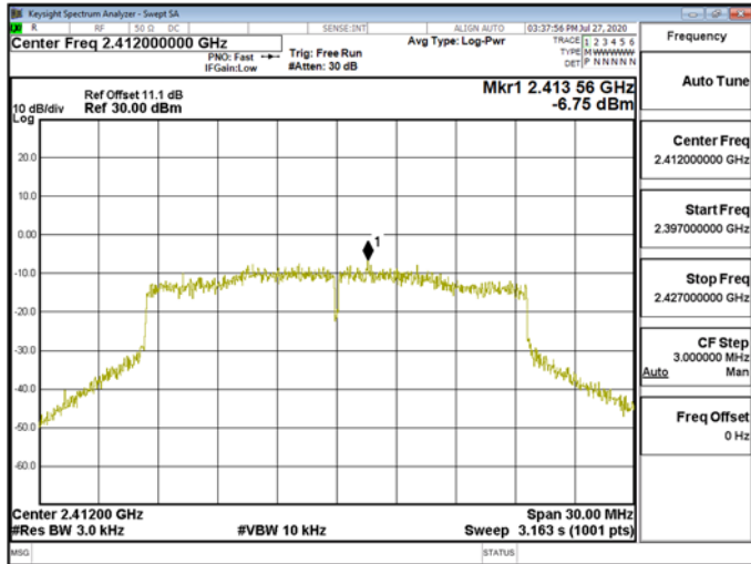
Power DensityWLAN\802.11ax_20MHz_Chain1_2412MHz_RU106_53
