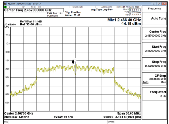
Power Density\WLAN\802.11n_20MHz_Chain1_2467MHz
