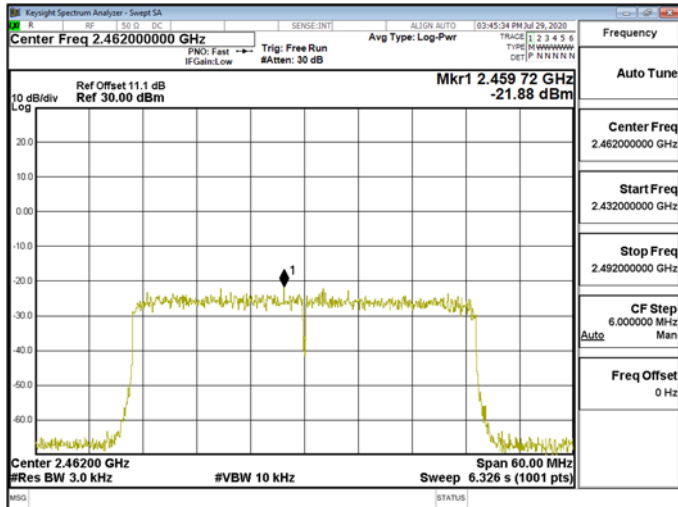
Power DensityWLAN\802.11ax_40MHz_Chain1_2462MHz_RU242_62
