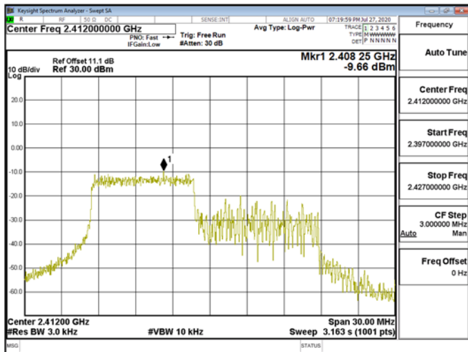
Power Density\WLAN\802.11ax_20MHz_Chain0_2412MHz_RU106_53
