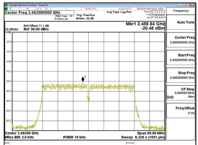
Power Density\WLAN\802.11n_40MHz_Chain1_2462MHz
