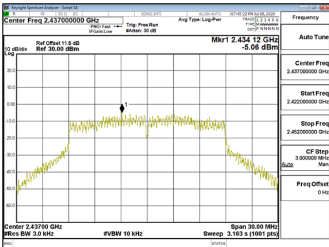
Power Density\WLAN\802.11n_20MHz_Chain1_2437MHz
