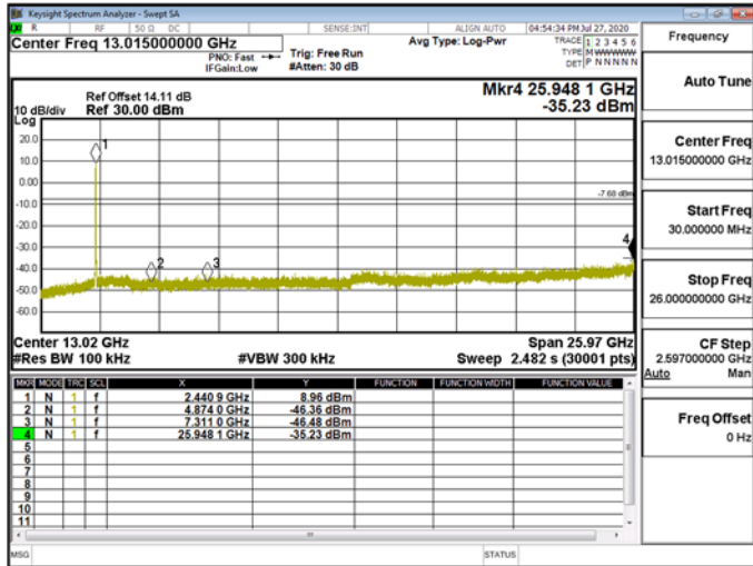
Spurious Emission\WLAN\802.11ax_20MHz_Chain1_2442MHz
