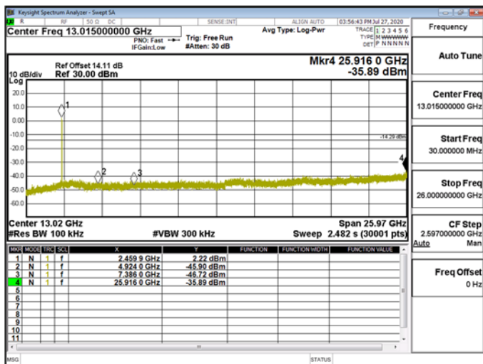
Spurious Emission\WLAN\802.11ax_20MHz_Chain1_2462MHz
