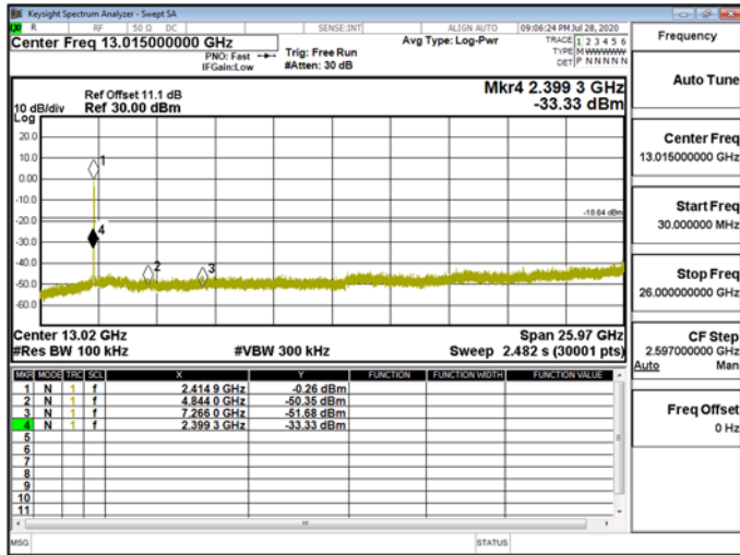
Spurious Emission\WLAN\802.11ax_40MHz_Chain0_2437MHz
