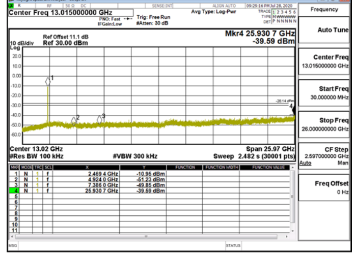
Spurious Emission\WLAN\802.11ax_40MHz_Chain0_2462MHz
