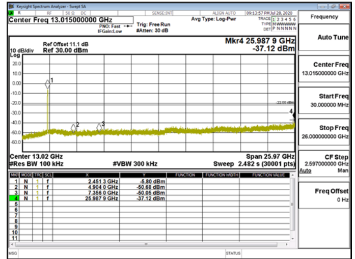
Spurious Emission\WLAN\802.11ax_40MHz_Chain0_2457MHz
