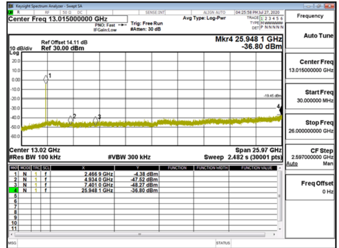
Spurious Emission\WLAN\802.11ax_20MHz_Chain1_2472MHz
