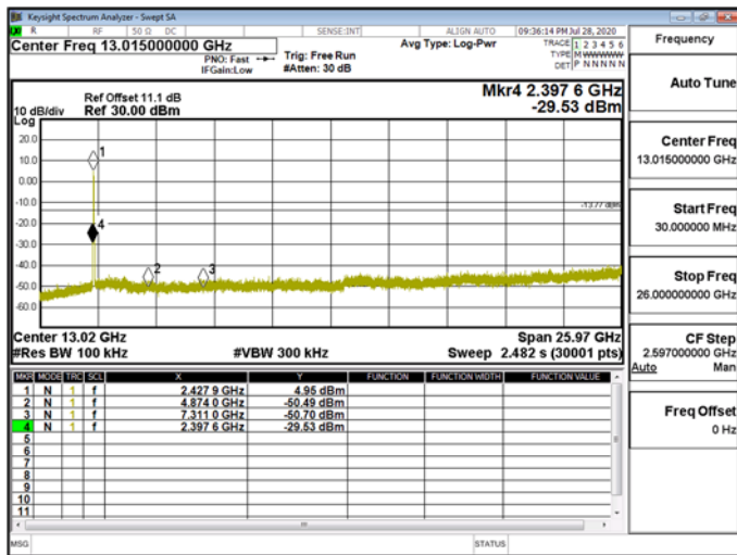
Spurious Emission\WLAN\802.11ax_40MHz_Chain0_2442MHz
