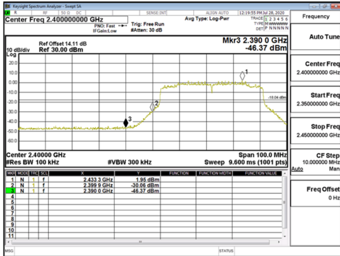
Band Edge\WLAN\802.11ax_40MHz_Chain1_2422MHz_RU242_61
