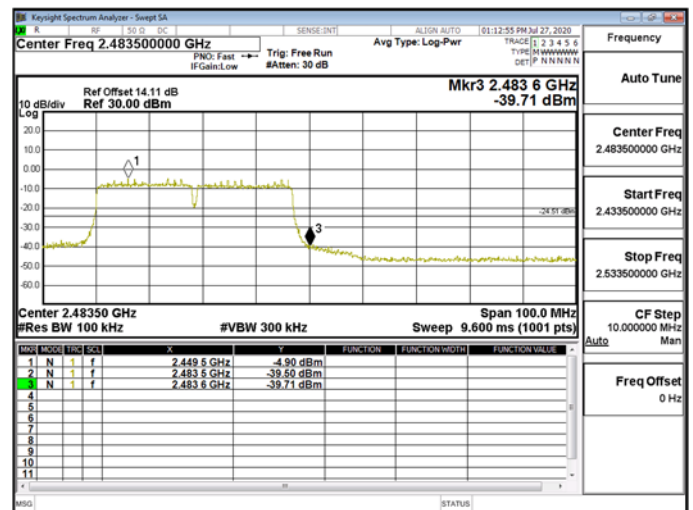
Band Edge\WLAN\802.11n_40MHz_Chain1_2462MHz
