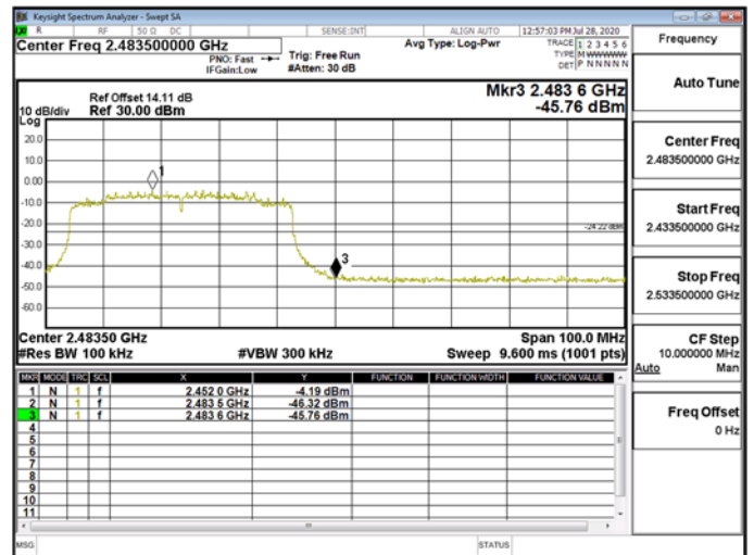
Band Edge\WLAN\802.11ax_40MHz_Chain1_2457MHz_RU242_62
