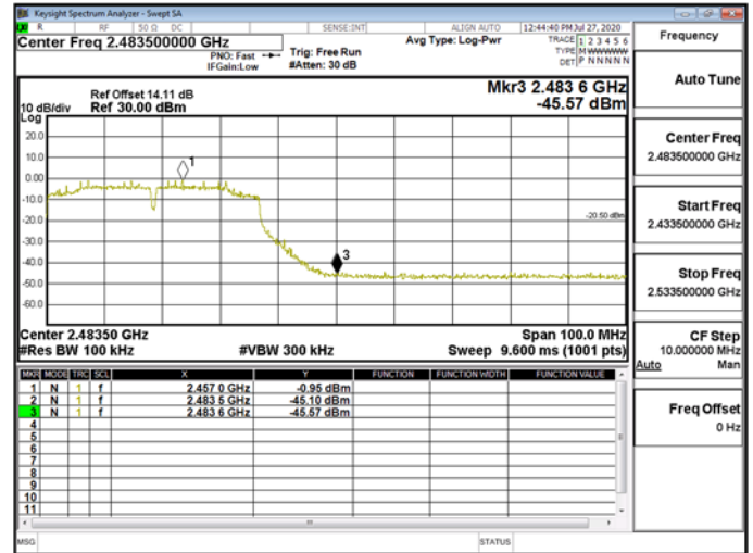
Band Edge\WLAN\802.11n_40MHz_Chain1_2457MHz
