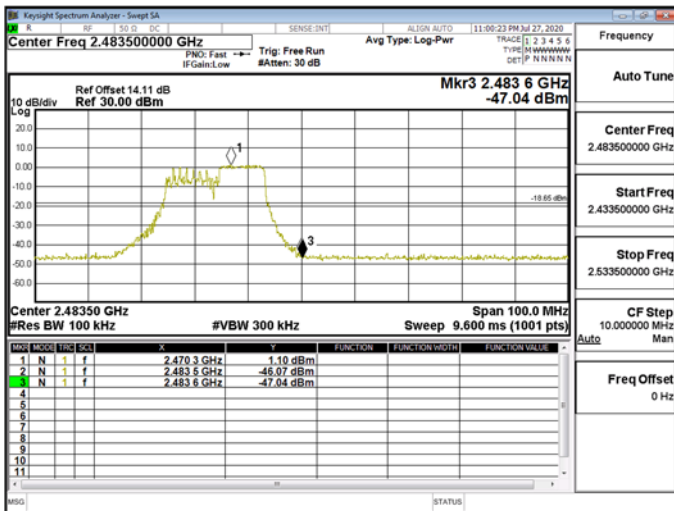
Band Edge\WLAN\802.11ax_20MHz_Chain1_2467MHz_RU26_8
