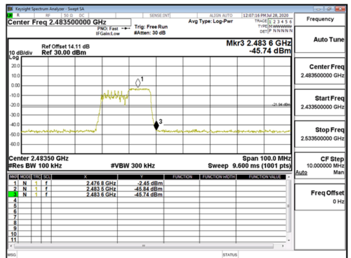
Band Edge\WLAN\802.11ax_20MHz_Chain1_2472MHz_RU106_54
