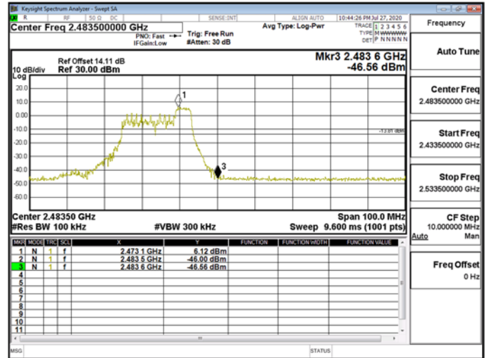
Band Edge\WLAN\802.11ax_20MHz_Chain1_2472MHz
