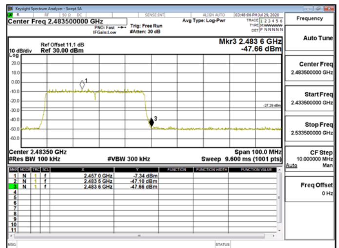
Band Edge\WLAN\802.11ax_40MHz_Chain1_2462MHz
