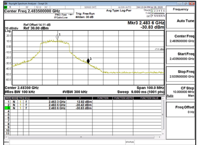
Band Edge\WLAN\802.11ax_40MHz_Chain1_2457MHz
