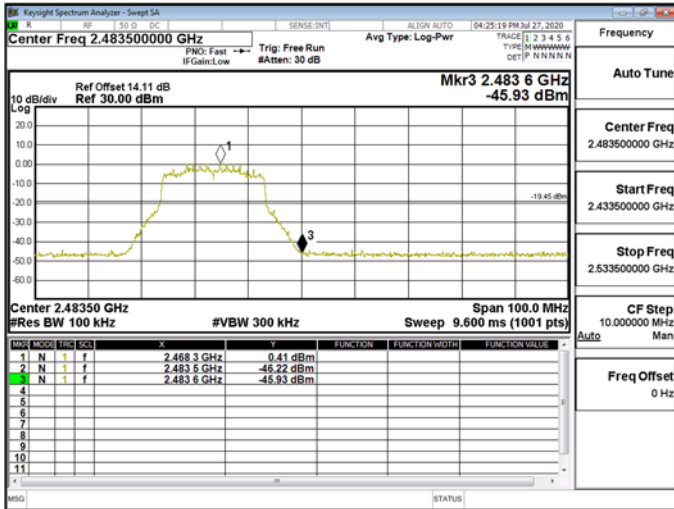
Band Edge\WLAN\802.11ax_20MHz_Chain1_2467MHz_RU106_54
