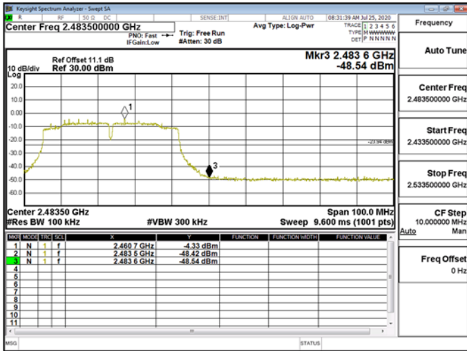
Band Edge\WLAN\802.11n_40MHz_Chain1_2462MHz
