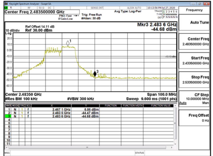
Band Edge\WLAN\802.11ax_20MHz_Chain1_2462MHz_RU26_8
