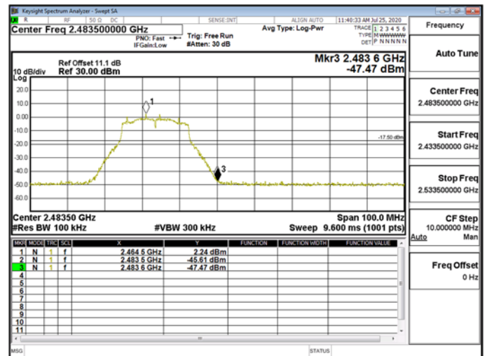
Band EdgeWLAN\802.11n_20MHz_Chain0_2472MHz
