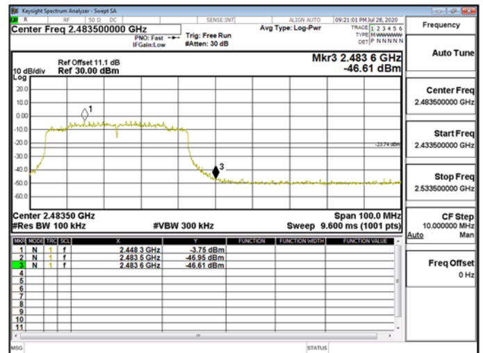
Band Edge\WLAN\802.11ax_40MHz_Chain0_2462MHz
