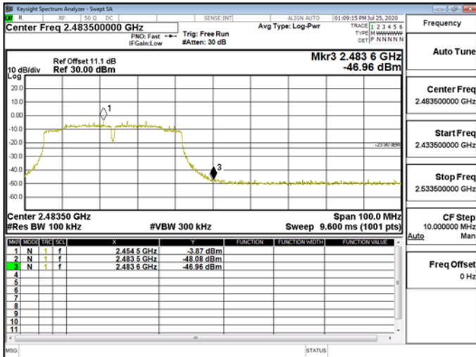
Band Edge\WLAN\802.11n_40MHz_Chain0_2462MHz
