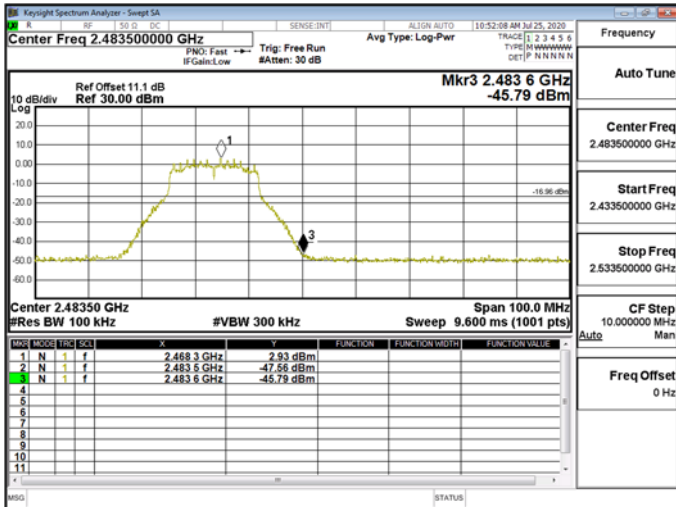
Band EdgeWLAN\802.11g_20MHz_Chain0_2472MHz
