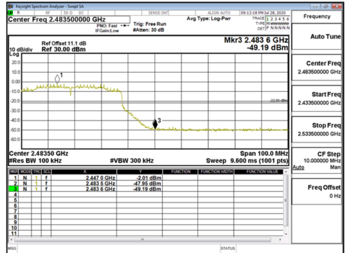
Band Edge\WLAN\802.11ax_40MHz_Chain0_2457MHz
