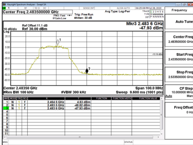
Band Edge\WLAN\802.11ax_20MHz_Chain0_2467MHz
