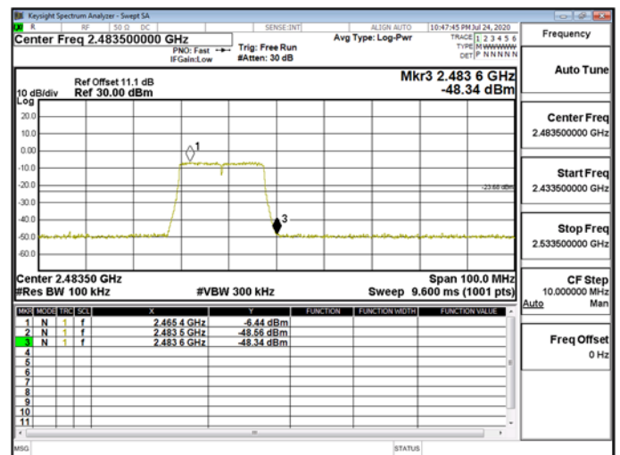
Band EdgeWLAN\802.11n_20MHz_Chain1_2472MHz
