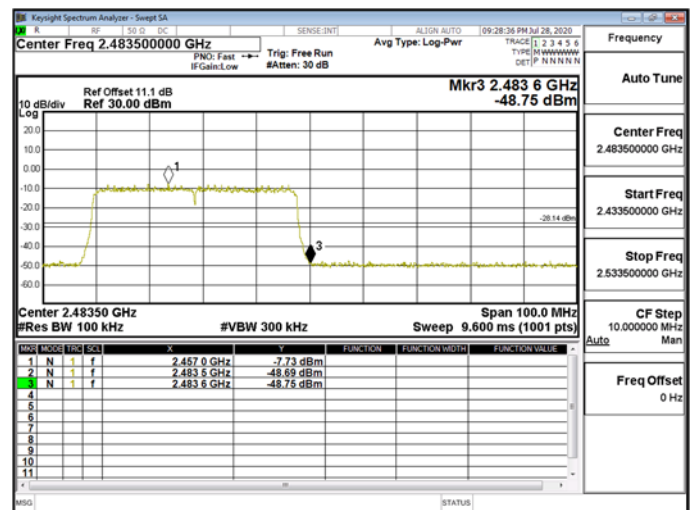
Band Edge\WLAN\802.11ax_40MHz_Chain0_2462MHz
