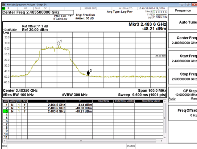
Band Edge\WLAN\802.11ax_20MHz_Chain1_2467MHz
