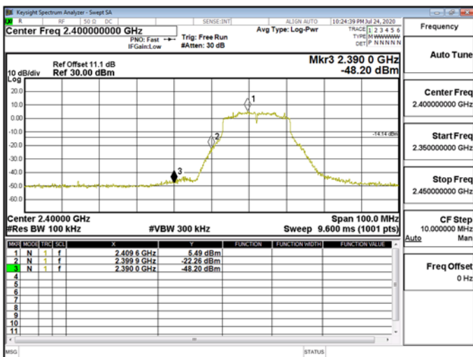
Band EdgeWLAN\802.11n_20MHz_Chain1_2412MHz
