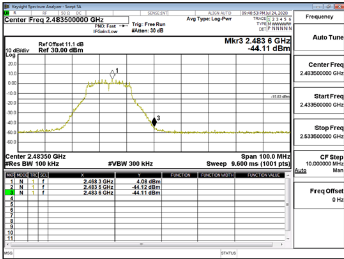
Band EdgeWLAN\802.11g_20MHz_Chain1_2472MHz
