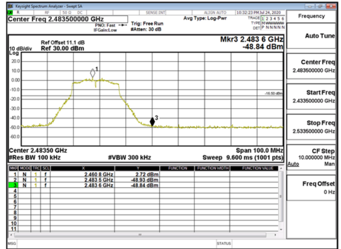
Band EdgeWLAN\802.11n_20MHz_Chain1_2467MHz
