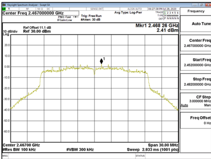
Reference Level\WLAN\802.11ax_20MHz_Chain0_2467MHz
