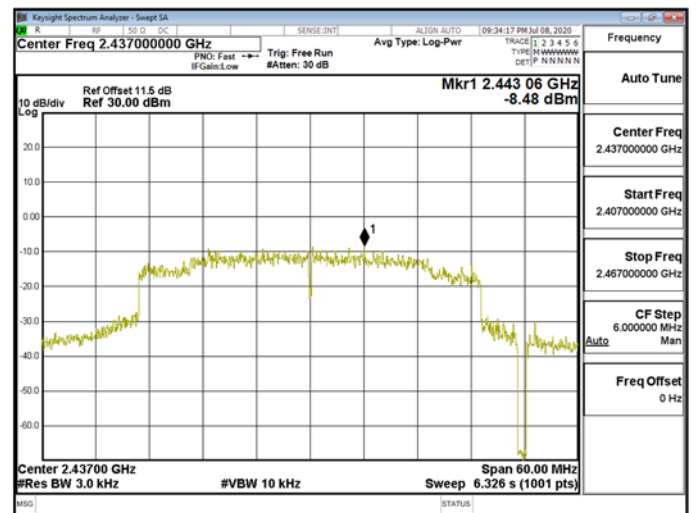
Power Density\WLAN\802.11ax_40MHz_Chain1_2437MHz
