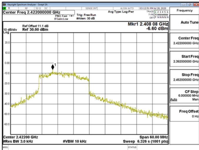
Power Density\WLAN\802.11ax_40MHz_Chain0_2422MHz_RU242_61
