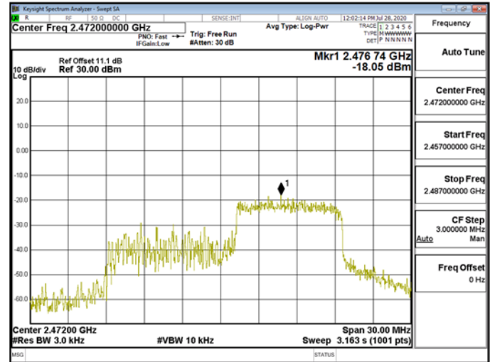
Power Density\WLAN\802.11ax_20MHz_Chain1_2472MHz_RU26_8
