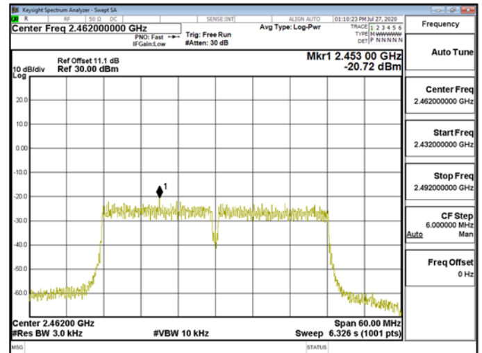
Power Density\WLAN\802.11n_40MHz_Chain1_2462MHz
