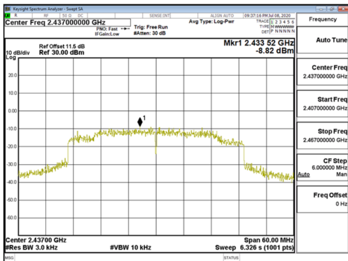
Power Density\WLAN\802.11ax_40MHz_Chain0_2437MHz
