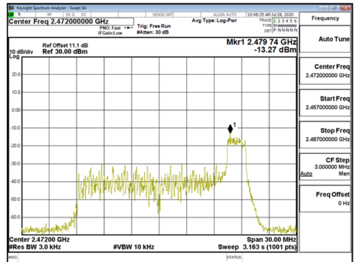
Power Density\WLAN\802.11ax_20MHz_Chain1_2472MHz_RU26_8
