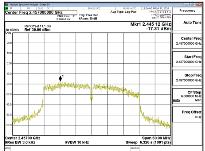
Power Density\WLAN\802.11n_40MHz_Chain1_2457MHz
