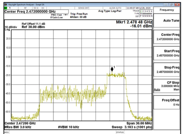
Power Density\WLAN\802.11ax_20MHz_Chain1_2472MHz_RU52_40
