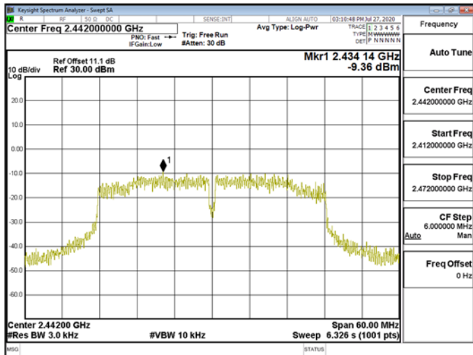
Power Density\WLAN\802.11n_40MHz_Chain1_2442MHz
