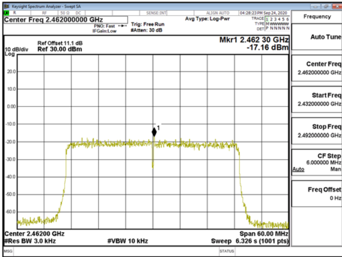
Power Density\WLAN\802.11ax_40MHz_Chain0_2462MHz_RU242_62
