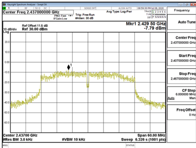
Power Density\WLAN\802.11n_40MHz_Chain0_2437MHz
