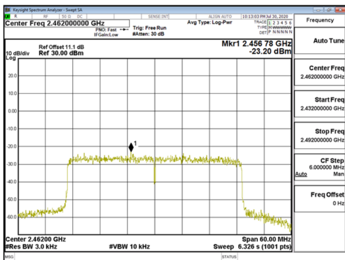
Power Density\WLAN\802.11ax_40MHz_Chain1_2462MHz
