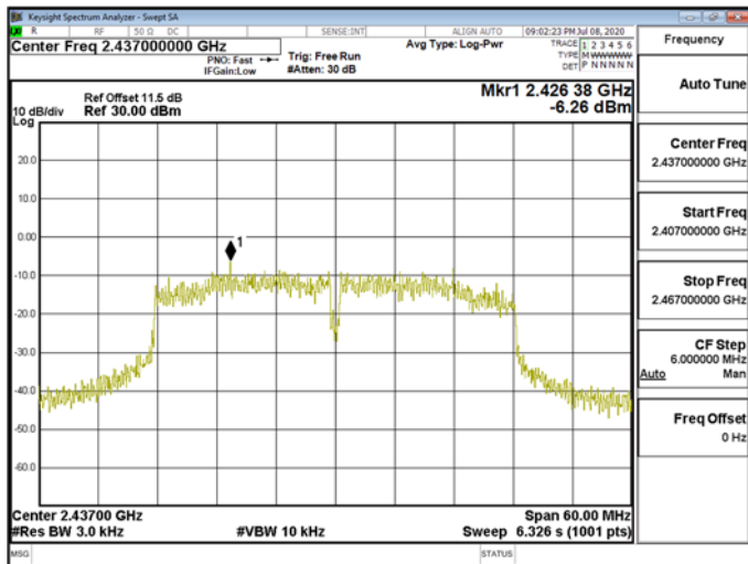
Power Density\WLAN\802.11n_40MHz_Chain1_2437MHz
