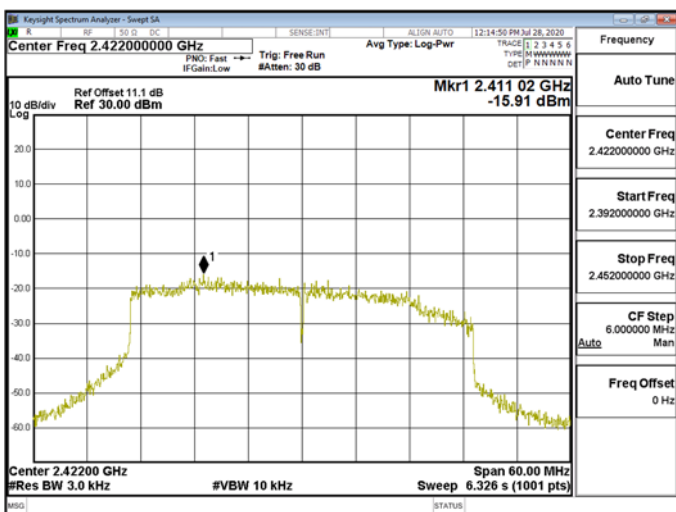
Power Density\WLAN\802.11ax_40MHz_Chain1_2422MHz
