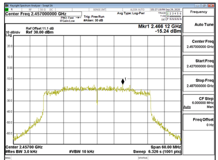
Power Density\WLAN\802.11ax_40MHz_Chain0_2457MHz
