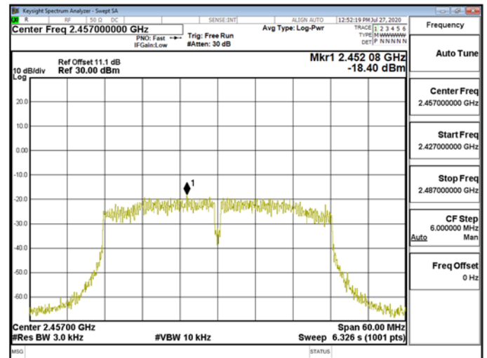
Power Density\WLAN\802.11n_40MHz_Chain0_2457MHz
