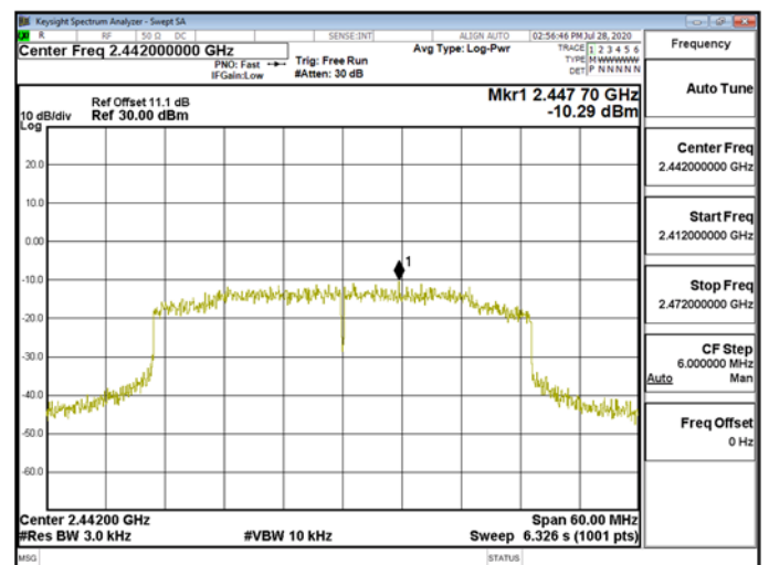
Power Density\WLAN\802.11ax_40MHz_Chain1_2442MHz
