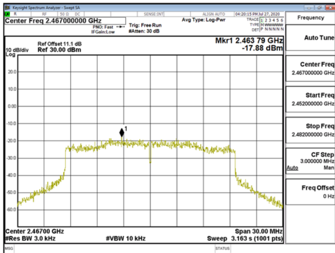
Power Density\WLAN\802.11ax_20MHz_Chain1_2467MHz
