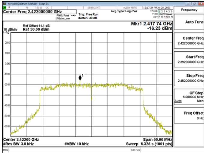
Power Density\WLAN\802.11ax_40MHz_Chain0_2422MHz_RU242_61
