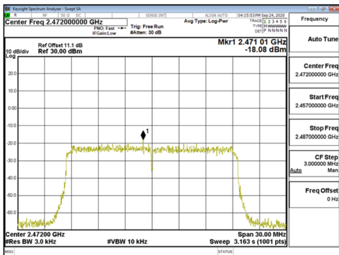
Power Density\WLAN\802.11ax_20MHz_Chain1_2472MHz
