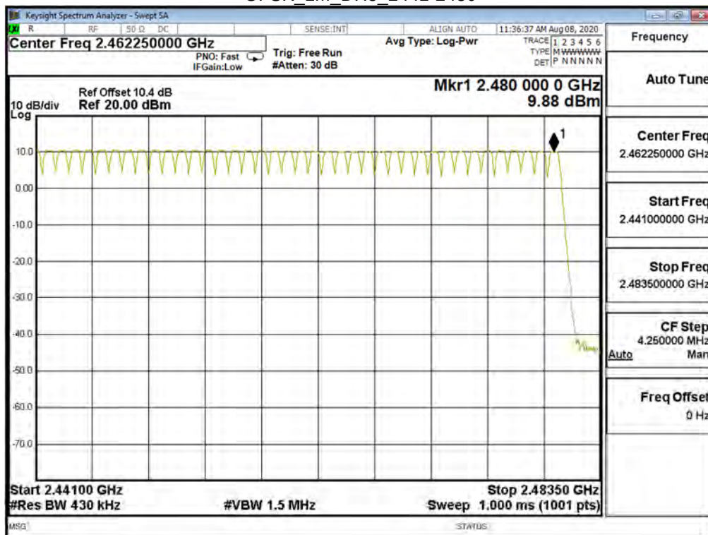
GFSK_1M_DH5_2441-2480
