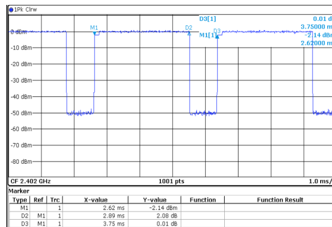
Time-domain plot for Bluetooth transmission signal
