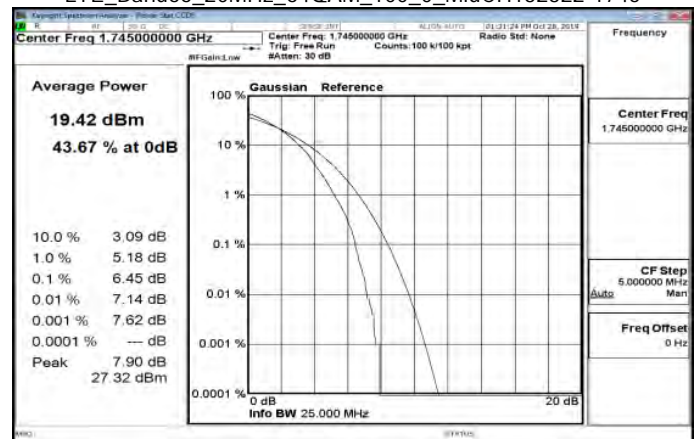
LTE_Band66_20MHz_64QAM_100_0_MidCH132322-1745
