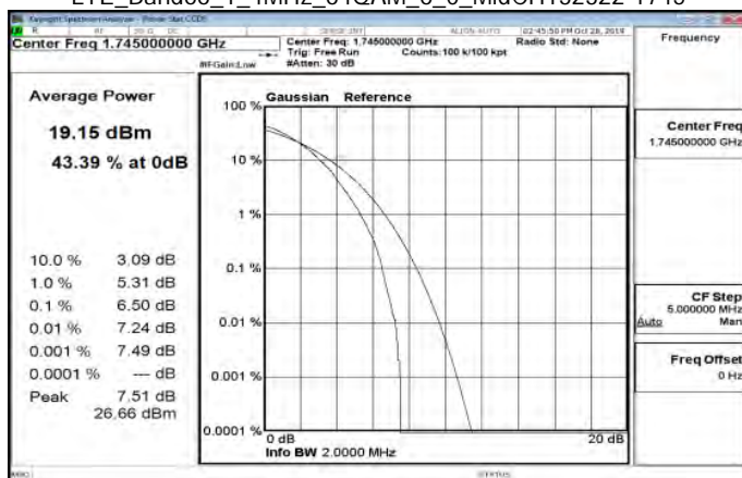
LTE_Band66_1_4MHz_64QAM_6_0_MidCH132322-1745
