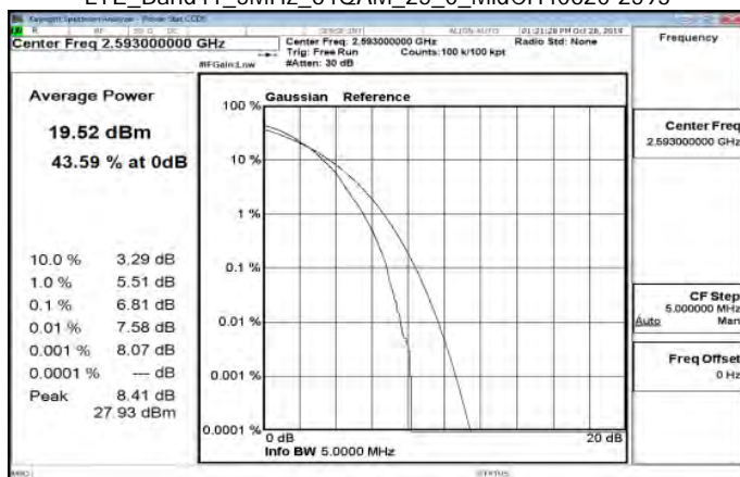
LTE_Band41_5MHz_64QAM_25_0_MidCH40620-2593
