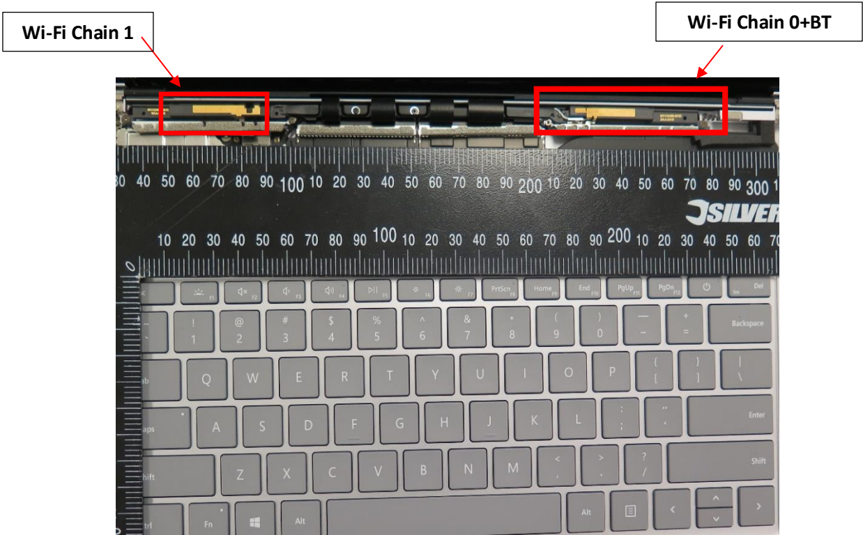
Figure 7 Wi-Fi/BT Chain 0 & 1 Antenna View
