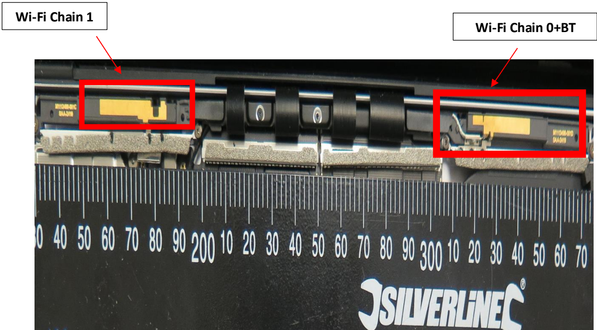
Figure 8 Close Up Antenna View
