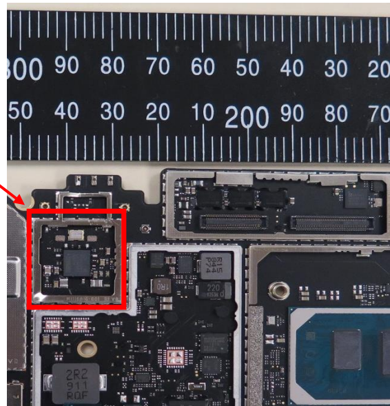
Figure 5 Close up Wi-Fi RF section without shield
