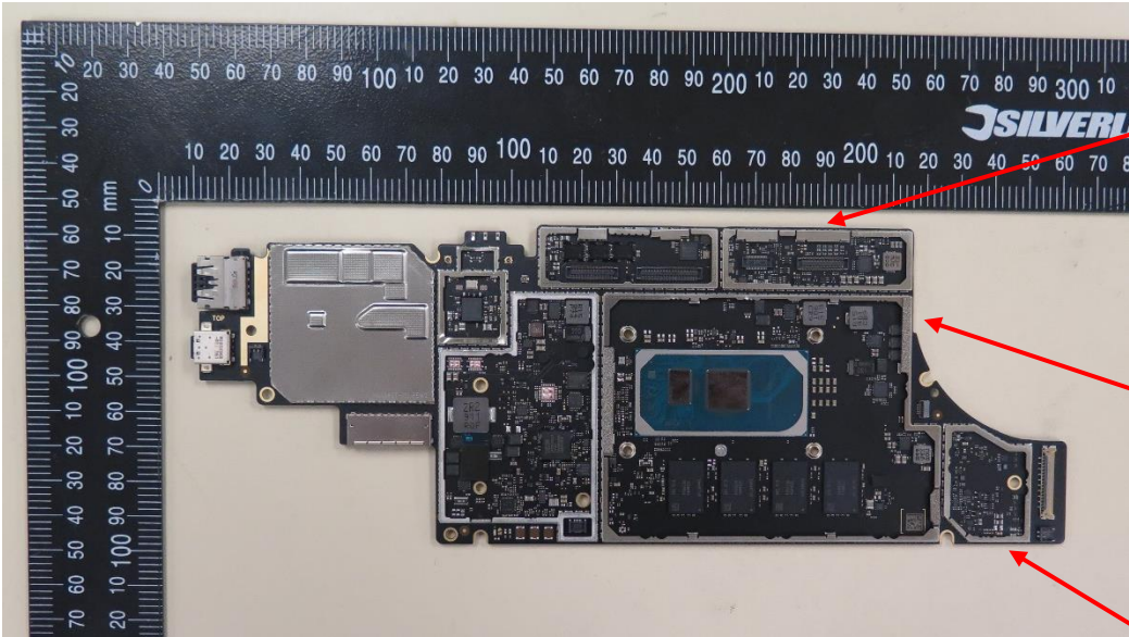
Figure 2 EUT cover off
