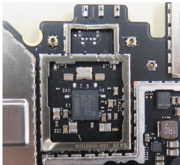
Figure 6 Close up Wi-Fi RF section -Top View
