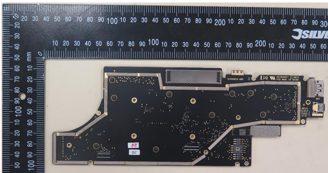
Figure 4 Main Logic Board Section-Back side
