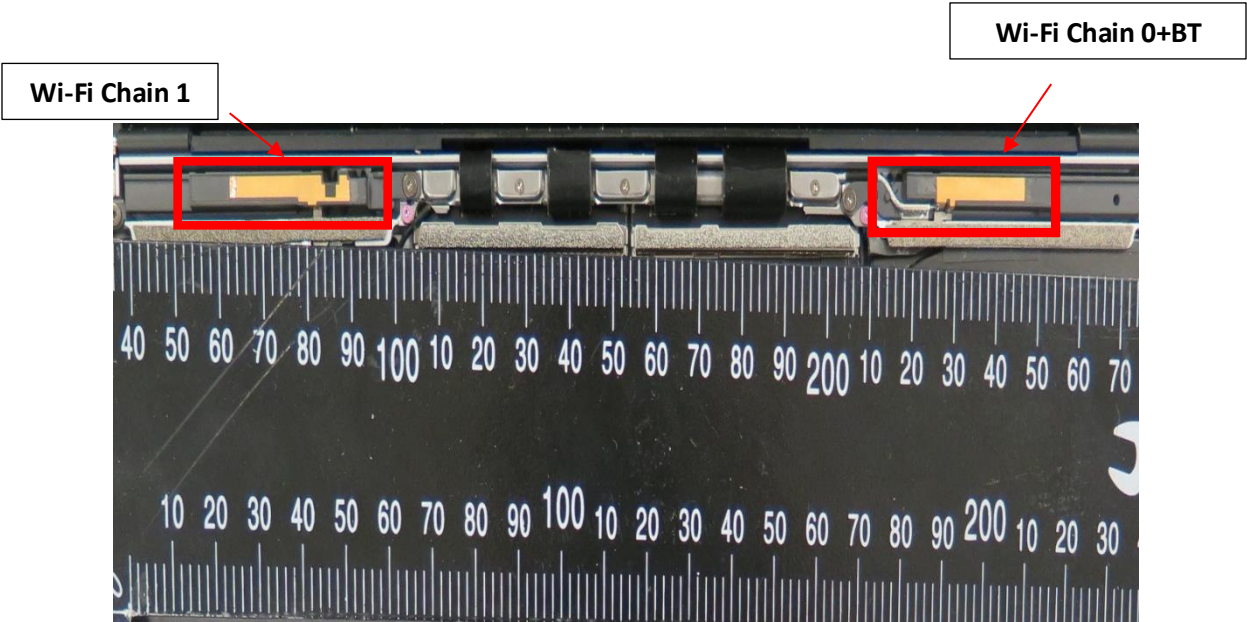
Figure 8 Close Up Antenna View
