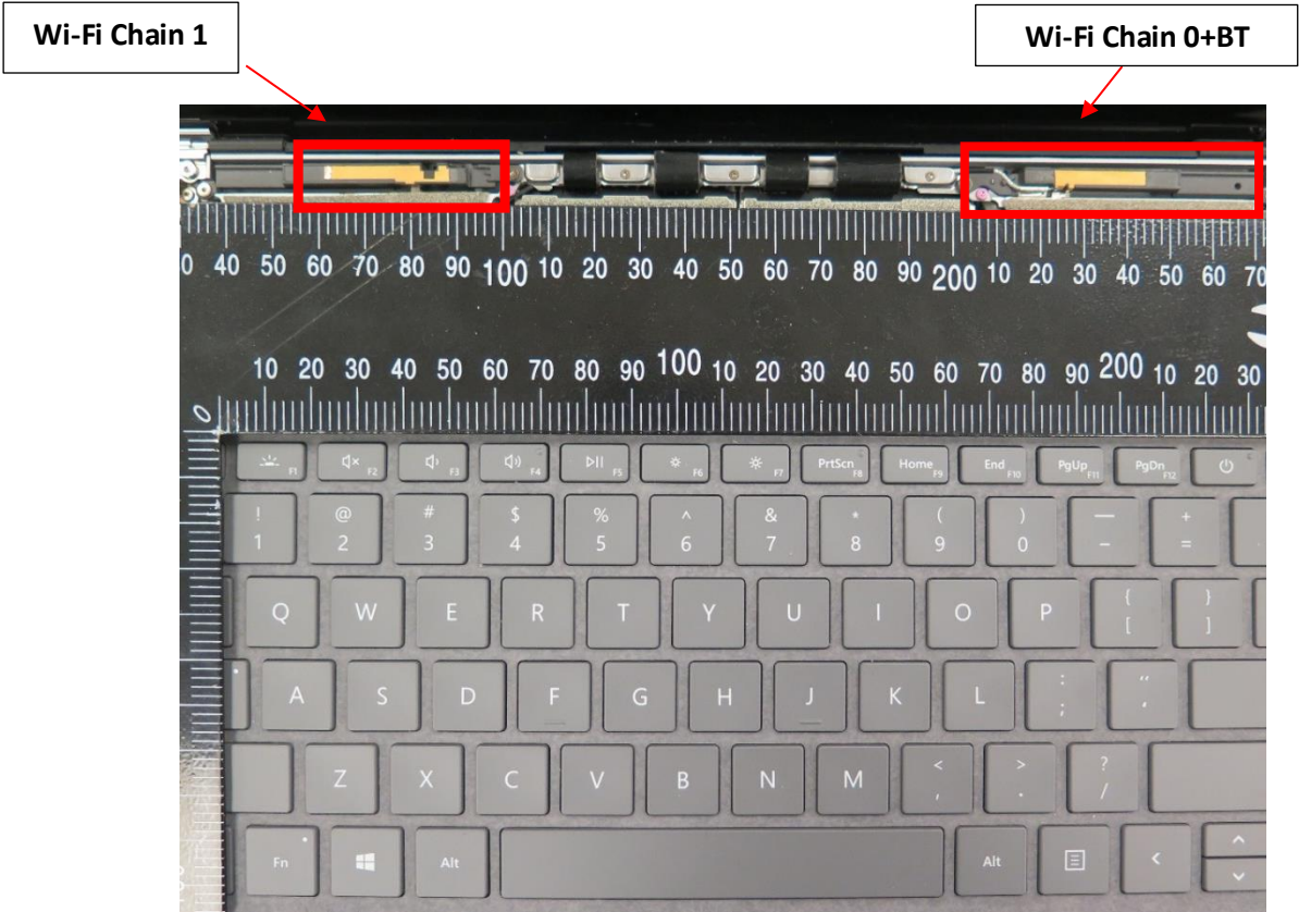
Figure 7 Wi-Fi/BT Chain 0 & 1 Antenna View
