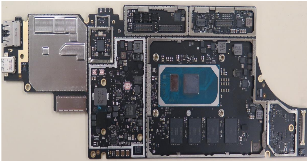
Figure 3 Close up Main Logic Board section
