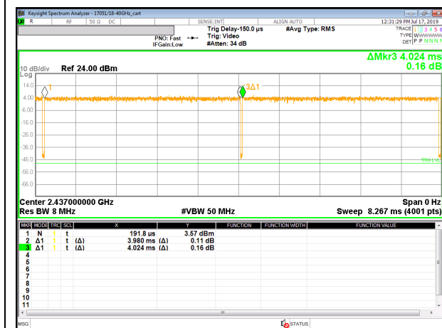
DUTY CYCLE 802.11n HT20 SDM MODE
