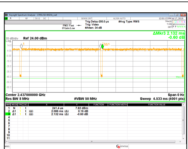
DUTY CYCLE 802.11g CDD MODE
