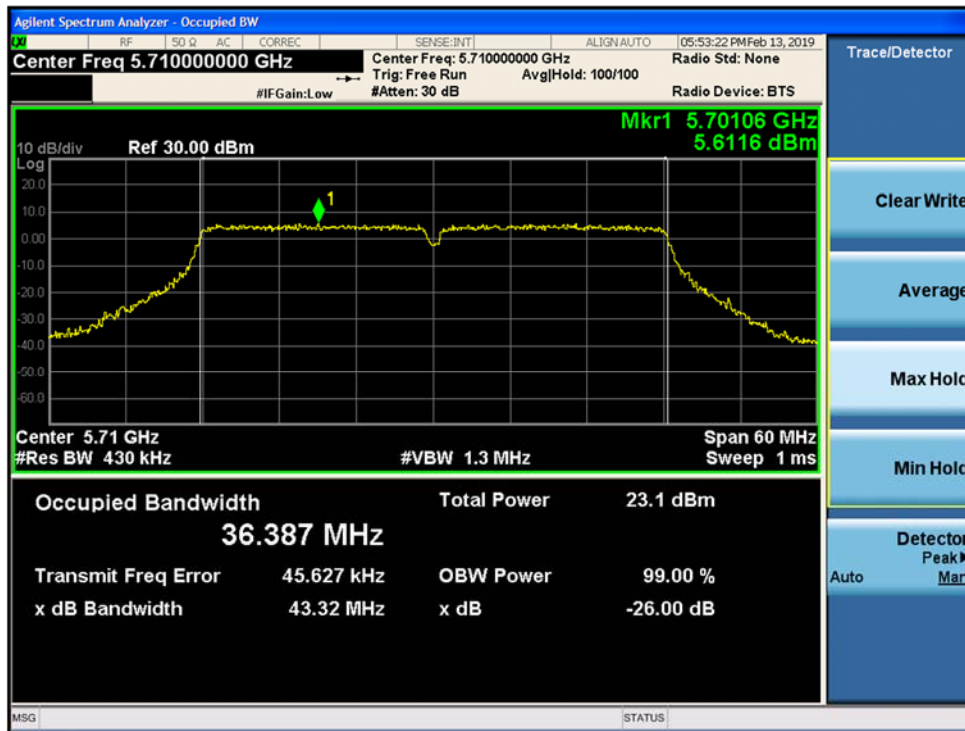
Figure 9-89. 26dB Emission Bandwidth and 99% OBW SISO Chain B 802.11ac VHT 40 (CH. 142)
