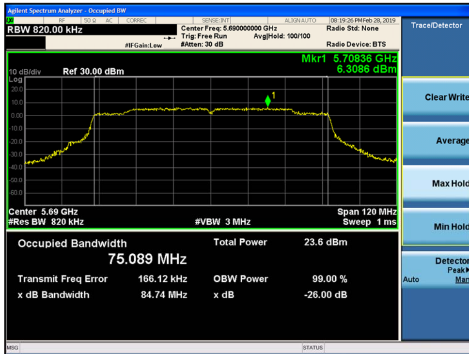
Figure 9-114. 26-dB Emission Bandwidth and 99% OBW MIMO Chain A 802.11ac VHT80 (Ch. 138)
