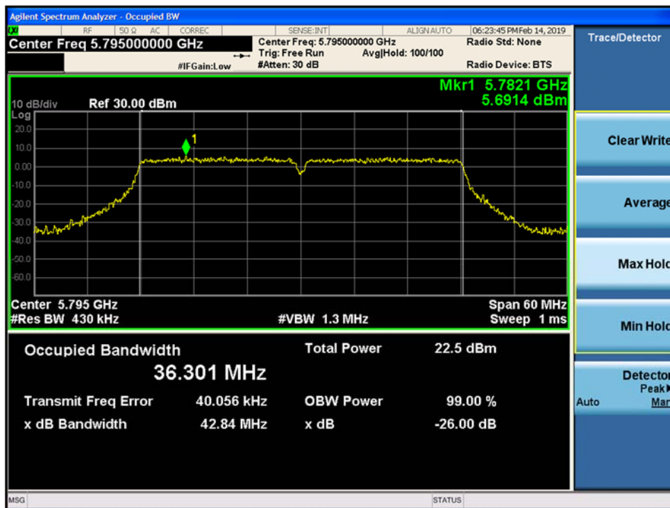
Figure 9-85. 26dB Emission Bandwidth and 99% OBW SISO Chain A 802.11ac VHT 40 (CH. 159)
