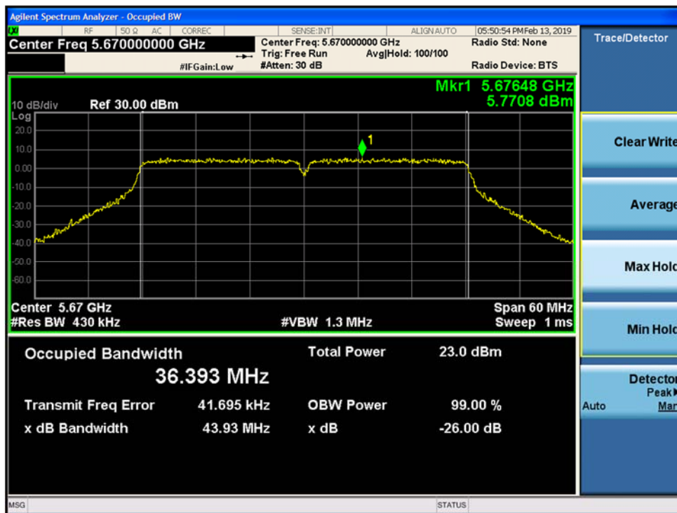
Figure 9-88. 26dB Emission Bandwidth and 99% OBW SISO Chain B 802.11ac VHT 40 (CH. 134)
