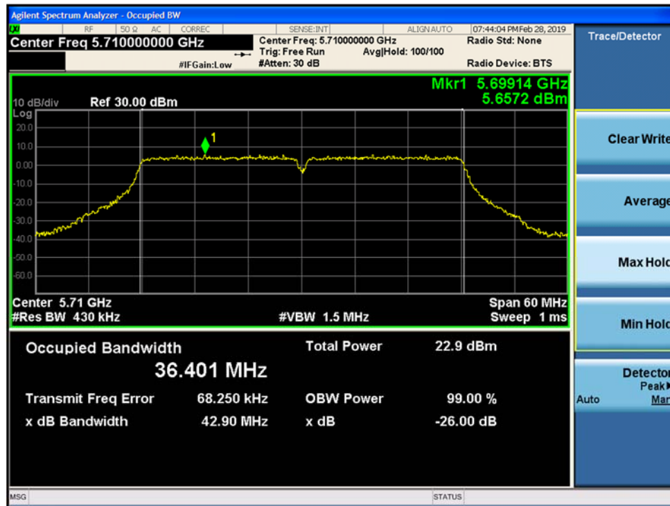
Figure 9-94. 26dB Emission Bandwidth and 99% OBW MIMO Chain A 802.11ac VHT 40 (CH.142)
