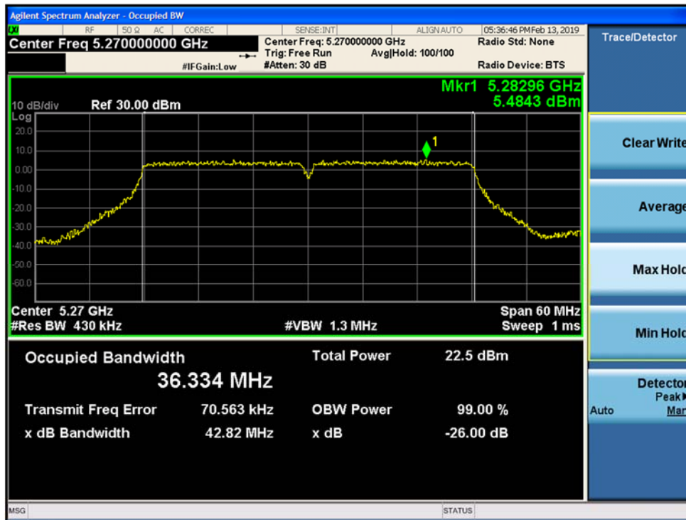
Figure 9-87. 26dB Emission Bandwidth and 99% OBW SISO Chain B 802.11ac VHT 40 (CH. 54)
