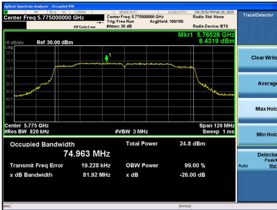
Figure 9-119. 26-dB Emission Bandwidth and 99% OBW MIMO Chain B 802.11ac VHT80 (Ch. 155)
