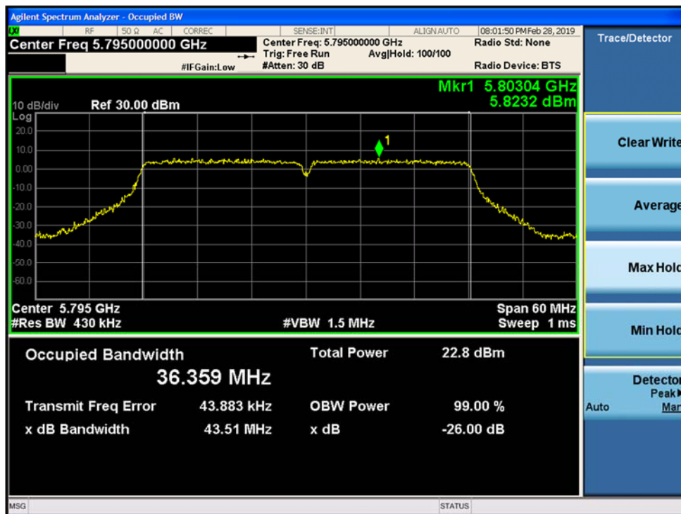
Figure 9-95. 26dB Emission Bandwidth and 99% OBW MIMO Chain A 802.11ac VHT 40 (CH.159)
