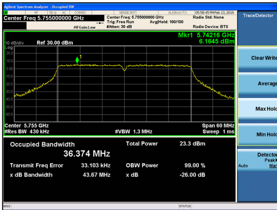
Figure 9-90. 26dB Emission Bandwidth and 99% OBW SISO Chain B 802.11ac VHT 40 (CH.151)
