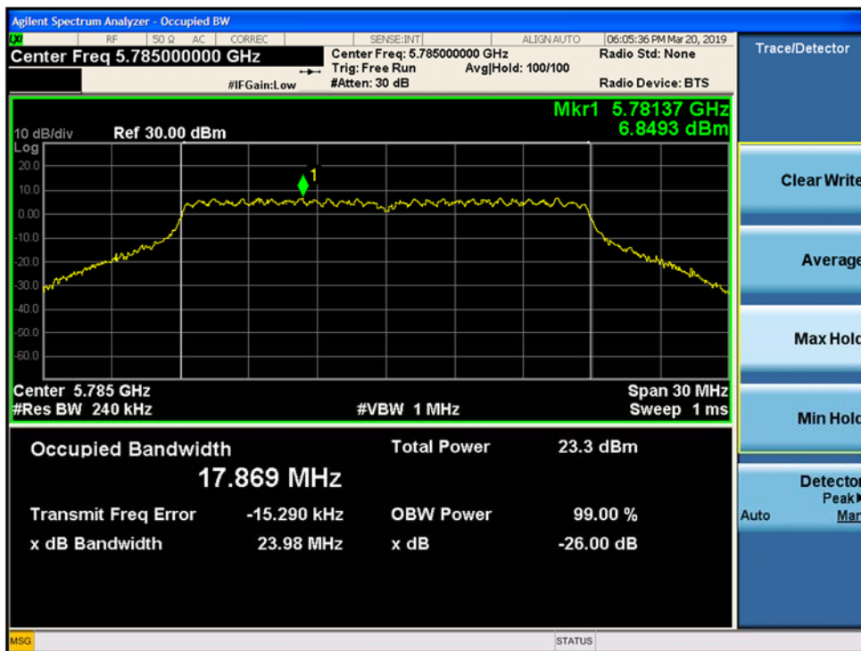
Figure 9-80. 26dB Emission Bandwidth and 99% OBW MIMO Chain B 802.11ac VHT 20 (CH. 157)
