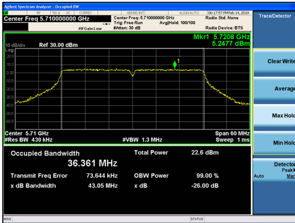
Figure 9-84. 26dB Emission Bandwidth and 99% OBW SISO Chain A 802.11ac VHT 40 (CH. 142)
