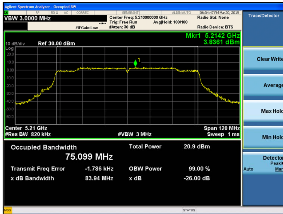
Figure 9-116. 26-dB Emission Bandwidth and 99% OBW MIMO Chain B 802.11ac VHT80 (Ch. 42)
