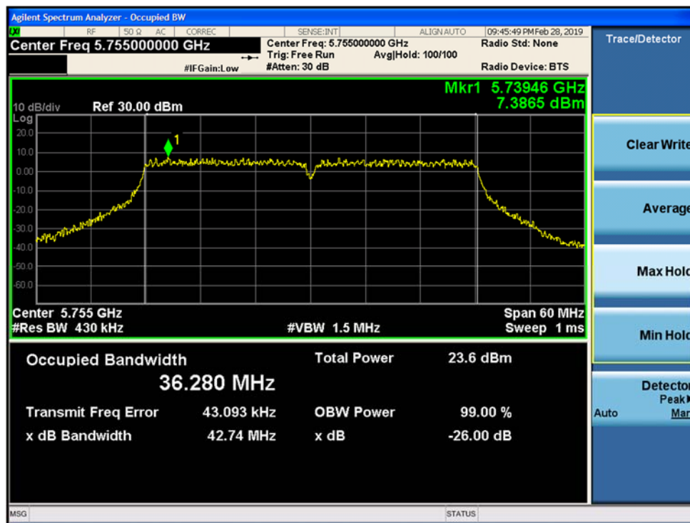
Figure 9-100. 26dB Emission Bandwidth and 99% OBW MIMO Chain B 802.11ac VHT 40 (CH.151)
