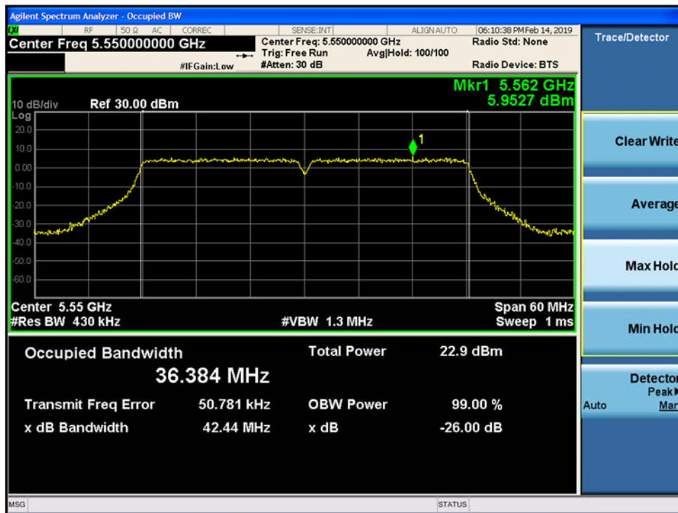
Figure 9-83. 26dB Emission Bandwidth and 99% OBW SISO Chain A 802.11ac VHT 40 (CH. 110)
