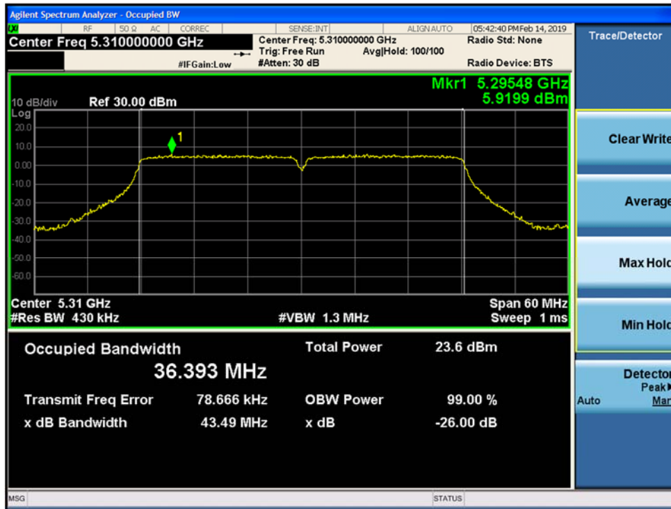
Figure 9-82. 26dB Emission Bandwidth and 99% OBW SISO Chain A 802.11ac VHT 40 (CH. 62)
