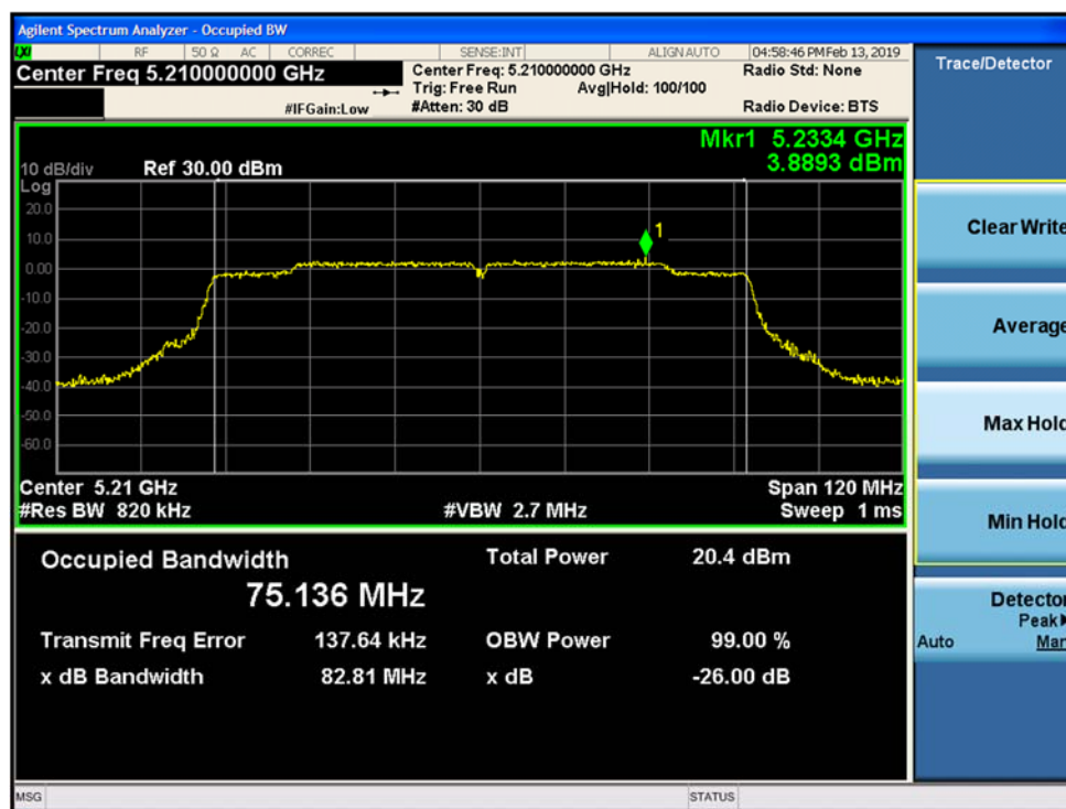
Figure 9-106. 26-dB Emission Bandwidth and 99% OBW SISO Chain B 802.11ac VHT80 (Ch. 42)
