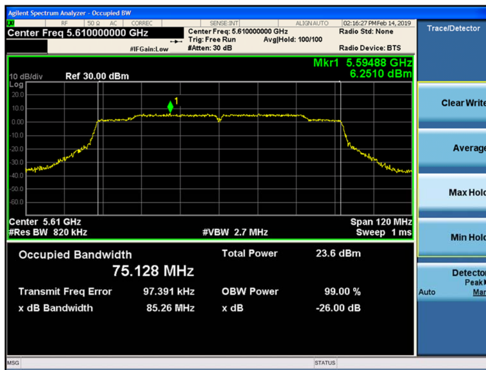
Figure 9-103. 26-dB Emission Bandwidth and 99% OBW SISO Chain A 802.11ac VHT80 (Ch. 122)
