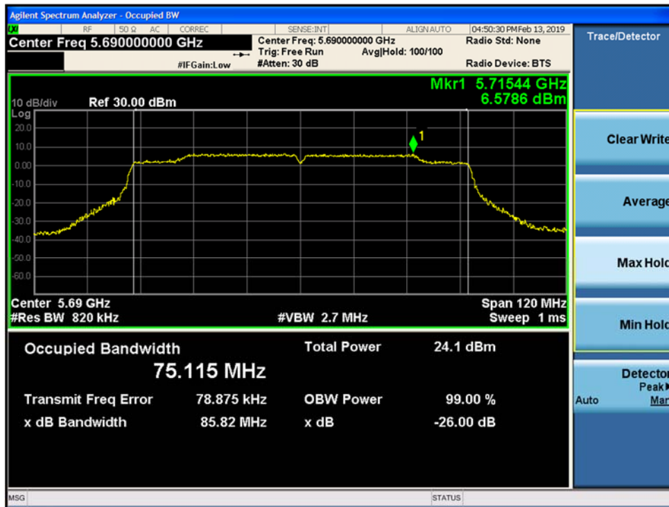
Figure 9-109. 26-dB Emission Bandwidth and 99% OBW SISO Chain B 802.11ac VHT80 (Ch. 138)
