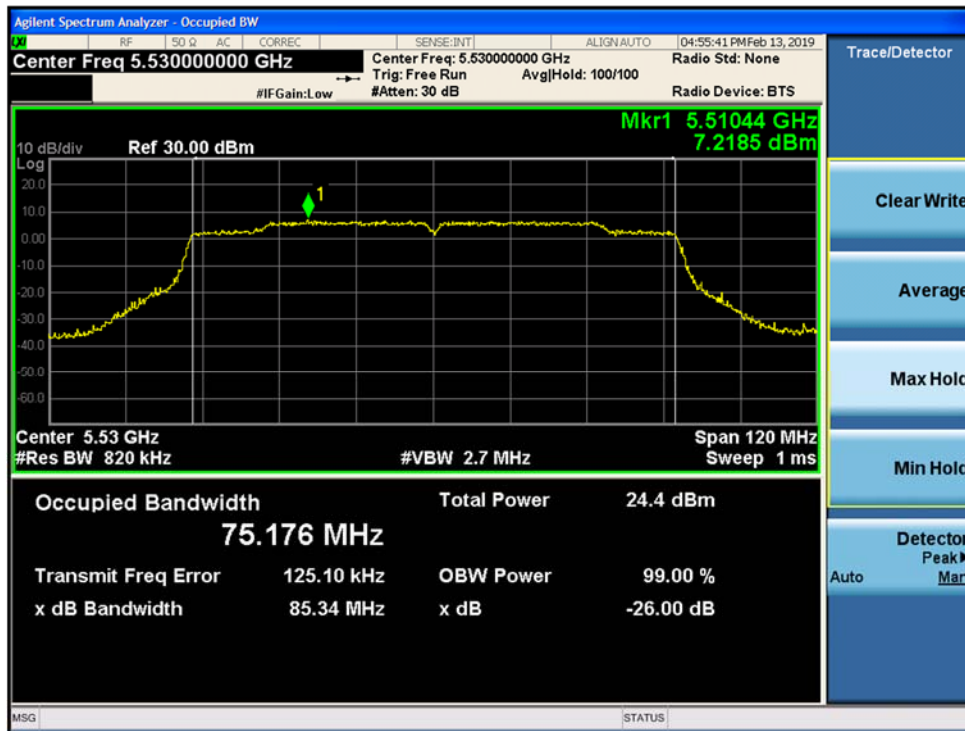
Figure 9-107. 26-dB Emission Bandwidth and 99% OBW SISO Chain B 802.11ac VHT80 (Ch. 106)
