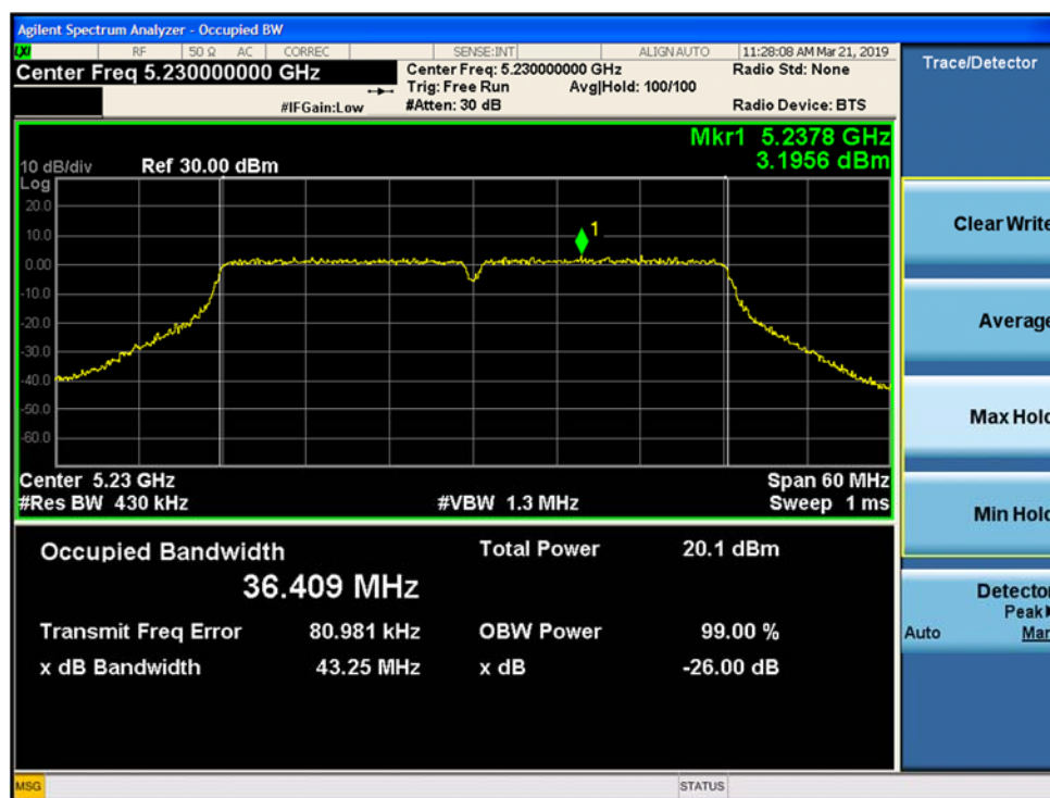
Figure 9-91. 26dB Emission Bandwidth and 99% OBW MIMO Chain A 802.11ac VHT 40 (CH.46)
