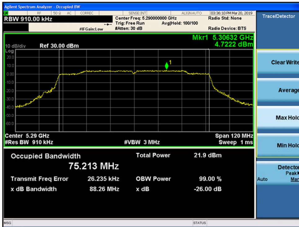
Figure 9-112. 26-dB Emission Bandwidth and 99% OBW MIMO Chain A 802.11ac VHT80 (Ch. 58)
