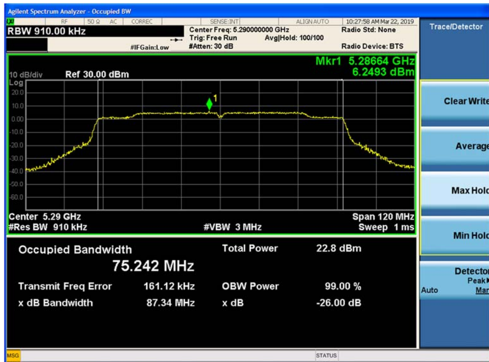
Figure 9-102. 26-dB Emission Bandwidth and 99% OBW SISO Chain A 802.11ac VHT80 (Ch. 58)
