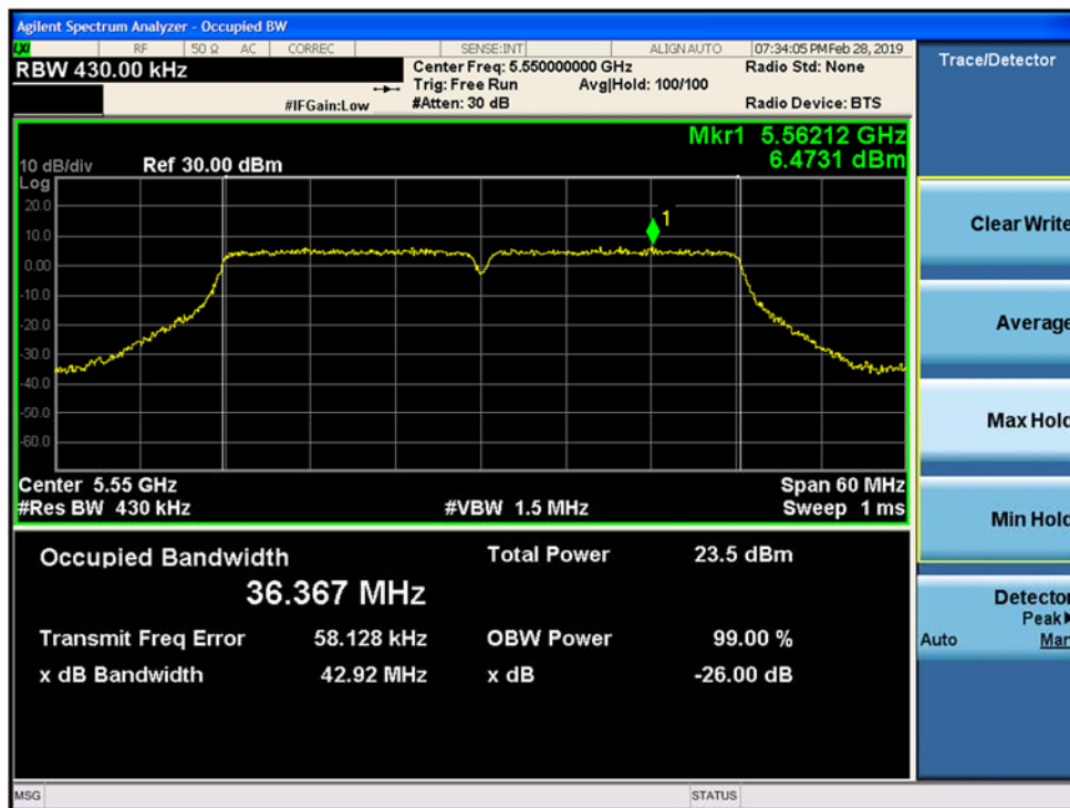
Figure 9-93. 26dB Emission Bandwidth and 99% OBW MIMO Chain A 802.11ac VHT 40 (CH.110)
