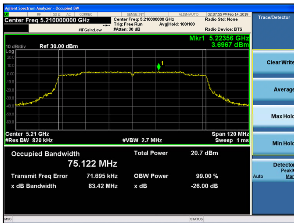
Figure 9-101. 26-dB Emission Bandwidth and 99% OBW SISO Chain A 802.11ac VHT80 (Ch. 42)
