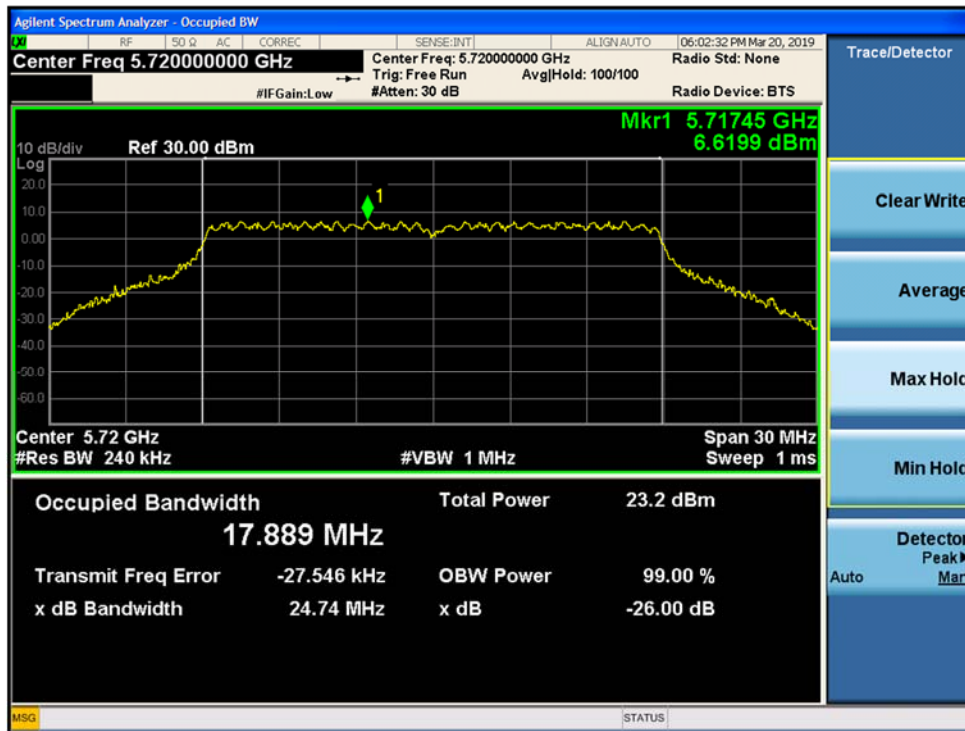
Figure 9-79. 26dB Emission Bandwidth and 99% OBW MIMO Chain B 802.11ac VHT 20 (CH. 144)
