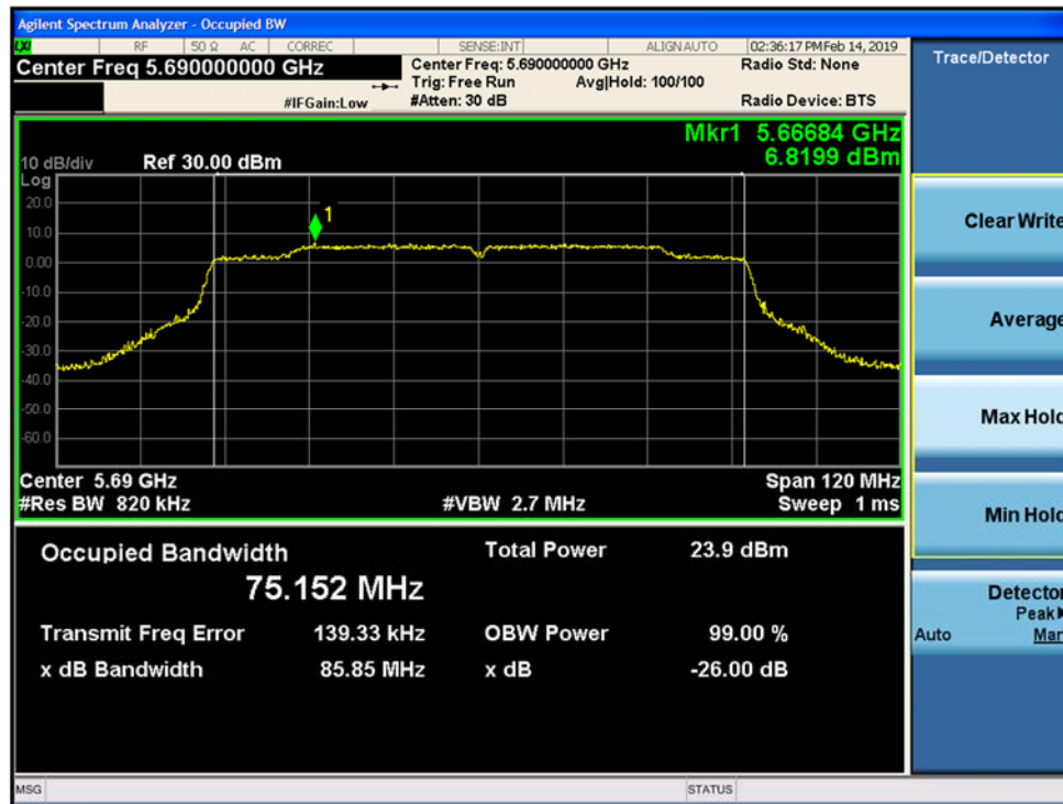
Figure 9-104. 26-dB Emission Bandwidth and 99% OBW SISO Chain A 802.11ac VHT80 (Ch. 138)
