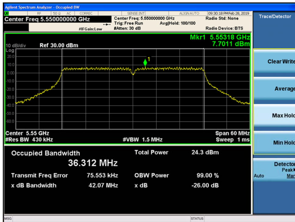
Figure 9-98. 26dB Emission Bandwidth and 99% OBW MIMO Chain B 802.11ac VHT 40 (CH.110)
