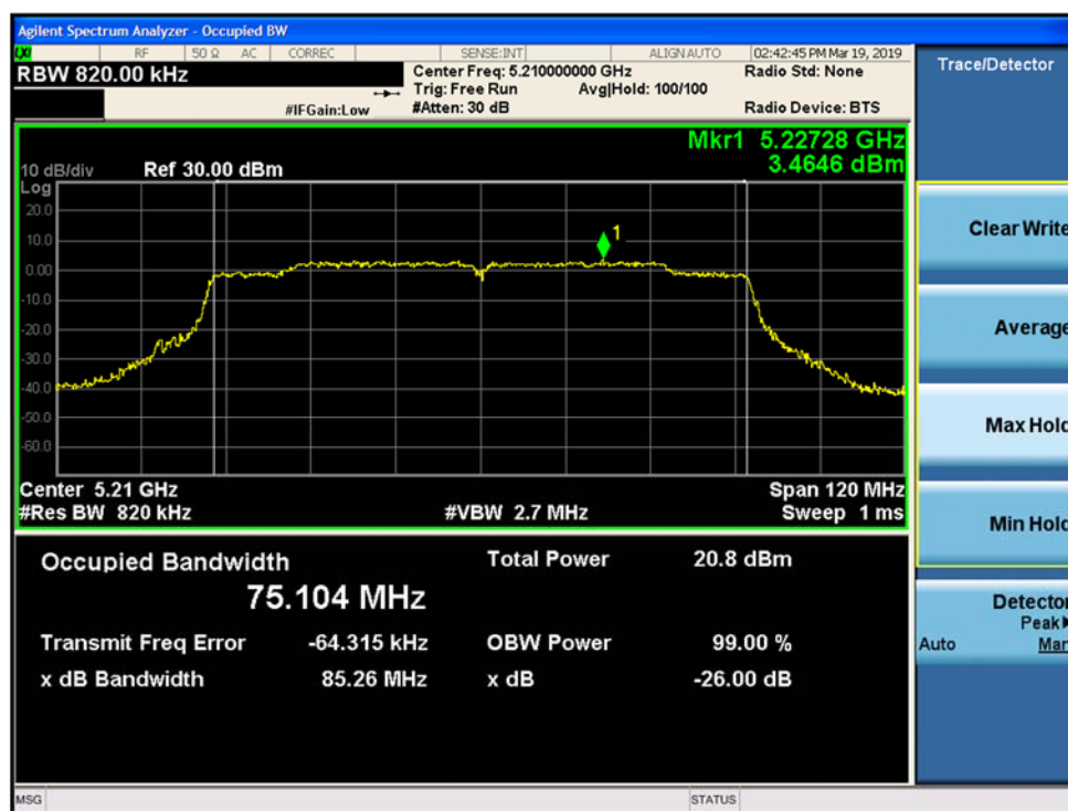
Figure 9-111. 26-dB Emission Bandwidth and 99% OBW MIMO Chain A 802.11ac VHT80 (Ch. 42)
