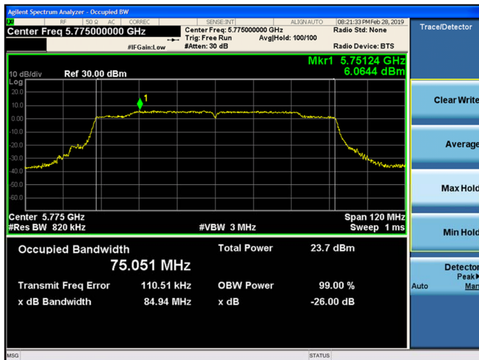
Figure 9-115. 26-dB Emission Bandwidth and 99% OBW MIMO Chain A 802.11ac VHT80 (Ch. 155)
