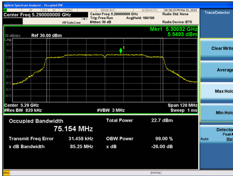
Figure 9-117. 26-dB Emission Bandwidth and 99% OBW MIMO Chain B 802.11ac VHT80 (Ch. 58)
