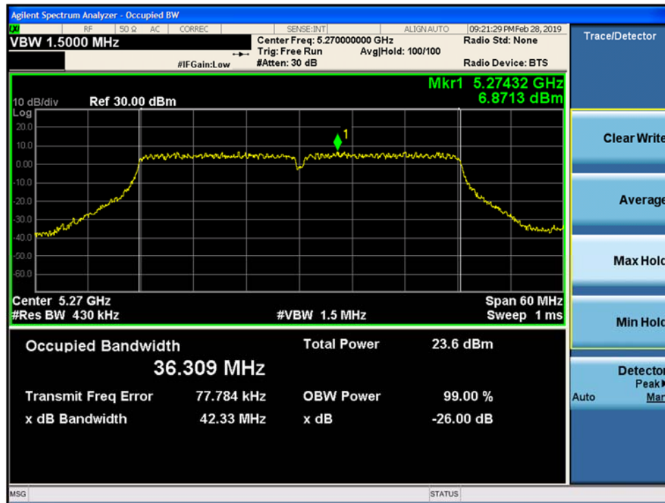
Figure 9-97. 26dB Emission Bandwidth and 99% OBW MIMO Chain B 802.11ac VHT 40 (CH.54)
