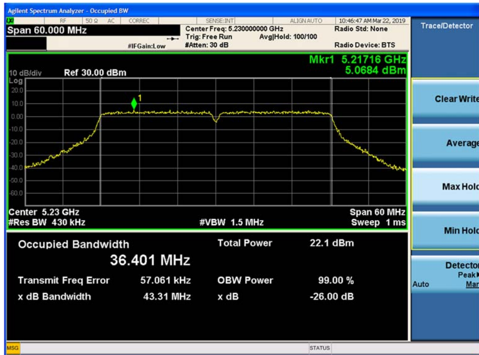
Figure 9-81. 26dB Emission Bandwidth and 99% OBW SISO Chain A 802.11ac VHT 40 (CH. 46)
