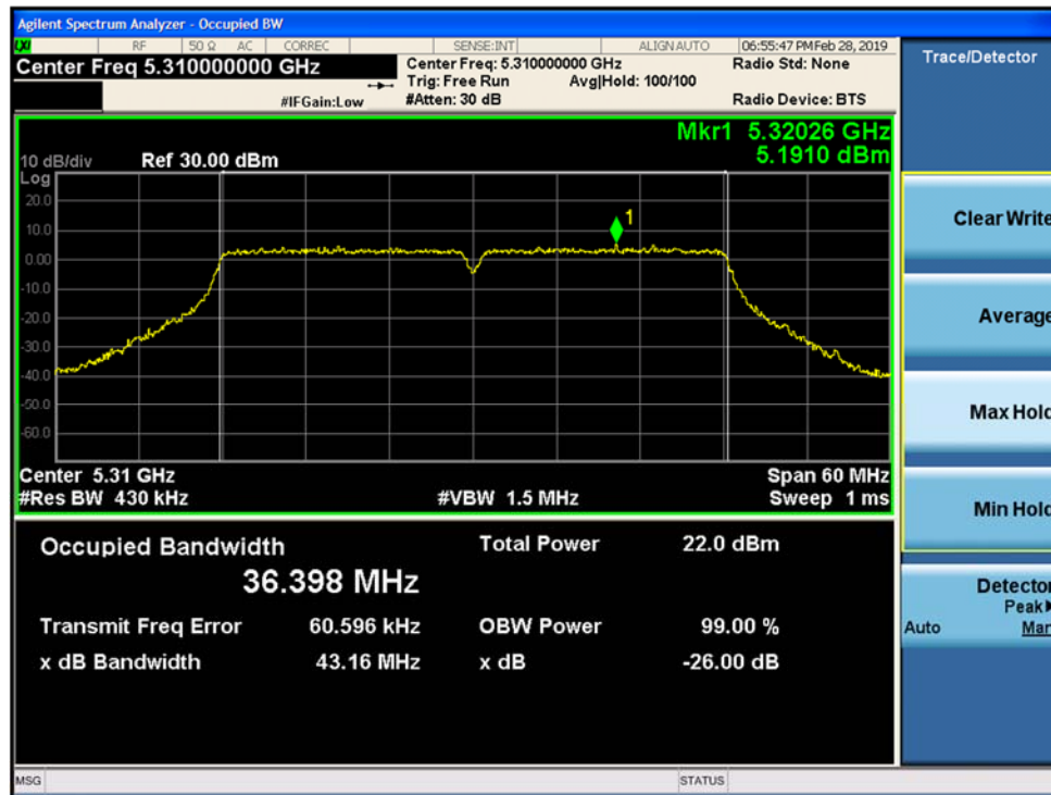
Figure 9-92. 26dB Emission Bandwidth and 99% OBW MIMO Chain A 802.11ac VHT 40 (CH.62)
