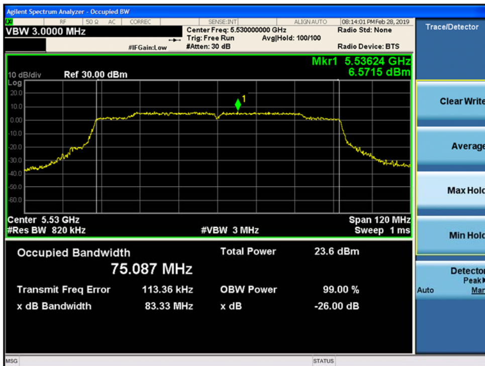
Figure 9-113. 26-dB Emission Bandwidth and 99% OBW MIMO Chain A 802.11ac VHT80 (Ch. 106)
