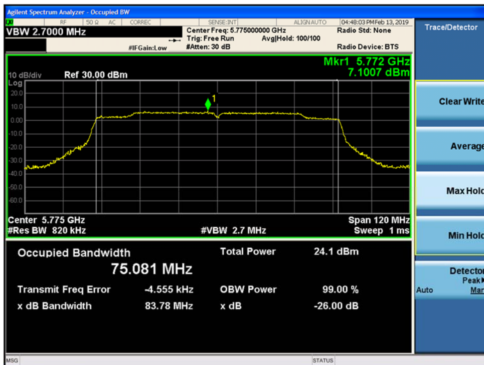
Figure 9-110. 26-dB Emission Bandwidth and 99% OBW SISO Chain B 802.11ac VHT80 (Ch. 155)
