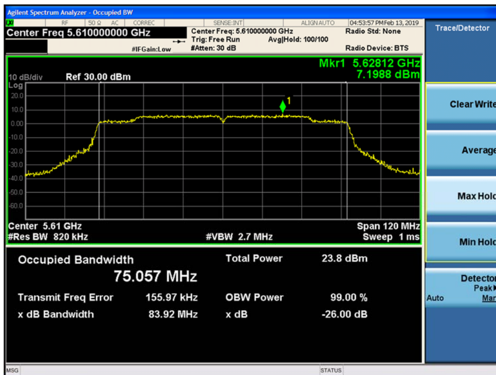
Figure 9-108. 26-dB Emission Bandwidth and 99% OBW SISO Chain B 802.11ac VHT80 (Ch. 122)
