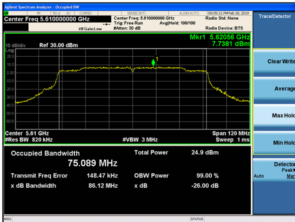
Figure 9-118. 26-dB Emission Bandwidth and 99% OBW MIMO Chain B 802.11ac VHT80 (Ch. 122)
