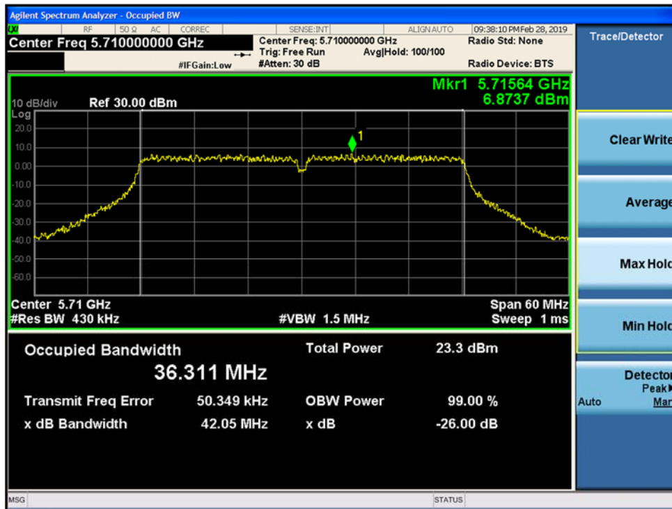
Figure 9-99. 26dB Emission Bandwidth and 99% OBW MIMO Chain B 802.11ac VHT 40 (CH.142)
