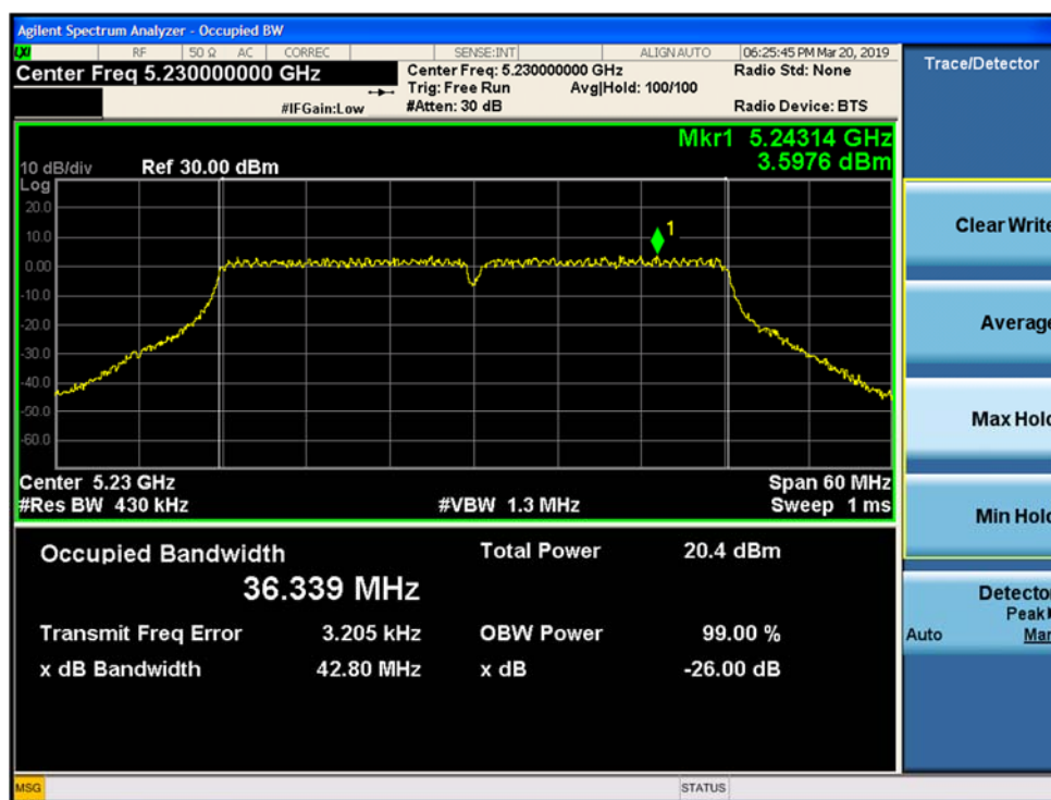
Figure 9-96. 26dB Emission Bandwidth and 99% OBW MIMO Chain B 802.11ac VHT 40 (CH.46)
