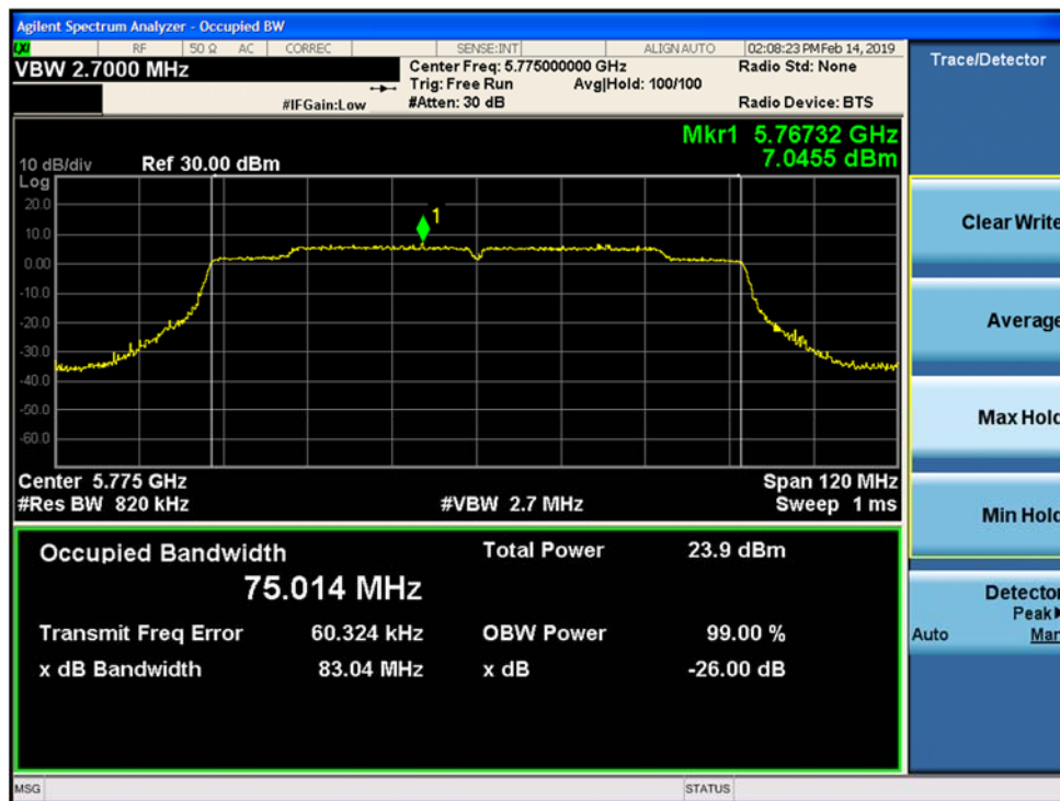
Figure 9-105. 26-dB Emission Bandwidth and 99% OBW SISO Chain A 802.11ac VHT80 (Ch. 155)
