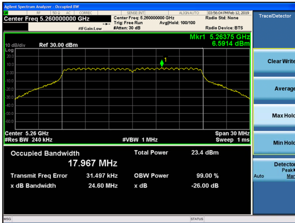
Figure 9-67. 26dB Emission Bandwidth and 99% OBW SISO Chain B 802.11ac VHT 20 (CH. 52)
