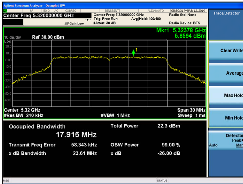
Figure 9-62. 26dB Emission Bandwidth and 99% OBW SISO Chain A 802.11ac VHT 20 (CH. 64)
