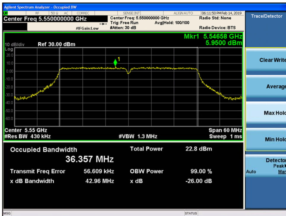
Figure 9-17. 26-dB Emission Bandwidth and 99% OBW SISO Chain A 802.11n HT40 (Ch. 110)
