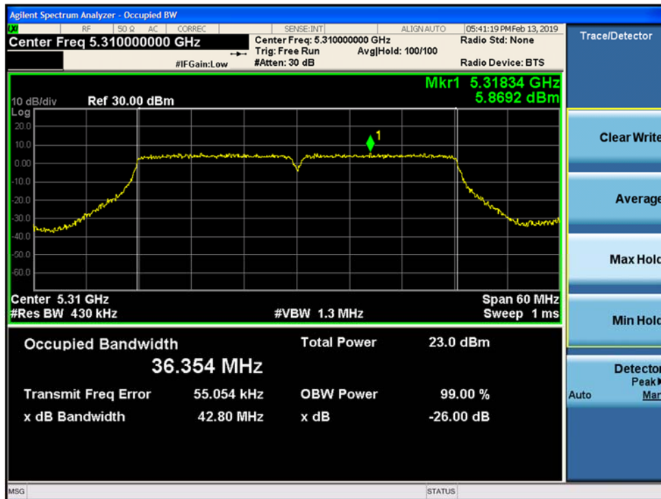
Figure 9-47. 26-dB Emission Bandwidth and 99% OBW SISO Chain B 802.11n HT40 (Ch. 62)
