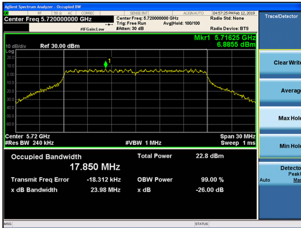
Figure 9-39. 26-dB Emission Bandwidth and 99% OBW MIMO Chain B 802.11n HT20 (Ch. 144)
