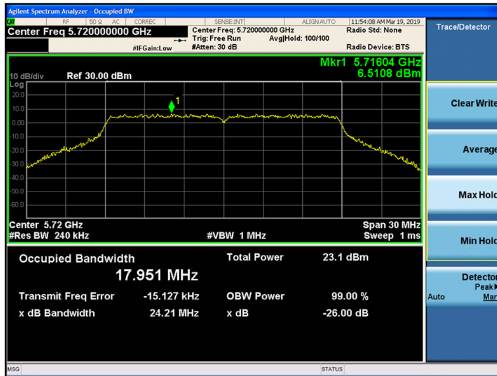
Figure 9-74. 26dB Emission Bandwidth and 99% OBW MIMO Chain A 802.11ac VHT 20 (CH. 144)
