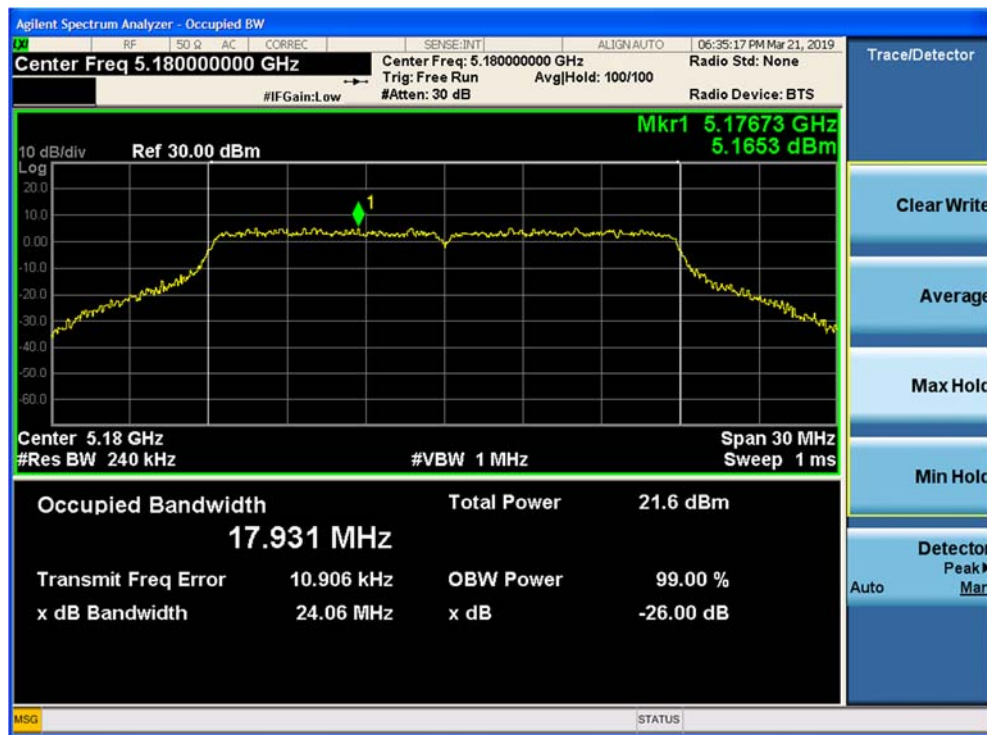
Figure 9-66. 26dB Emission Bandwidth and 99% OBW SISO Chain B 802.11ac VHT 20 (CH. 36)
