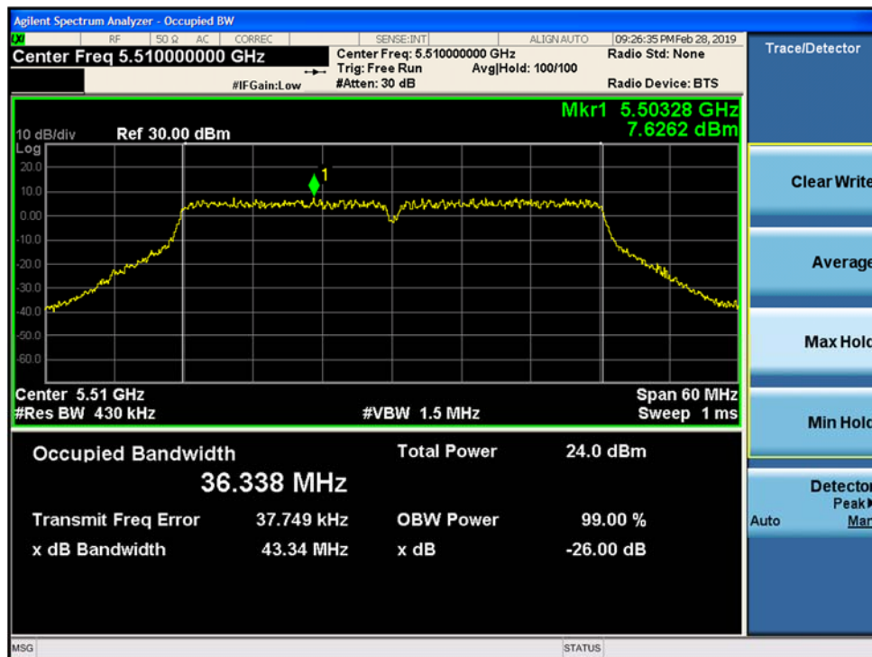
Figure 9-58. 26-dB Emission Bandwidth and 99% OBW MIMO Chain B 802.11n HT40 (Ch. 102)
