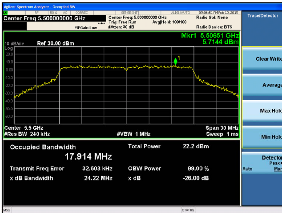
Figure 9-63. 26dB Emission Bandwidth and 99% OBW SISO Chain A 802.11ac VHT 20 (CH. 100)
