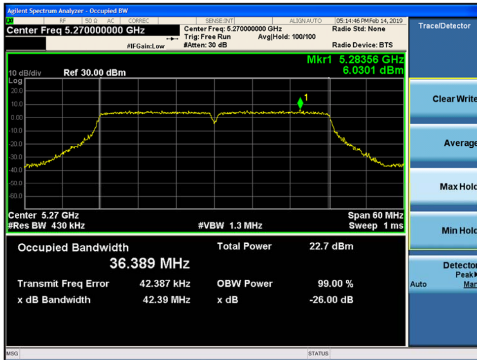
Figure 9-16. 26-dB Emission Bandwidth and 99% OBW SISO Chain A 802.11n HT40 (Ch. 54)
