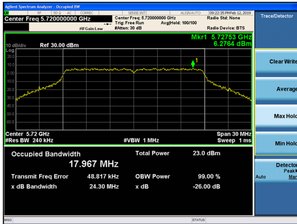
Figure 9-64. 26dB Emission Bandwidth and 99% OBW SISO Chain A 802.11ac VHT 20 (CH. 144)
