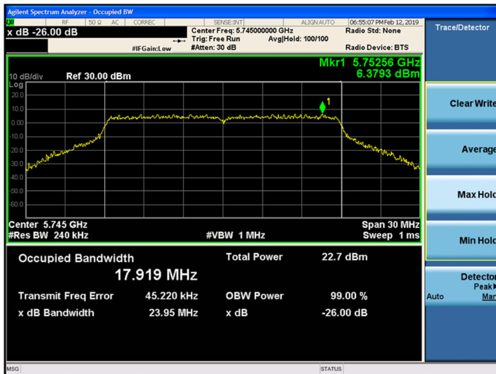
Figure 9-65. 26dB Emission Bandwidth and 99% OBW SISO Chain A 802.11ac VHT 20 (CH. 149)
