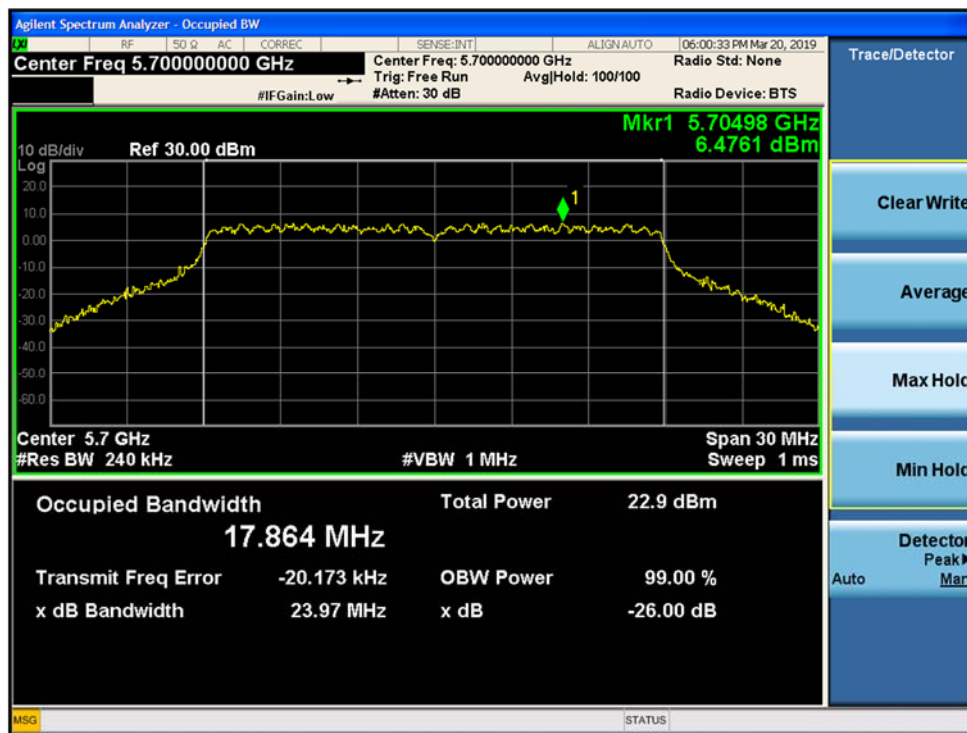
Figure 9-78. 26dB Emission Bandwidth and 99% OBW MIMO Chain B 802.11ac VHT 20 (CH. 140)
