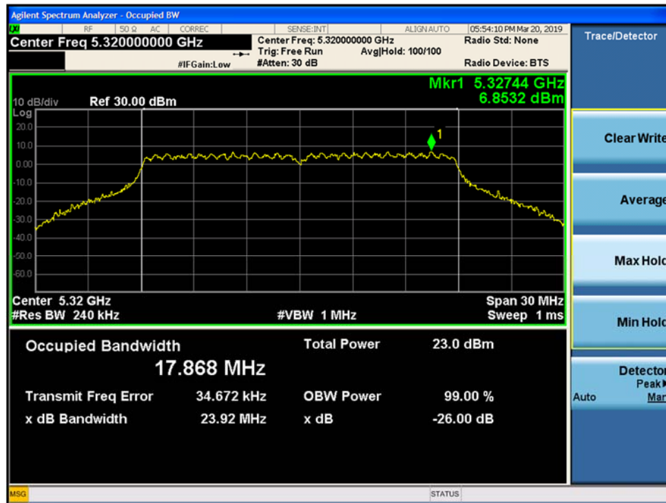
Figure 9-77. 26dB Emission Bandwidth and 99% OBW MIMO Chain B 802.11ac VHT 20 (CH. 64)
