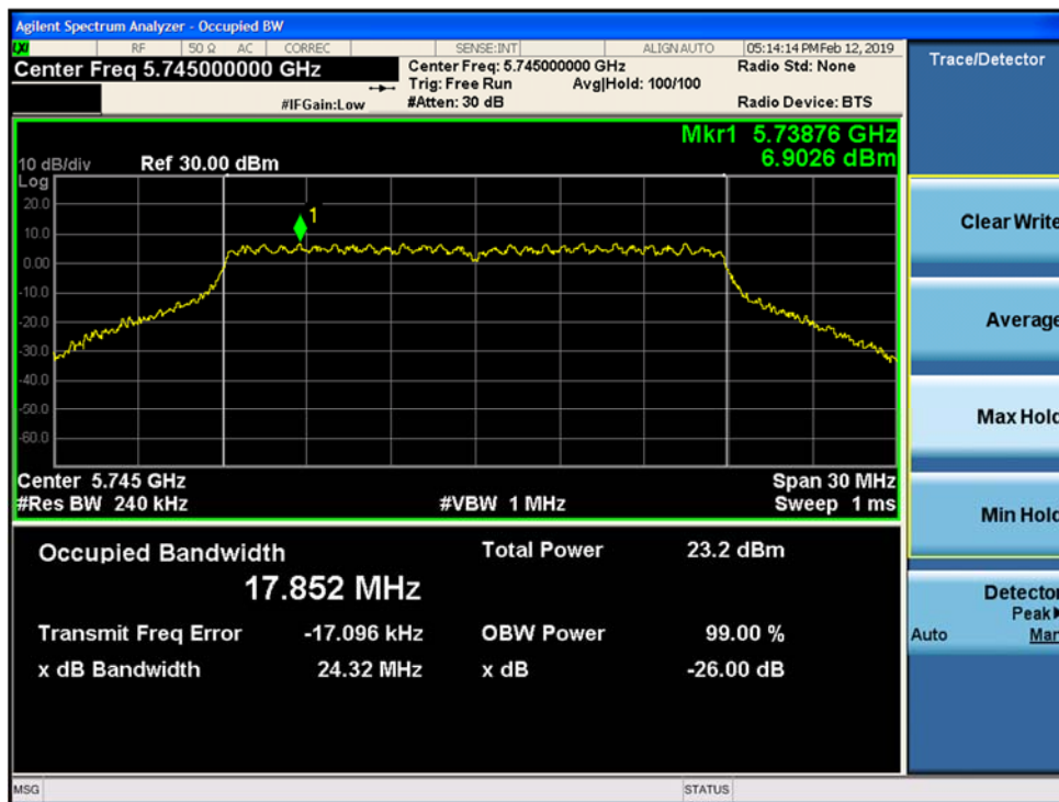
Figure 9-70. 26dB Emission Bandwidth and 99% OBW SISO Chain B 802.11ac VHT 20 (CH. 149)
