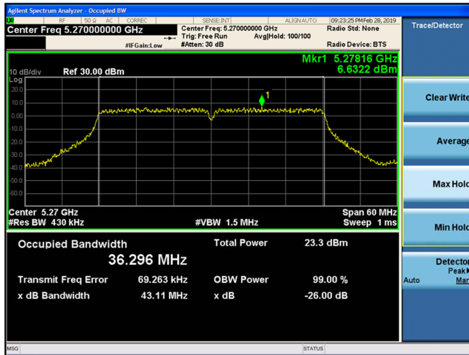
Figure 9-57. 26-dB Emission Bandwidth and 99% OBW MIMO Chain B 802.11n HT40 (Ch. 54)
