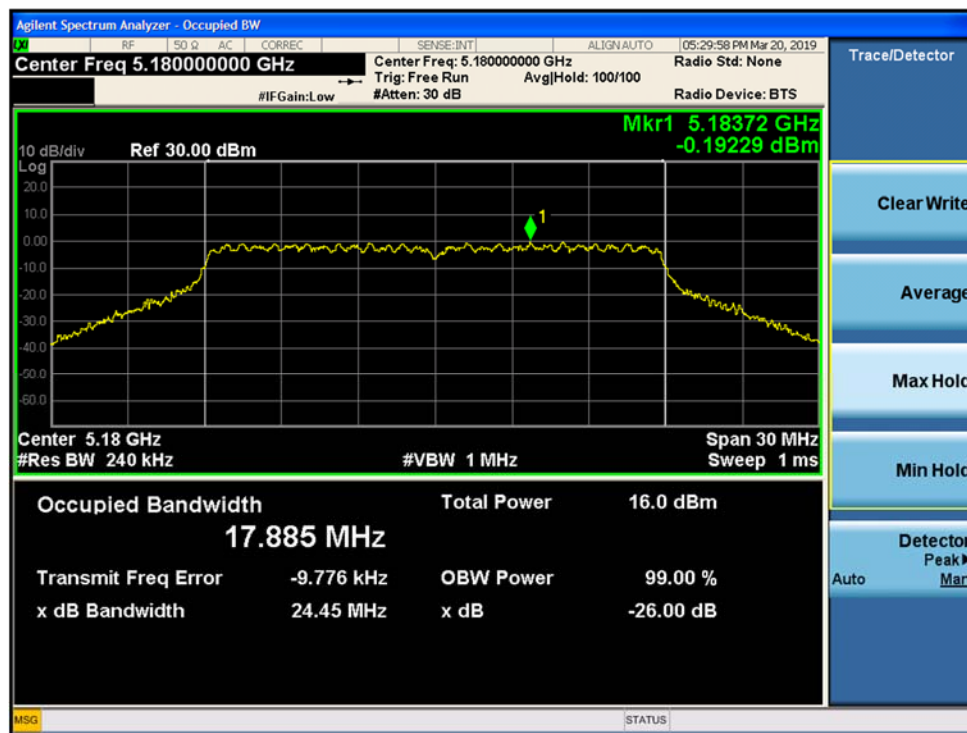
Figure 9-76. 26dB Emission Bandwidth and 99% OBW MIMO Chain B 802.11ac VHT 20 (CH. 36)
