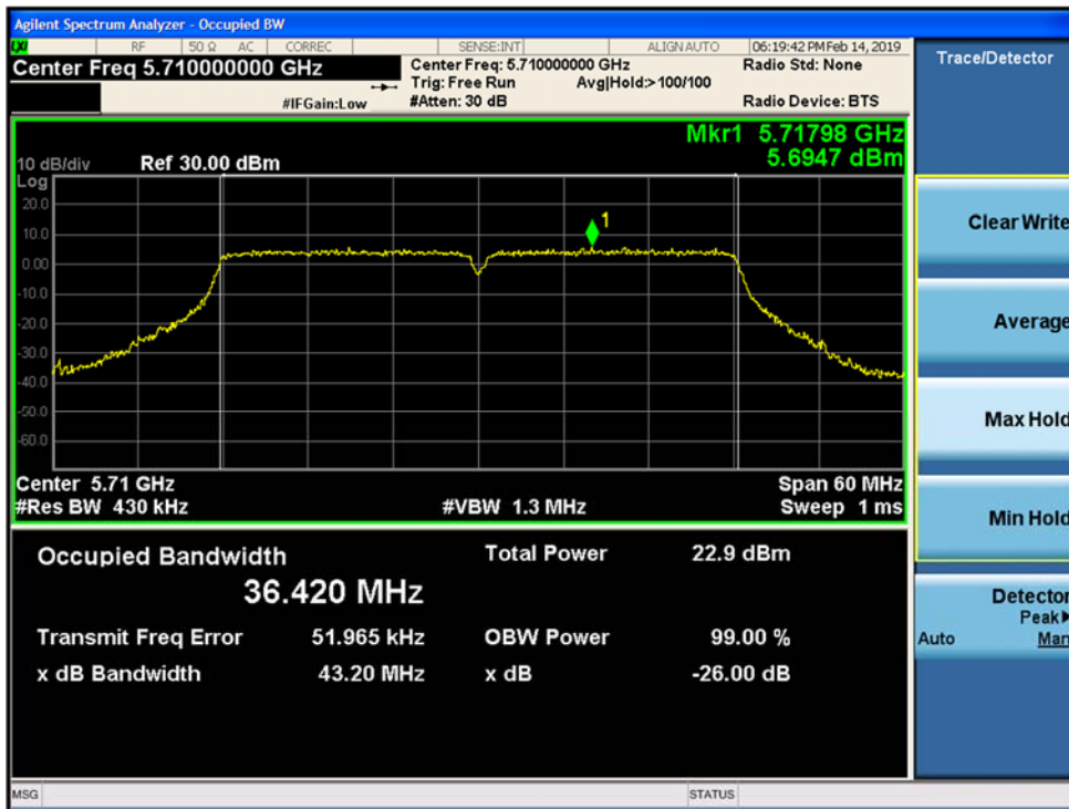
Figure 9-18. 26-dB Emission Bandwidth and 99% OBW SISO Chain A 802.11n HT40 (Ch. 142)
