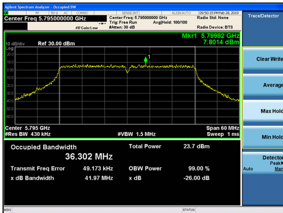
Figure 9-60. 26-dB Emission Bandwidth and 99% OBW MIMO Chain B 802.11n HT40 (Ch. 159)
