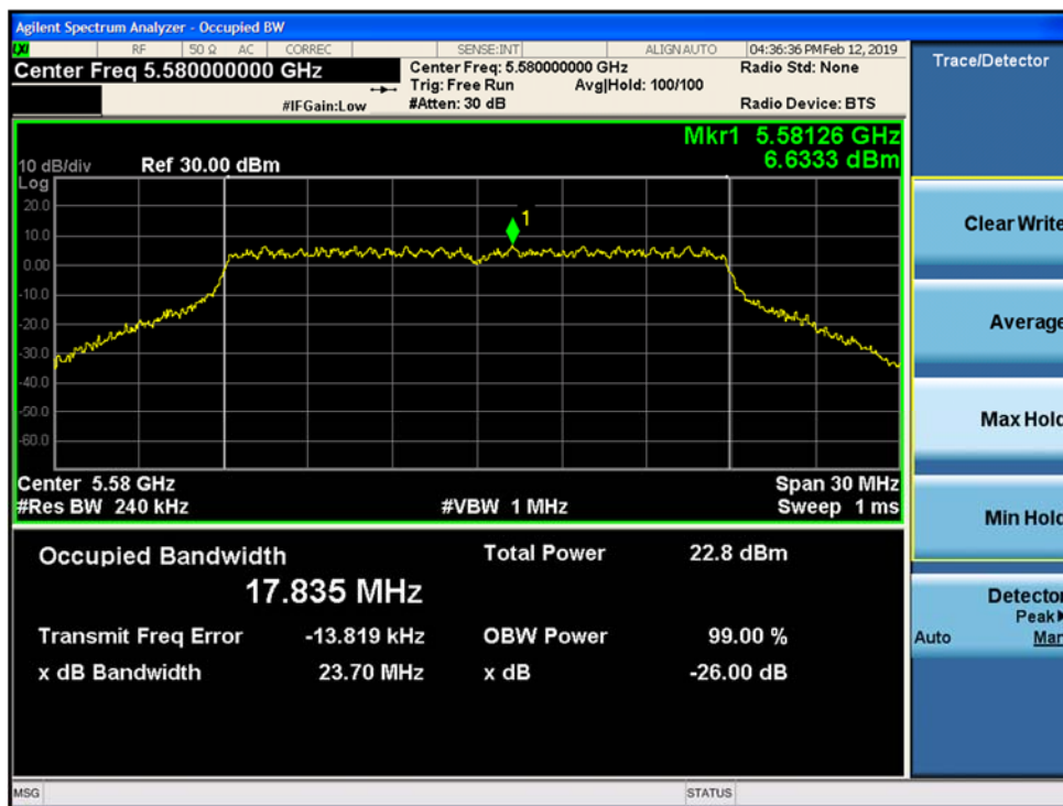
Figure 9-68. 26dB Emission Bandwidth and 99% OBW SISO Chain B 802.11ac VHT 20 (CH. 116)
