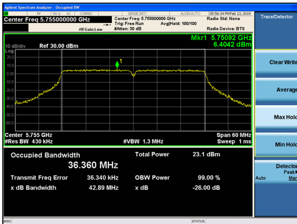
Figure 9-50. 26-dB Emission Bandwidth and 99% OBW SISO Chain B 802.11n HT40 (Ch. 151)
