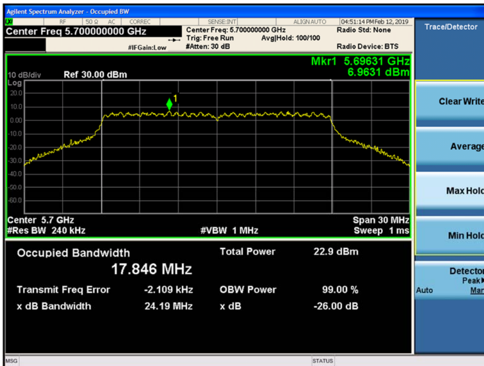
Figure 9-38. 26-dB Emission Bandwidth and 99% OBW MIMO Chain B 802.11n HT20 (Ch. 140)
