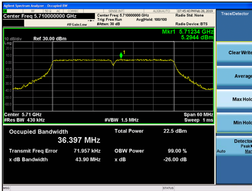
Figure 9-54. 26-dB Emission Bandwidth and 99% OBW MIMO Chain A 802.11n HT40 (Ch. 142)
