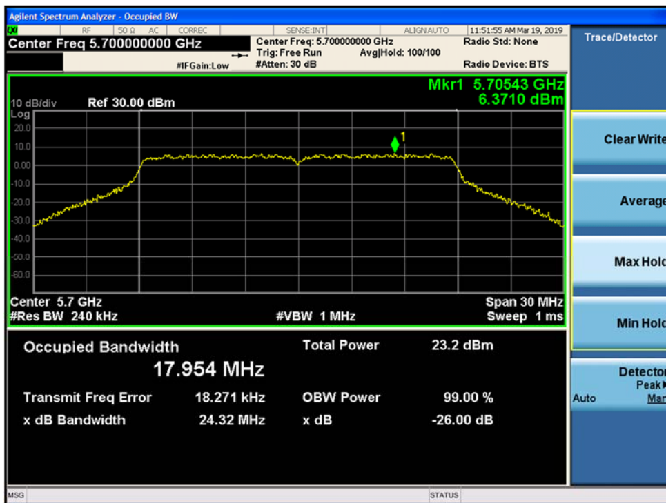
Figure 9-73. 26dB Emission Bandwidth and 99% OBW MIMO Chain A 802.11ac VHT 20 (CH. 140)
