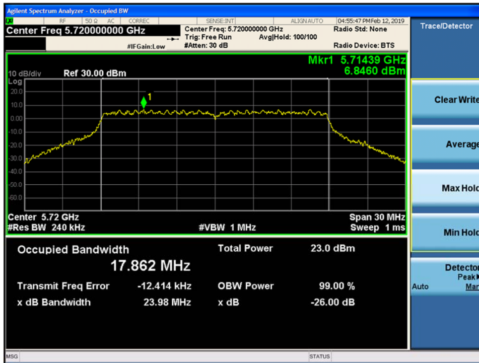
Figure 9-69 26dB Emission Bandwidth and 99% OBW SISO Chain B 802.11ac VHT 20 (CH. 144)
