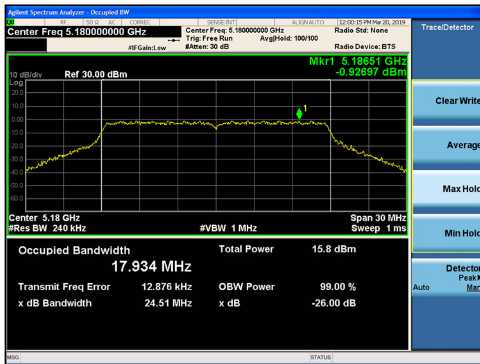
Figure 9-71. 26dB Emission Bandwidth and 99% OBW MIMO Chain A 802.11ac VHT 20 (CH. 36)
