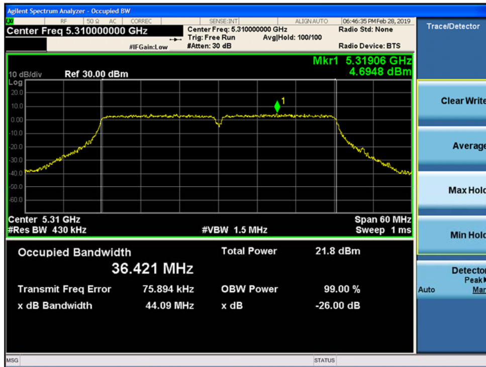
Figure 9-52. 26-dB Emission Bandwidth and 99% OBW MIMO Chain A 802.11n HT40 (Ch. 62)
