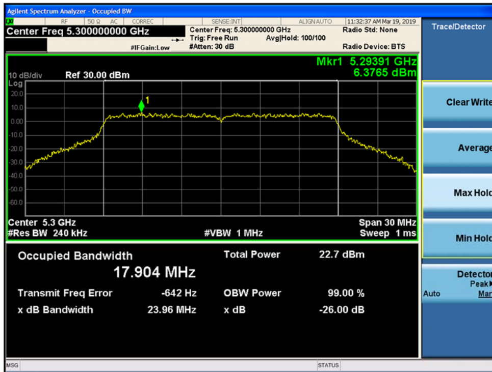
Figure 9-72. 26dB Emission Bandwidth and 99% OBW MIMO Chain A 802.11ac VHT 20 (CH. 60)
