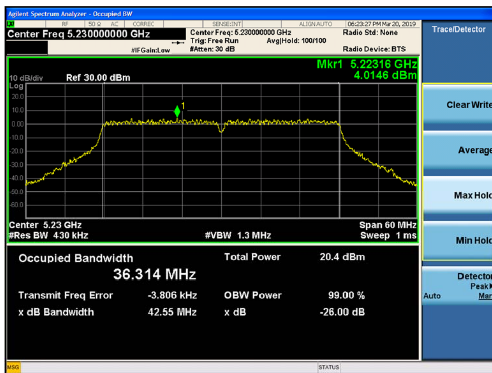
Figure 9-56. 26-dB Emission Bandwidth and 99% OBW MIMO Chain B 802.11n HT40 (Ch. 46)
