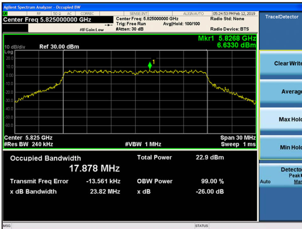
Figure 9-40. 26-dB Emission Bandwidth and 99% OBW MIMO Chain B 802.11n HT20 (Ch. 165)
