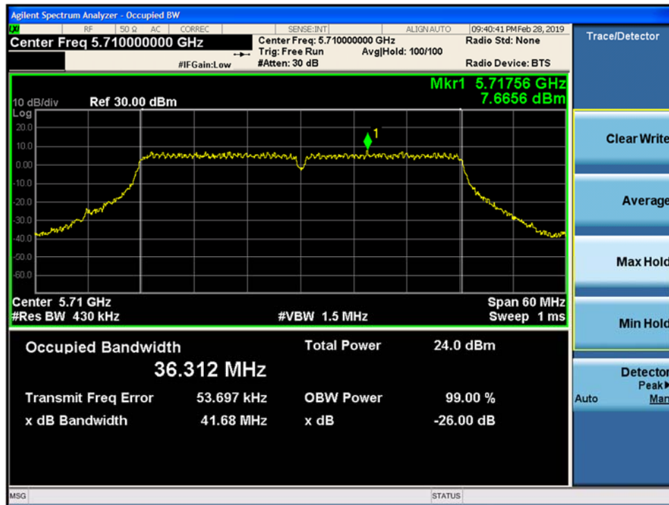
Figure 9-59. 26-dB Emission Bandwidth and 99% OBW MIMO Chain B 802.11n HT40 (Ch. 142)
