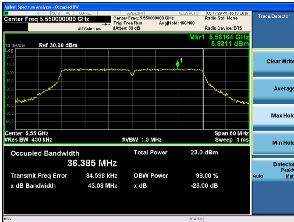
Figure 9-48. 26-dB Emission Bandwidth and 99% OBW SISO Chain B 802.11n HT40 (Ch. 110)
