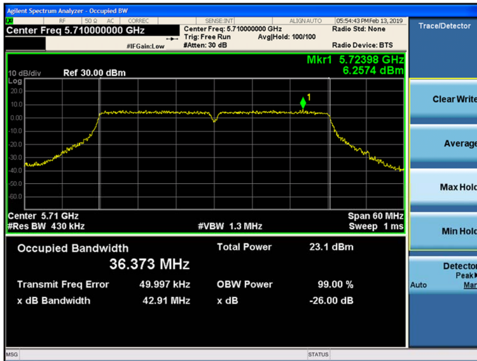
Figure 9-49. 26-dB Emission Bandwidth and 99% OBW SISO Chain B 802.11n HT40 (Ch. 142)
