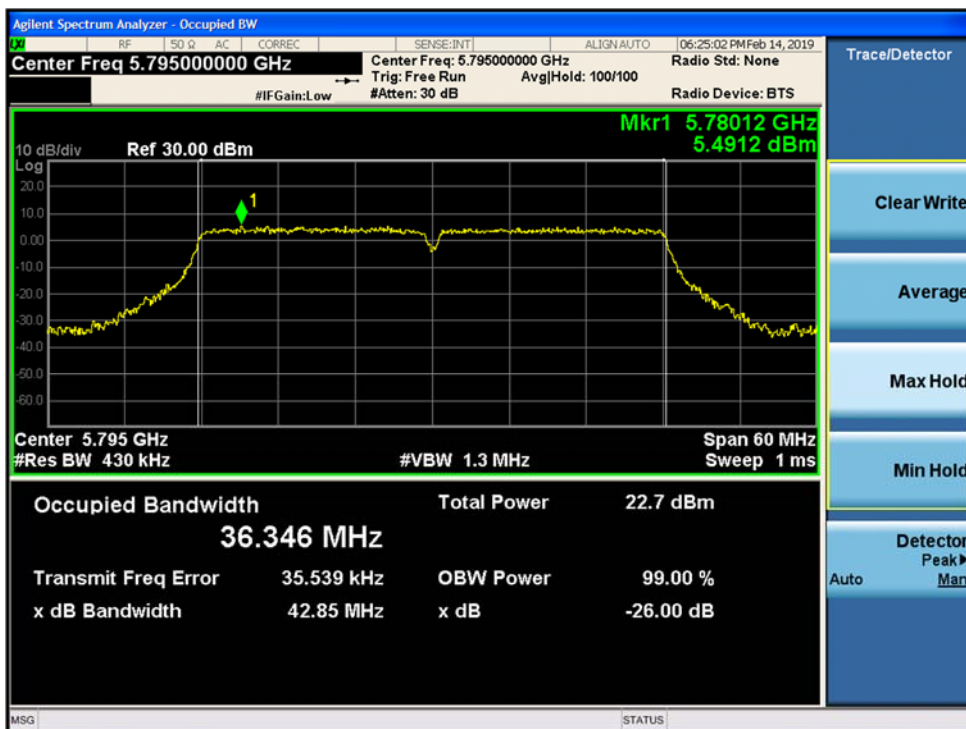
Figure 9-19. 26-dB Emission Bandwidth and 99% OBW SISO Chain A 802.11n HT40 (Ch. 159)
