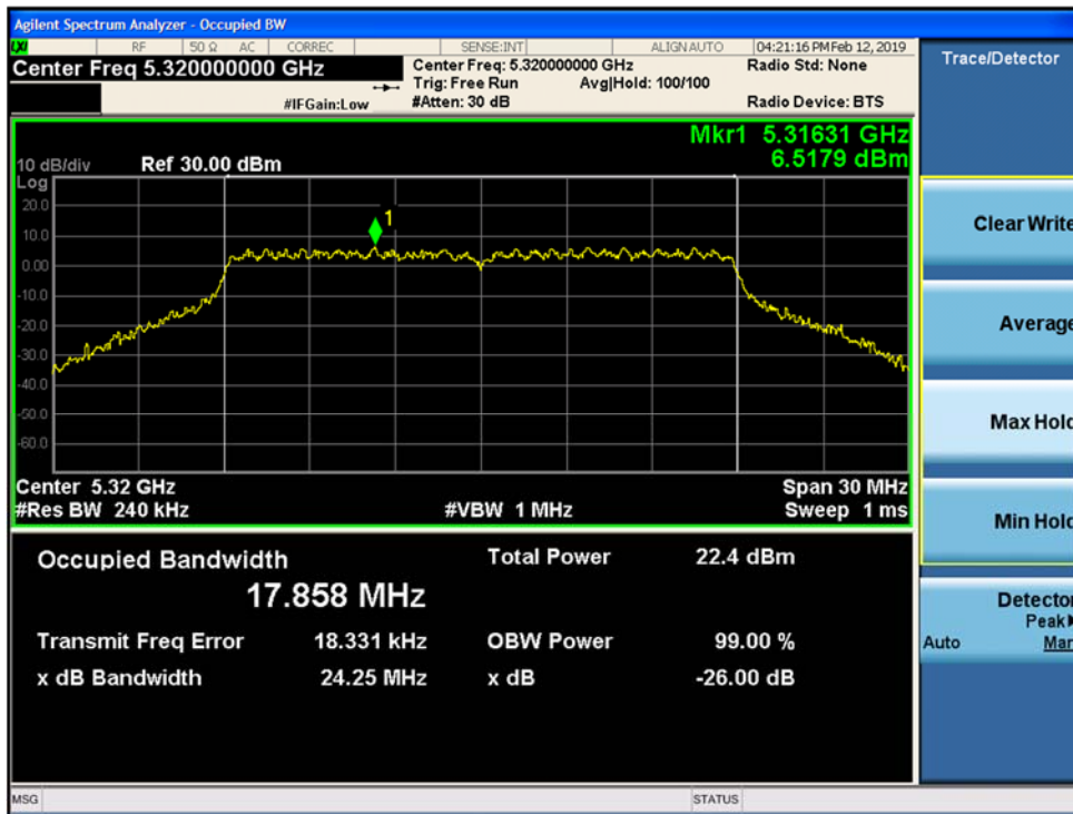
Figure 9-37. 26-dB Emission Bandwidth and 99% OBW MIMO Chain B 802.11n HT20 (Ch. 64)
