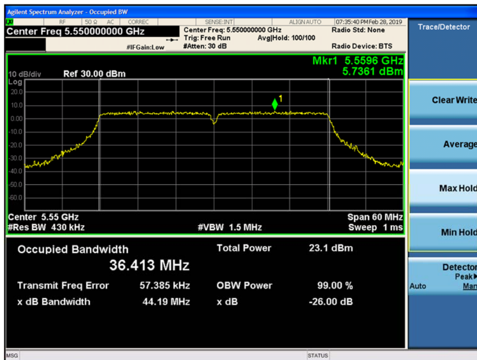
Figure 9-53. 26-dB Emission Bandwidth and 99% OBW MIMO Chain A 802.11n HT40 (Ch. 110)
