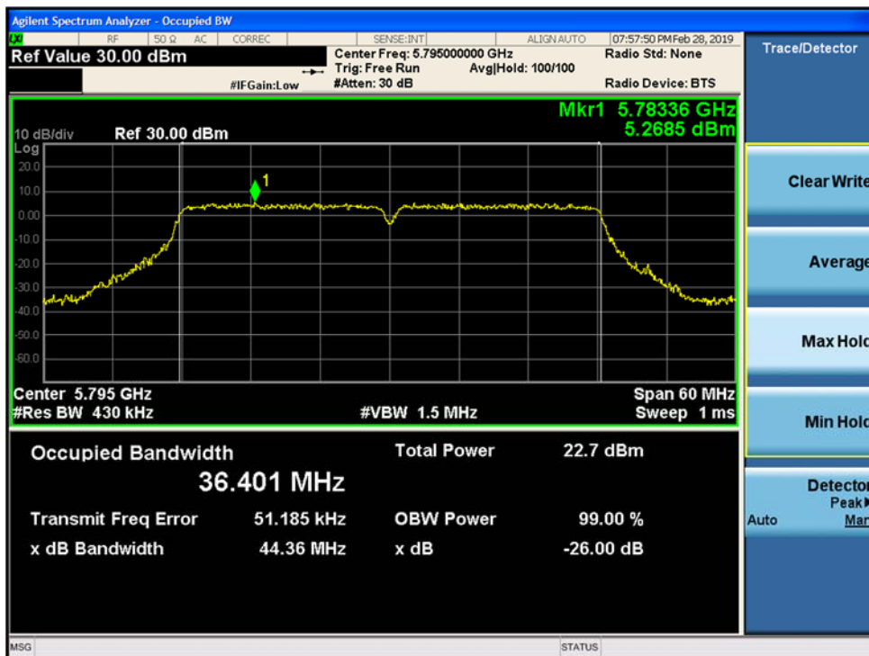
Figure 9-55. 26-dB Emission Bandwidth and 99% OBW MIMO Chain A 802.11n HT40 (Ch. 159)
