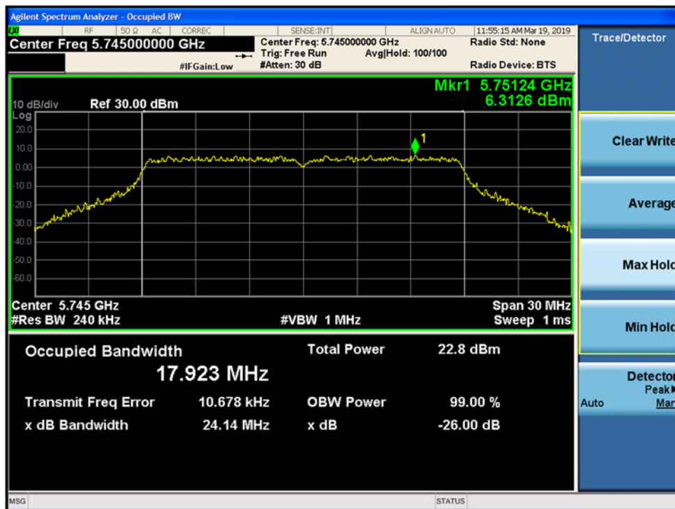
Figure 9-75. 26dB Emission Bandwidth and 99% OBW MIMO Chain A 802.11ac VHT 20 (CH. 149)
