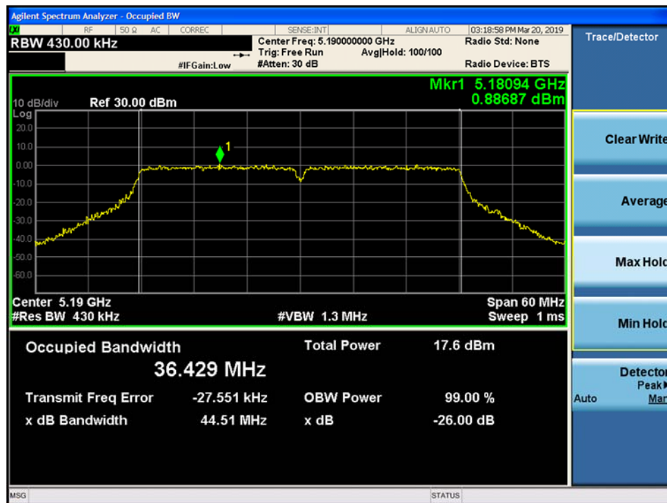
Figure 9-51. 26-dB Emission Bandwidth and 99% OBW MIMO Chain A 802.11n HT40 (Ch. 38)
