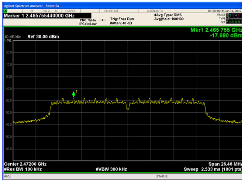
Plot 9-231 Chain B Reference Level 802.11n - Ch.13 (2472 MHz)
