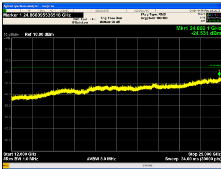
Plot 9-206 Chain B Conducted Spurious Emissions 12 - 25 GHz 802.11g - Ch.1 (2412 MHz)
