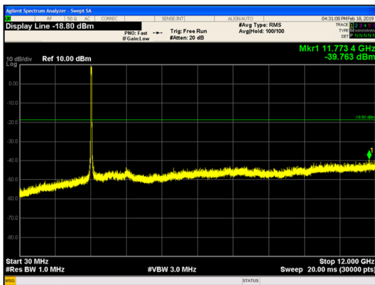
Plot 9-238 Chain B Conducted Spurious Emissions 30 MHz - 12 GHz 802.11n20 - Ch.7 (2442 MHz)
