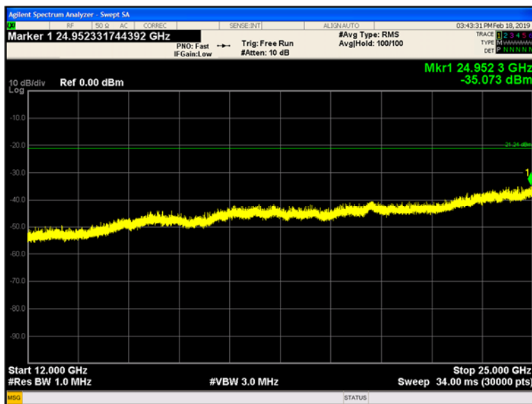
Plot 9-182 Chain A Conducted Spurious Emissions 12 - 25 GHz 802.11n40 - Ch.9 (2452 MHz)
