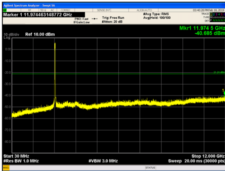
Plot 9-181 Chain A Conducted Spurious Emissions 30 MHz - 12 GHz 802.11n40 - Ch.9 (2452 MHz)
