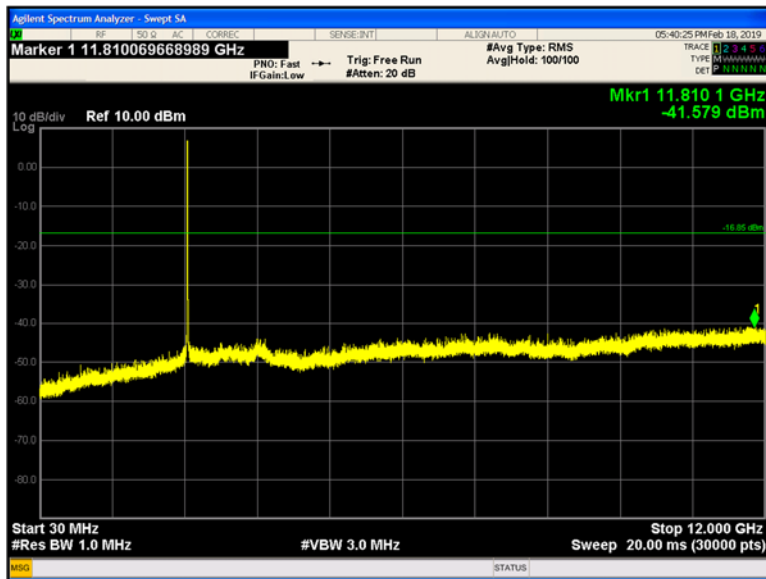
Plot 9-199 Chain B Conducted Spurious Emissions 3 0MHz - 12 GHz 802.11b - Ch.12 (2467 MHz)
