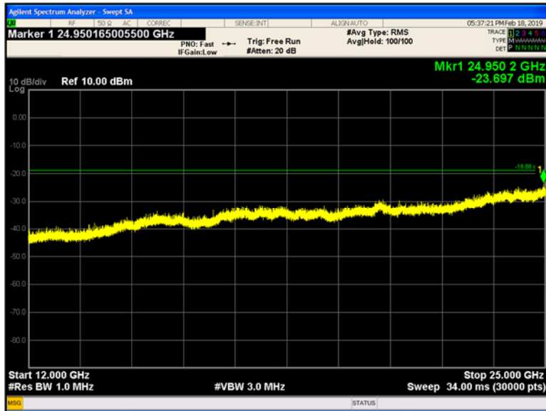
Plot 9-215 Chain B Conducted Spurious Emissions 12 - 25 GHz 802.11g - Ch.12 (2467 MHz)
