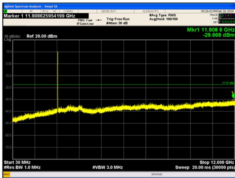
Plot 9-226 Chain B Conducted Spurious Emissions 30 MHz - 12 GHz 802.11n - Ch.11 (2462 MHz)
