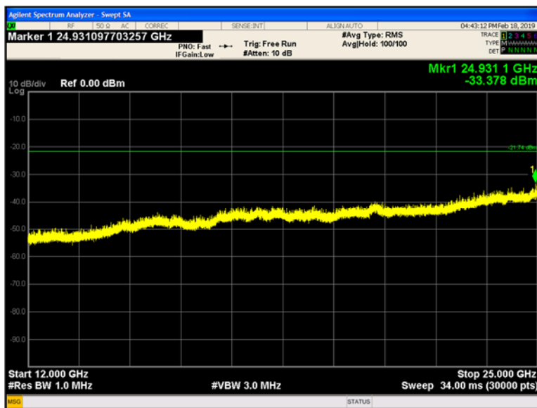
Plot 9-242 Chain B Conducted Spurious Emissions 12 - 25 GHz 802.11n40 - Ch.9 (2452 MHz)
