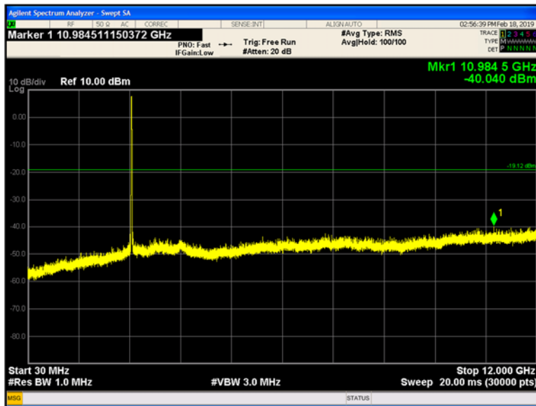
Plot 9-169 Chain A Conducted Spurious Emissions 30 MHz - 12 GHz 802.11n - Ch.12 (2467 MHz)
