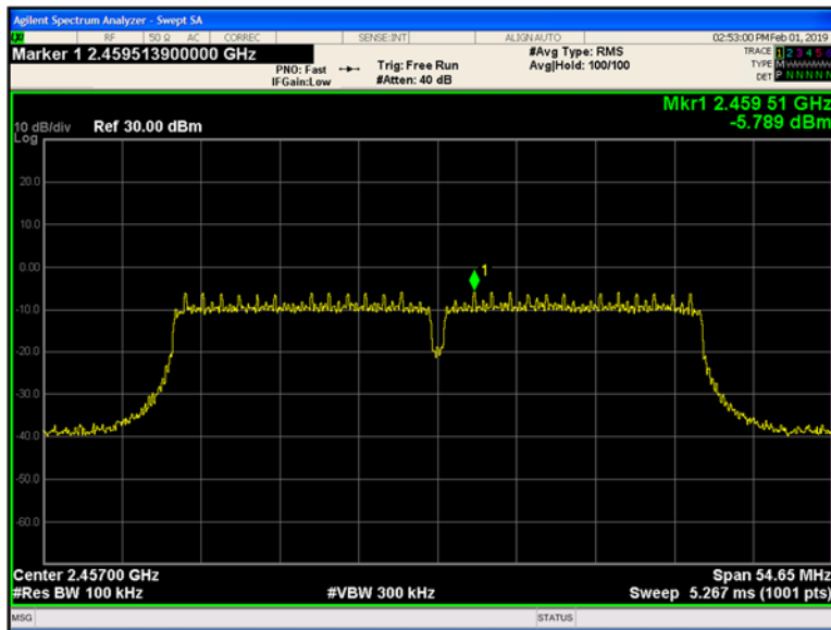
Plot 9-243 Chain B Reference Level 802.11n40 - Ch.10 (2457 MHz)
