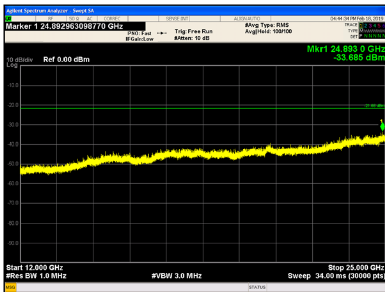
Plot 9-236 Chain B Conducted Spurious Emissions 12 - 25 GHz 802.11n40 - Ch.3 (2422 MHz)
