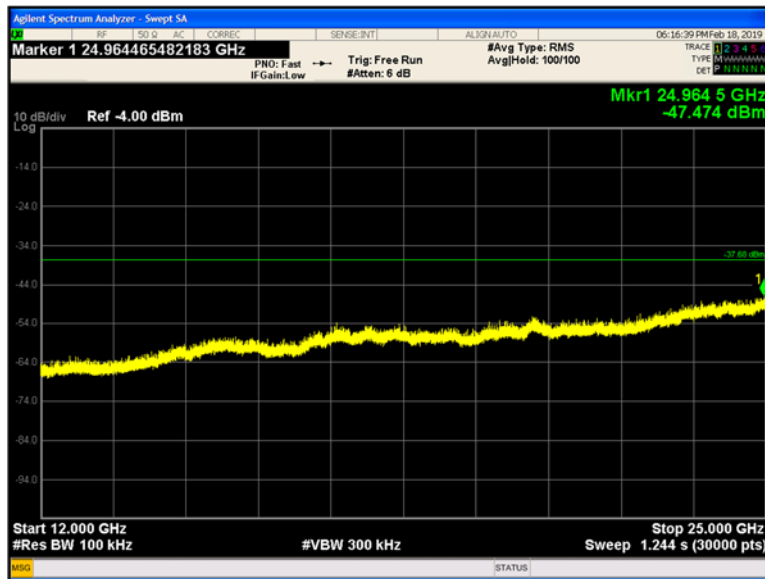
Plot 9-233 Chain B Conducted Spurious Emissions 12 - 25 GHz 802.11n - Ch.13 (2472 MHz)
