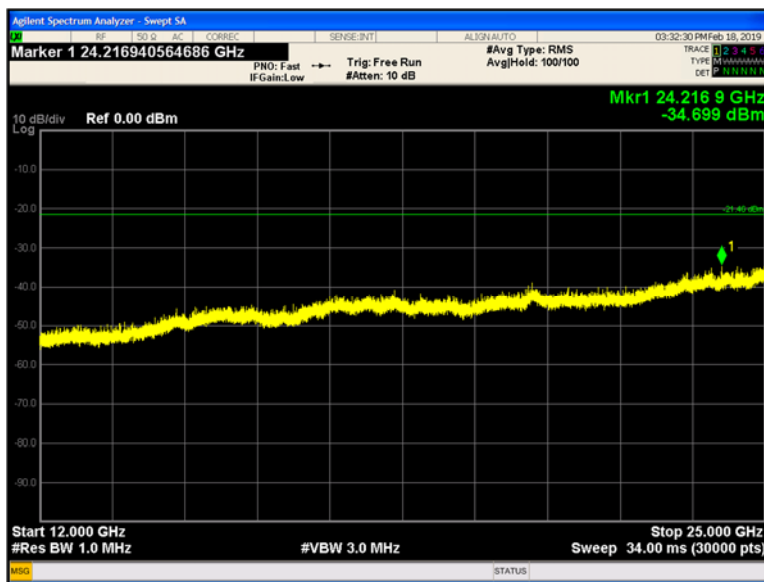
Plot 9-176 Chain A Conducted Spurious Emissions 12 - 25 GHz 802.11n40 - Ch.3 (2422 MHz)
