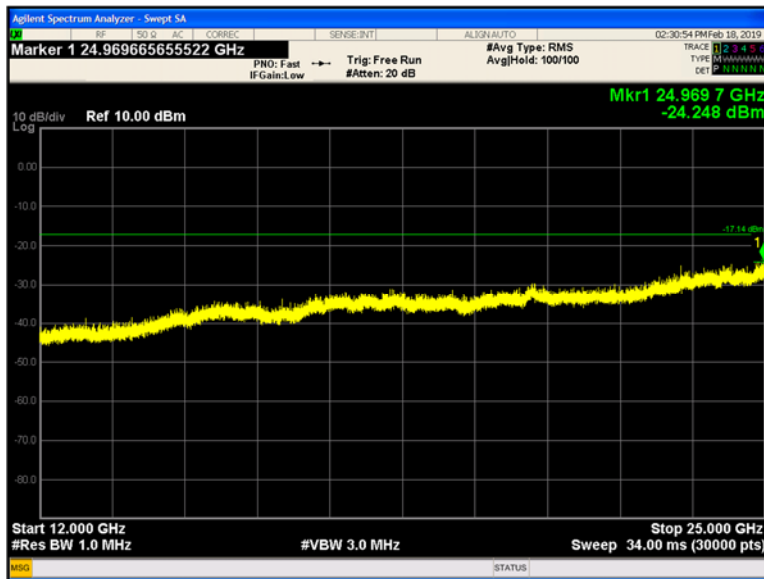
Plot 9-167 Chain A Conducted Spurious Emissions 12 - 25 GHz 802.11n - Ch.11 (2462 MHz)
