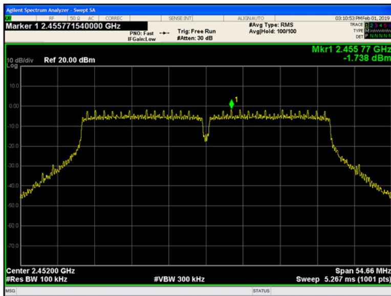
Plot 9-240 Chain B Reference Level 802.11n40 - Ch.9 (2452 MHz)
