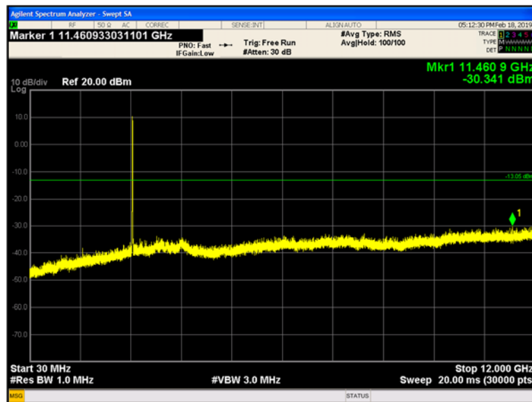
Plot 9-196 Chain B Conducted Spurious Emissions 3 0MHz - 12 GHz 802.11b - Ch.11 (2462 MHz)
