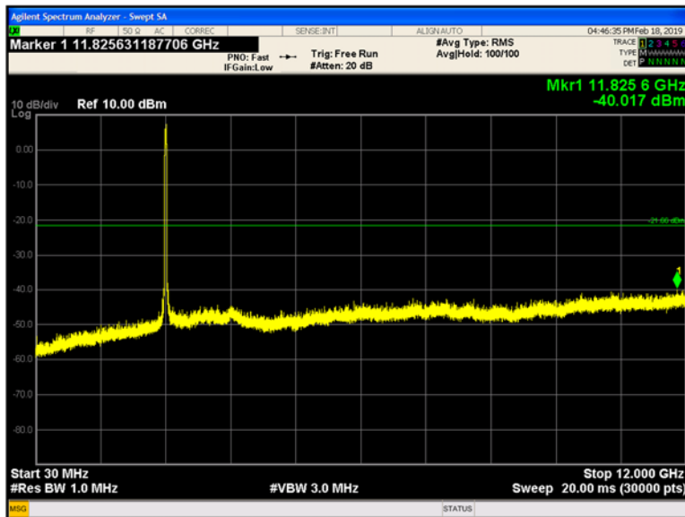
Plot 9-235 Chain B Conducted Spurious Emissions 30 MHz - 12 GHz 802.11n40 - Ch.3 (2422 MHz)
