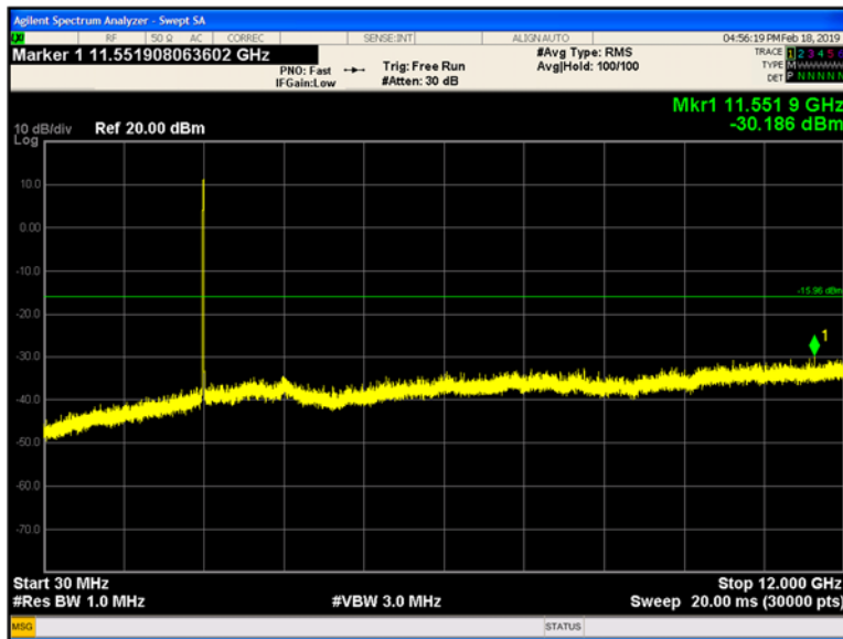
Plot 9-205 Chain B Conducted Spurious Emissions 30 MHz - 12 GHz 802.11g - Ch.1 (2412 MHz)
