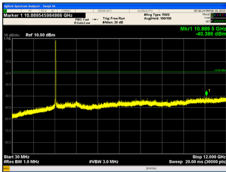
Plot 9-214 Chain B Conducted Spurious Emissions 30 MHz - 12 GHz 802.11g - Ch.12 (2467 MHz)
