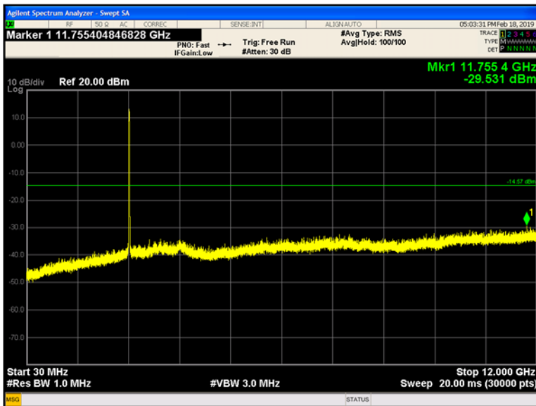
Plot 9-223 Chain B Conducted Spurious Emissions 30 MHz - 12 GHz 802.11n - Ch.6 (2437 MHz)
