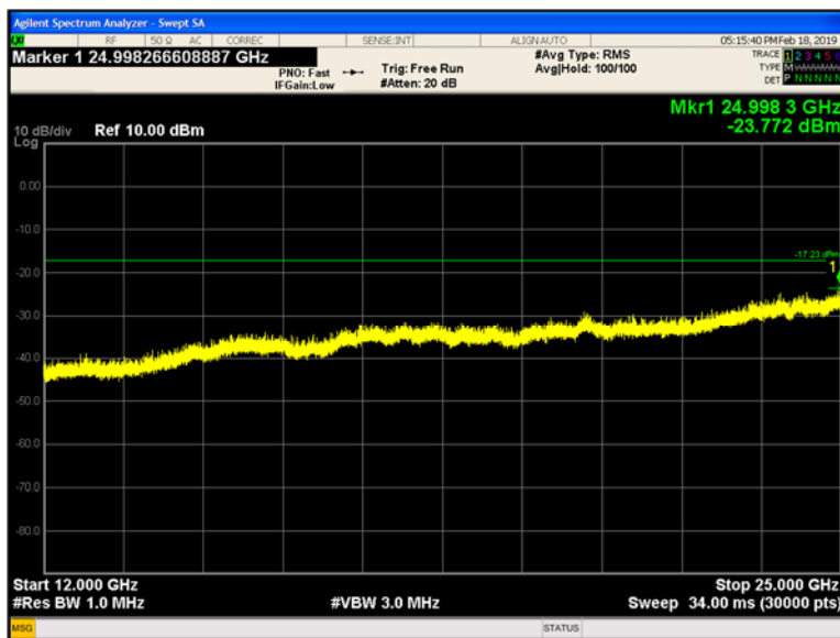
Plot 9-212 Chain B Conducted Spurious Emissions 12 - 25 GHz 802.11g - Ch.11 (2462 MHz)
