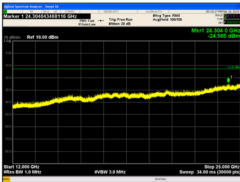
Plot 9-194 Chain B Conducted Spurious Emissions 12 - 25 GHz 802.11b - Ch.6 (2437 MHz)
