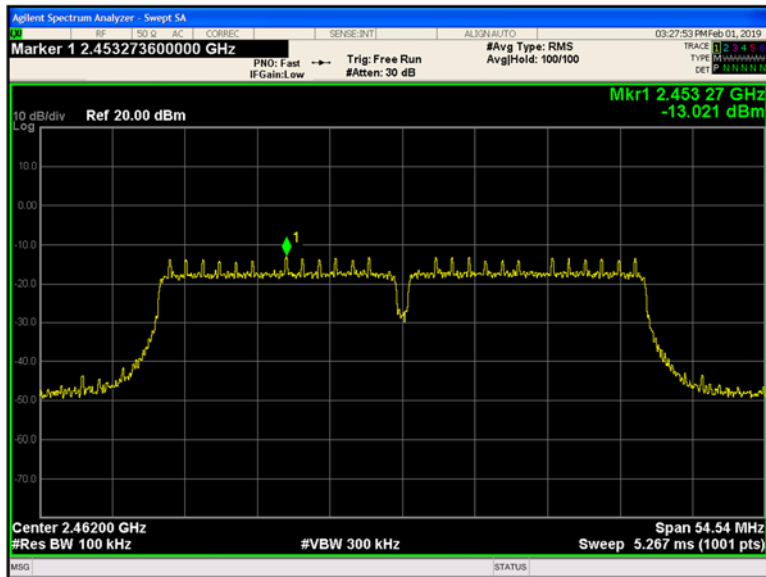
Plot 9-186 Chain A Reference Level 802.11n40 - Ch.11 (2462 MHz)
