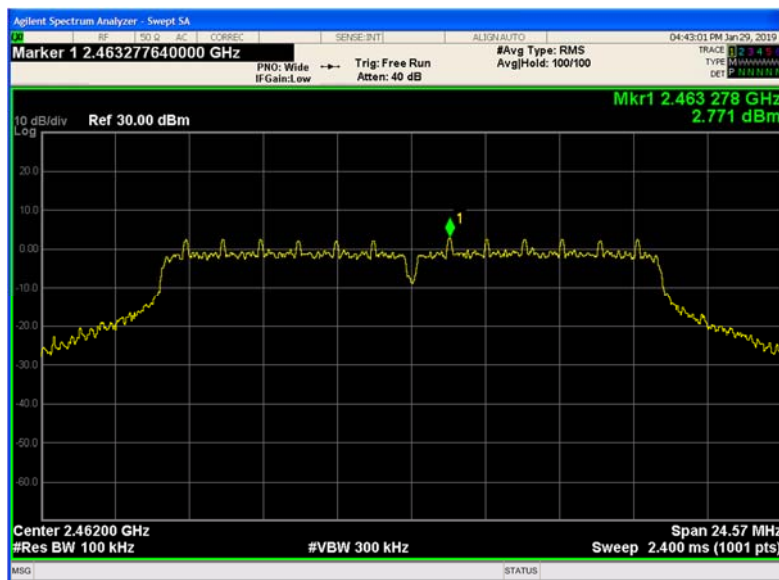
Plot 9-210 Chain B Reference Level 802.11g - Ch.11 (2462 MHz)
