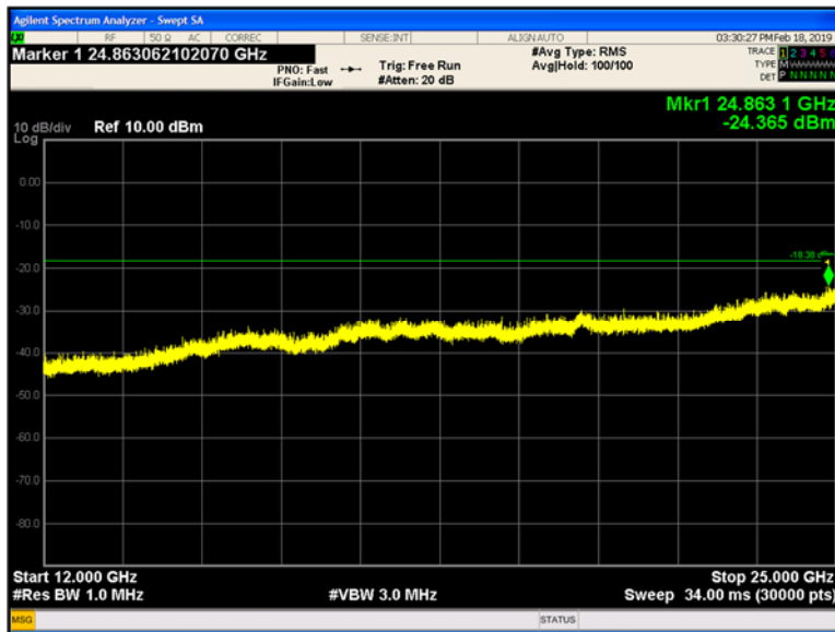
Plot 9-179 Chain A Conducted Spurious Emissions 12 - 25 GHz 802.11n40 - Ch.7 (2442 MHz)
