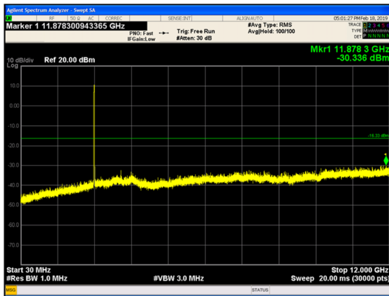
Plot 9-220 Chain B Conducted Spurious Emissions 30 MHz - 12 GHz 802.11n - Ch.1 (2412 MHz)
