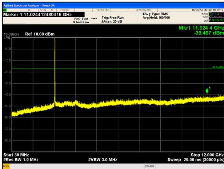
Plot 9-166 Chain A Conducted Spurious Emissions 30 MHz - 12 GHz 802.11n - Ch.11 (2462 MHz)
