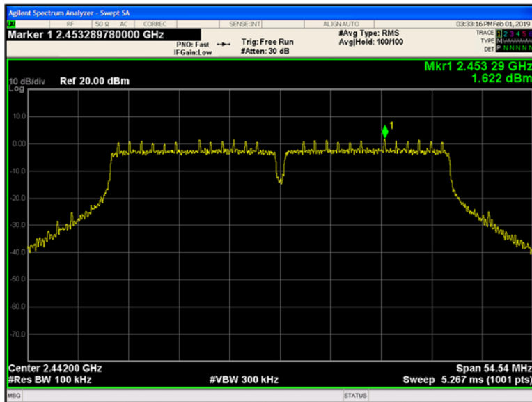
Plot 9-177 Chain A Reference Level 802.11n40 - Ch.7 (2442 MHz)
