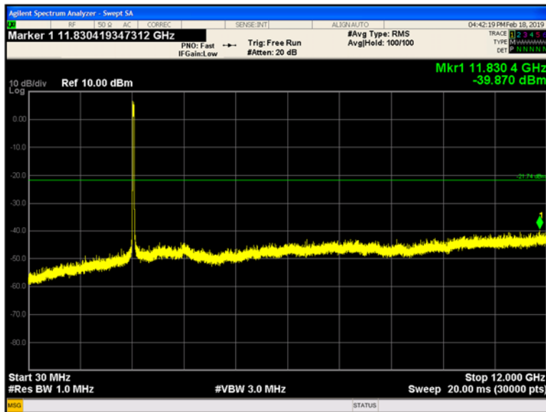
Plot 9-241 Chain B Conducted Spurious Emissions 30 MHz - 12 GHz 802.11n40 - Ch.9 (2452 MHz)
