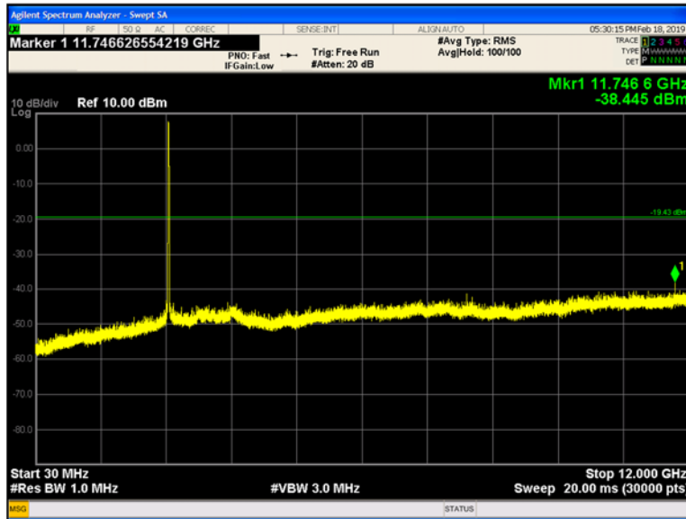
Plot 9-229 Chain B Conducted Spurious Emissions 30 MHz - 12 GHz 802.11n - Ch.12 (2467 MHz)
