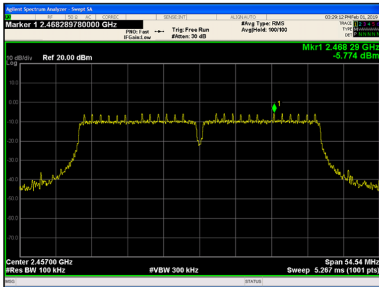
Plot 9-183 Chain A Reference Level 802.11n40 - Ch.10 (2457 MHz)
