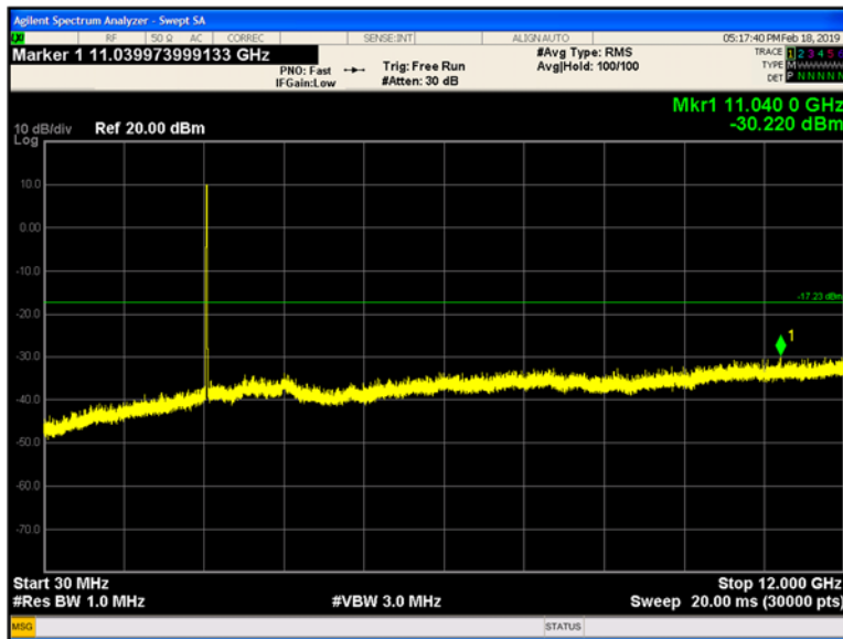
Plot 9-211 Chain B Conducted Spurious Emissions 30 MHz - 12 GHz 802.11g - Ch.11 (2462 MHz)
