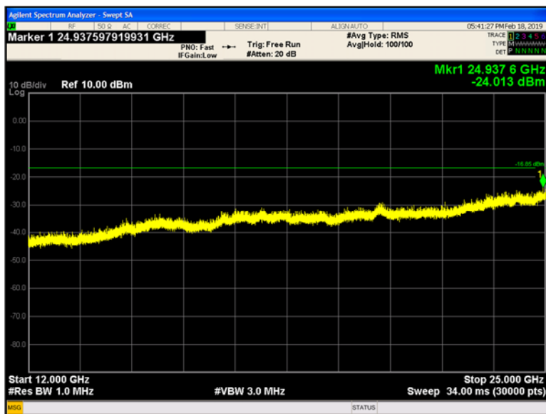
Plot 9-200 Chain B Conducted Spurious Emissions 12 - 25 GHz 802.11b - Ch.12 (2467 MHz)
