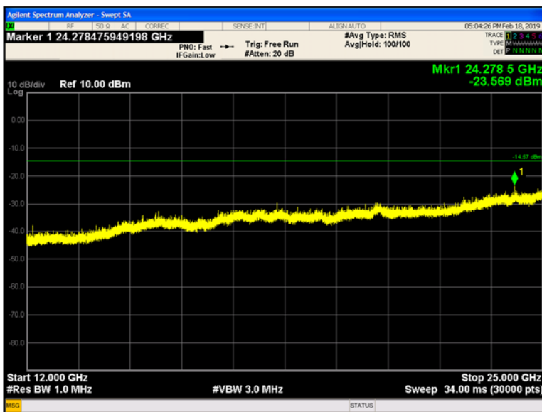
Plot 9-224 Chain B Conducted Spurious Emissions 12 - 25 GHz 802.11n - Ch.6 (2437 MHz)
