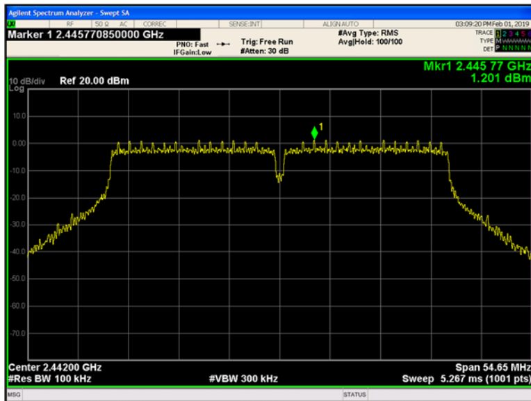
Plot 9-237 Chain B Reference Level 802.11n40 - Ch.7 (2442 MHz)
