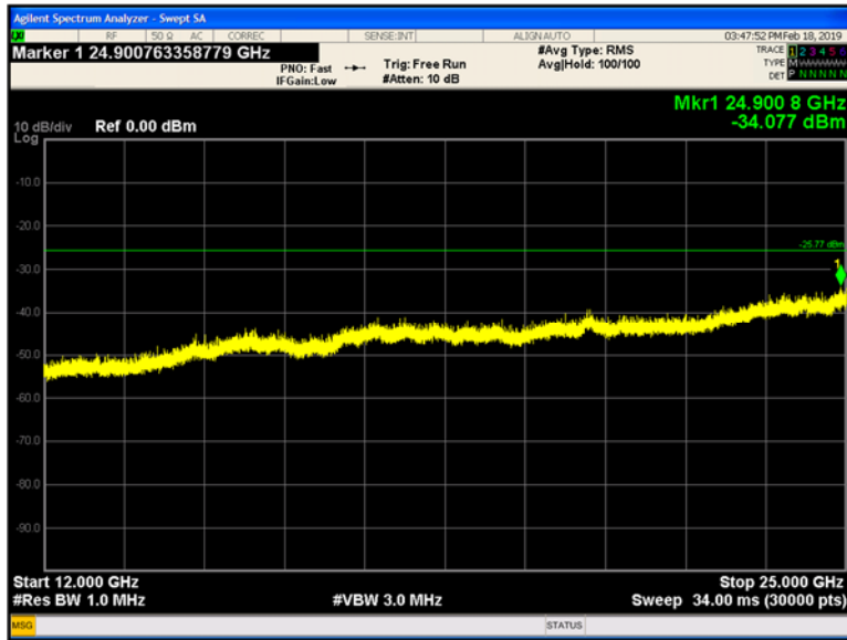
Plot 9-185 Chain A Conducted Spurious Emissions 12 - 25 GHz 802.11n40 - Ch.10 (2457 MHz)
