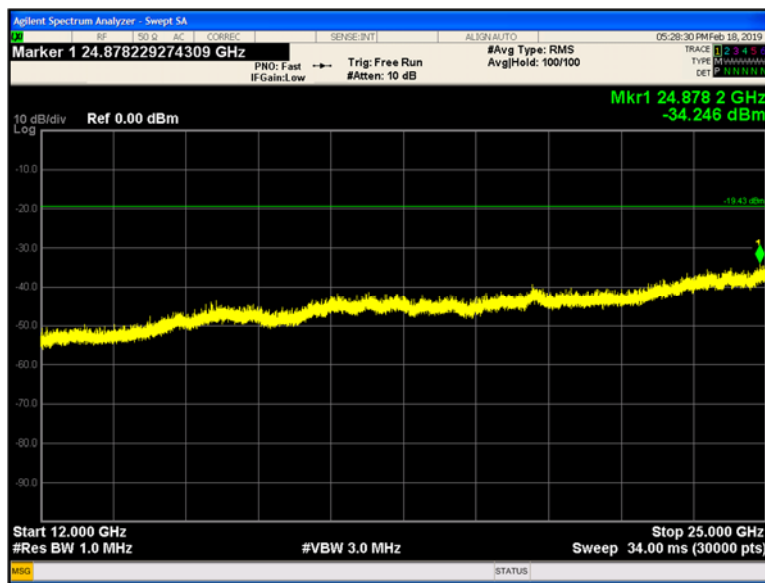
Plot 9-230 Chain B Conducted Spurious Emissions 12 - 25 GHz 802.11n - Ch.12 (2467 MHz)
