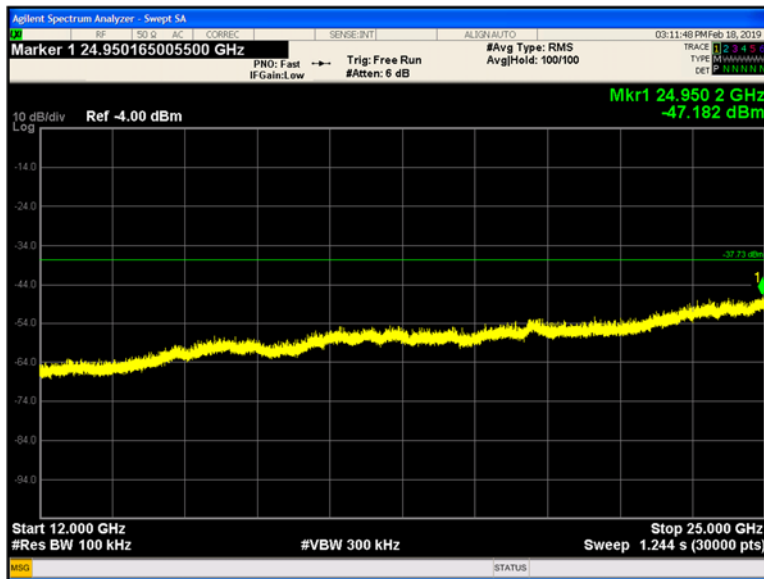
Plot 9-173 Chain A Conducted Spurious Emissions 12 - 25 GHz 802.11n - Ch.13 (2472 MHz)
