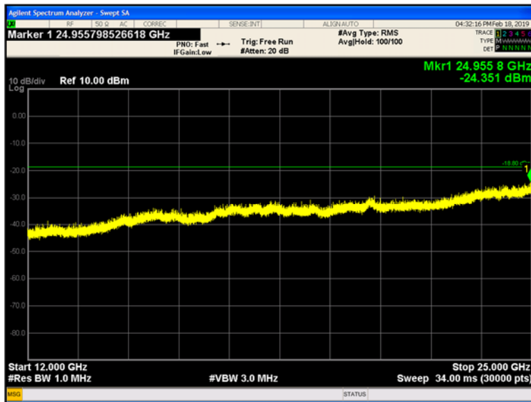
Plot 9-239 Chain B Conducted Spurious Emissions 12 - 25 GHz 802.11n40 - Ch.7 (2442 MHz)
