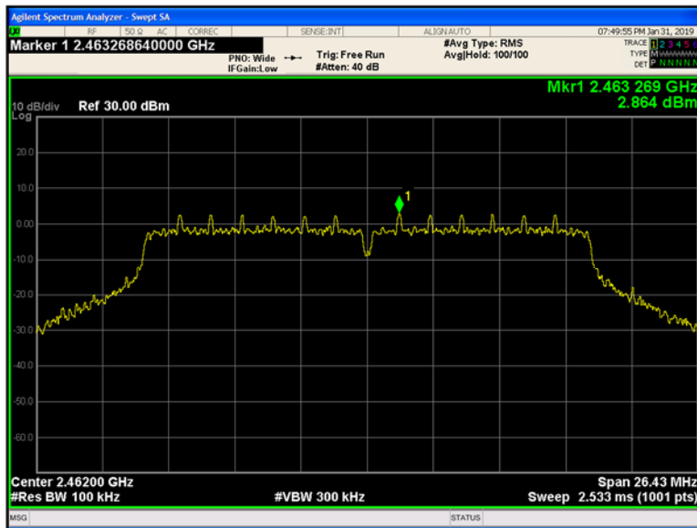
Plot 9-165 Chain A Reference Level 802.11n - Ch.11 (2462 MHz)
