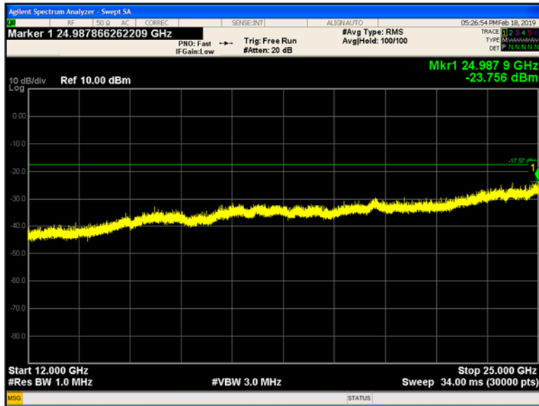
Plot 9-227 Chain B Conducted Spurious Emissions 12 - 25 GHz 802.11n - Ch.11 (2462 MHz)
