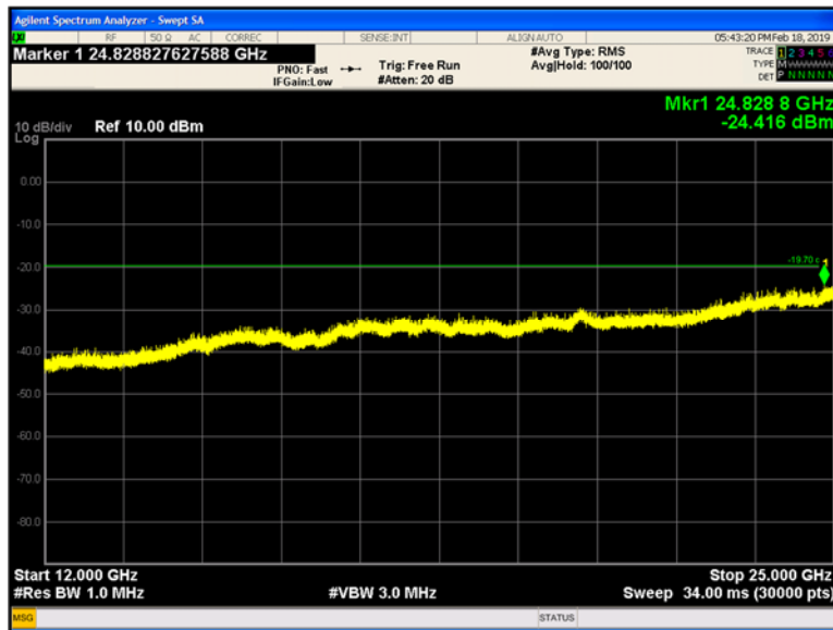
Plot 9-203 Chain B Conducted Spurious Emissions 12 - 25 GHz 802.11b - Ch.13 (2472 MHz)
