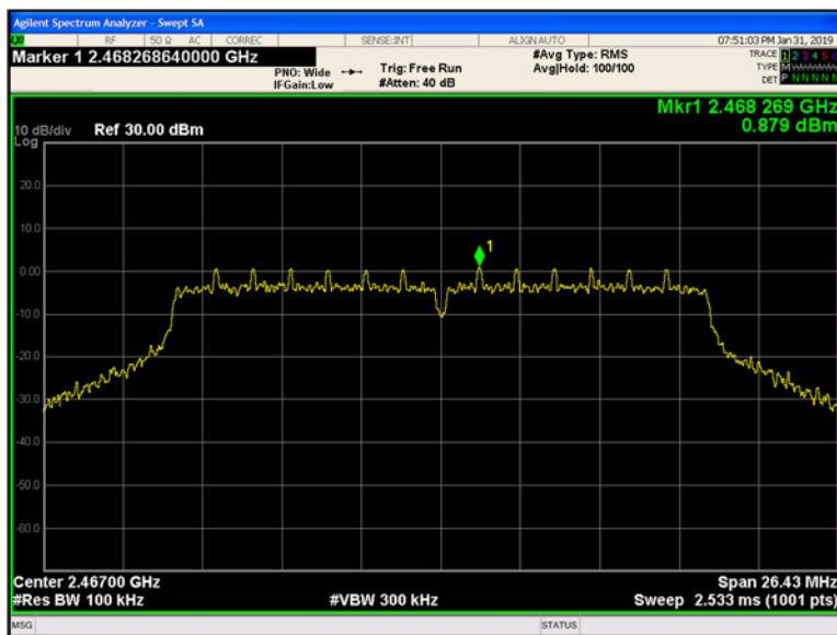
Plot 9-168 Chain A Reference Level 802.11n - Ch.12 (2467 MHz)
