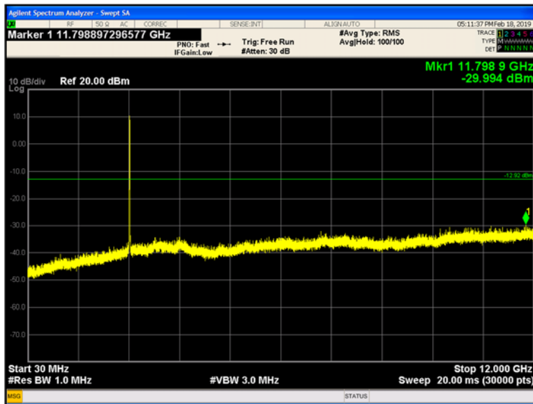
Plot 9-193 Chain B Conducted Spurious Emissions 30 MHz - 12 GHz 802.11b - Ch.6 (2437 MHz)
