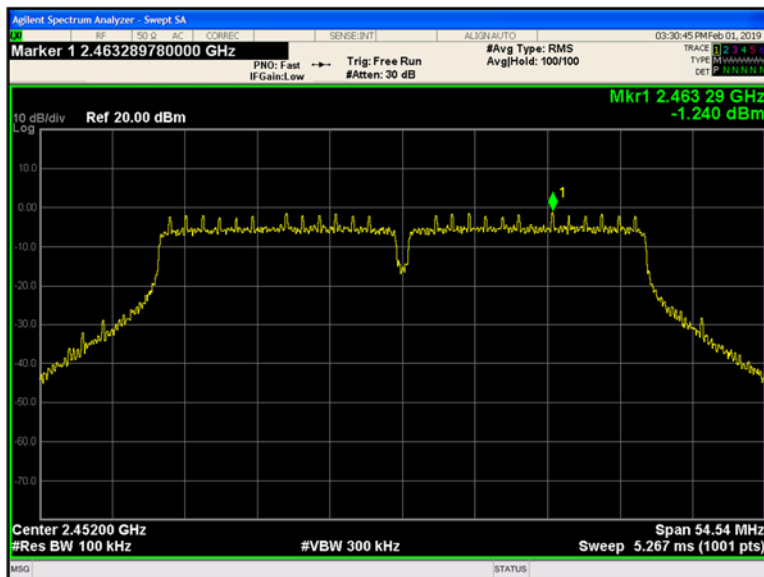
Plot 9-180 Chain A Reference Level 802.11n40 - Ch.9 (2452 MHz)
