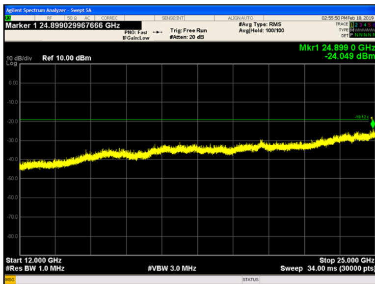
Plot 9-170 Chain A Conducted Spurious Emissions 12 - 25 GHz 802.11n - Ch.12 (2467 MHz)
