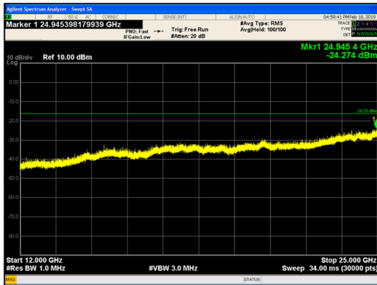
Plot 9-221 Chain B Conducted Spurious Emissions 12 - 25 GHz 802.11n - Ch.1 (2412 MHz)
