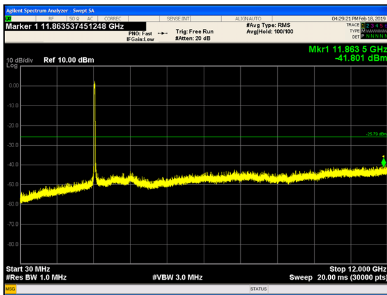
Plot 9-244 Chain B Conducted Spurious Emissions 30 MHz - 12 GHz 802.11n40 - Ch.10 (2457 MHz)
