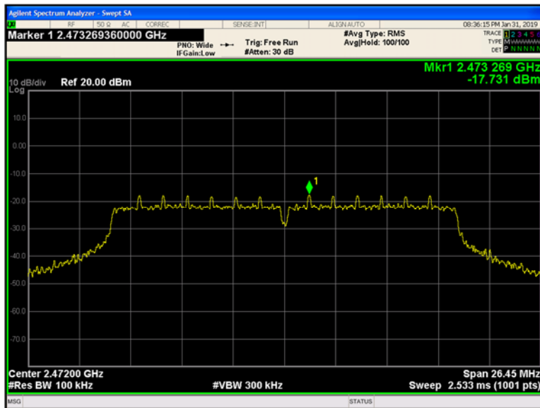
Plot 9-171 Chain A Reference Level 802.11n - Ch.13 (2472 MHz)
