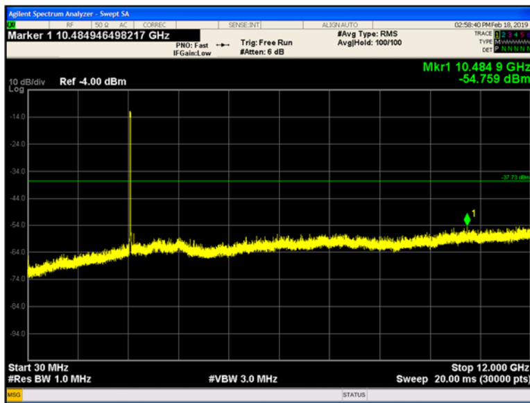
Plot 9-172 Chain A Conducted Spurious Emissions 30 MHz - 12 GHz 802.11n - Ch.13 (2472 MHz)
