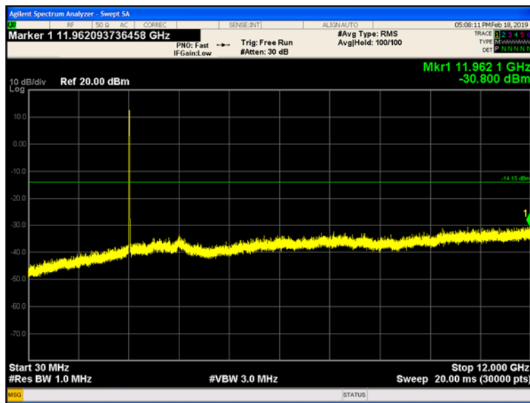
Plot 9-208 Chain B Conducted Spurious Emissions 30 MHz - 12 GHz 802.11g - Ch.6 (2437 MHz)
