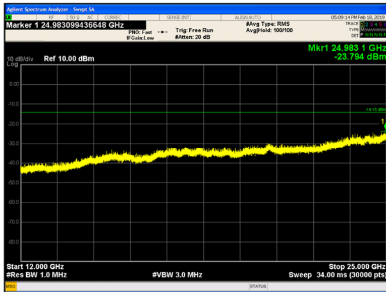
Plot 9-209 Chain B Conducted Spurious Emissions 12 - 25 GHz 802.11g - Ch.6 (2437 MHz)
