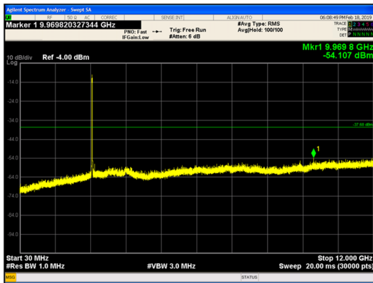
Plot 9-232 Chain B Conducted Spurious Emissions 30 MHz - 12 GHz 802.11n - Ch.13 (2472 MHz)
