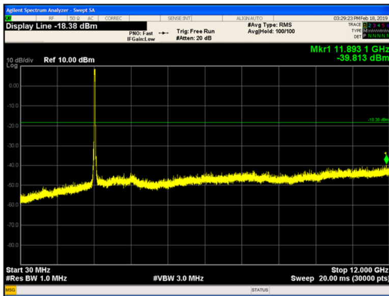
Plot 9-178 Chain A Conducted Spurious Emissions 30 MHz - 12 GHz 802.11n20 - Ch.7 (2442 MHz)
