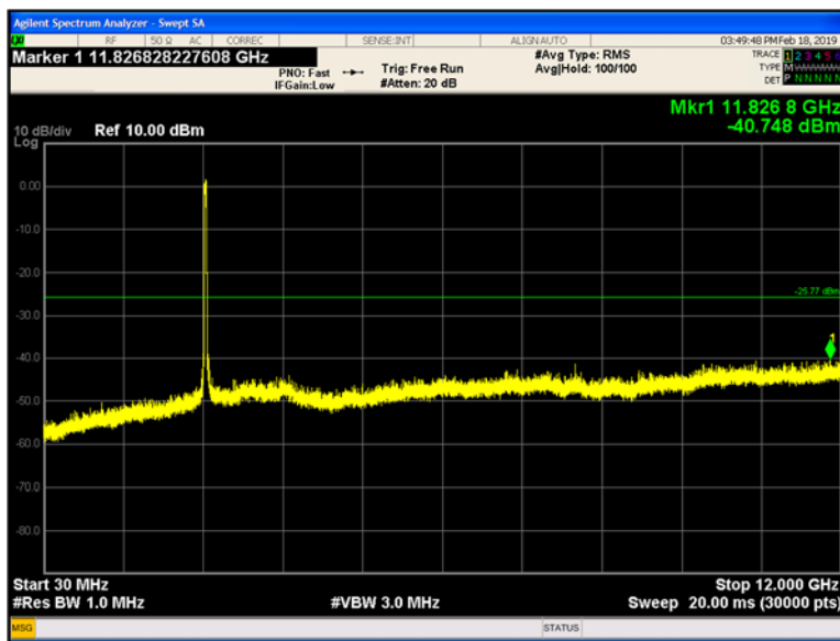
Plot 9-184 Chain A Conducted Spurious Emissions 30 MHz - 12 GHz 802.11n40 - Ch.10 (2457 MHz)
