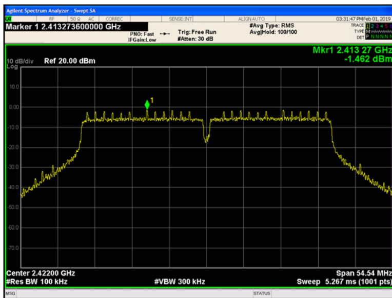
Plot 9-174 Chain A Reference Level 802.11n40 - Ch.3 (2422 MHz)
