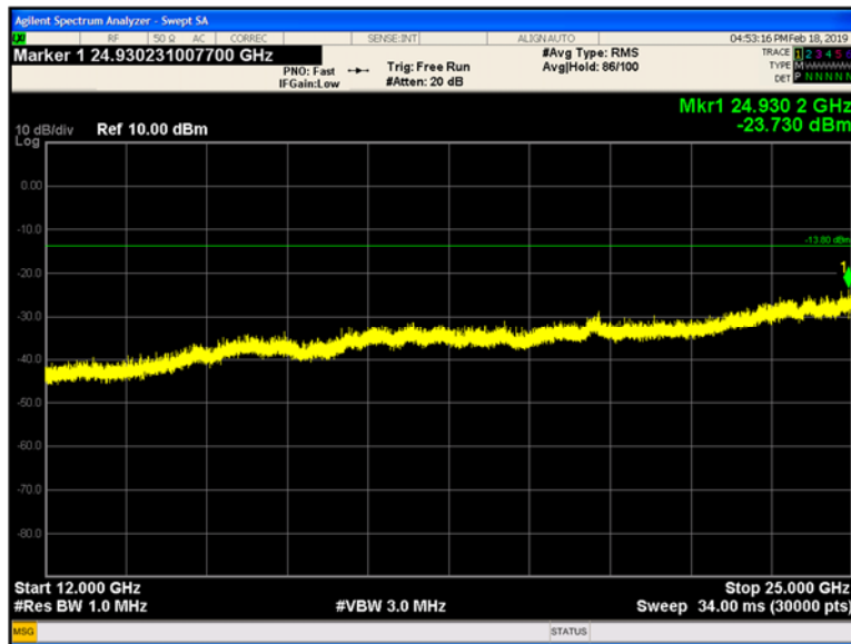
Plot 9-191 Chain B Conducted Spurious Emissions 12 - 25 GHz 802.11b - Ch.1 (2412 MHz)
