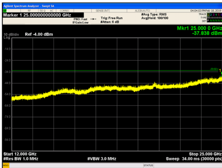
Plot 9-188 Chain A Conducted Spurious Emissions 12 - 25 GHz 802.11n40 - Ch.11 (2462 MHz)
