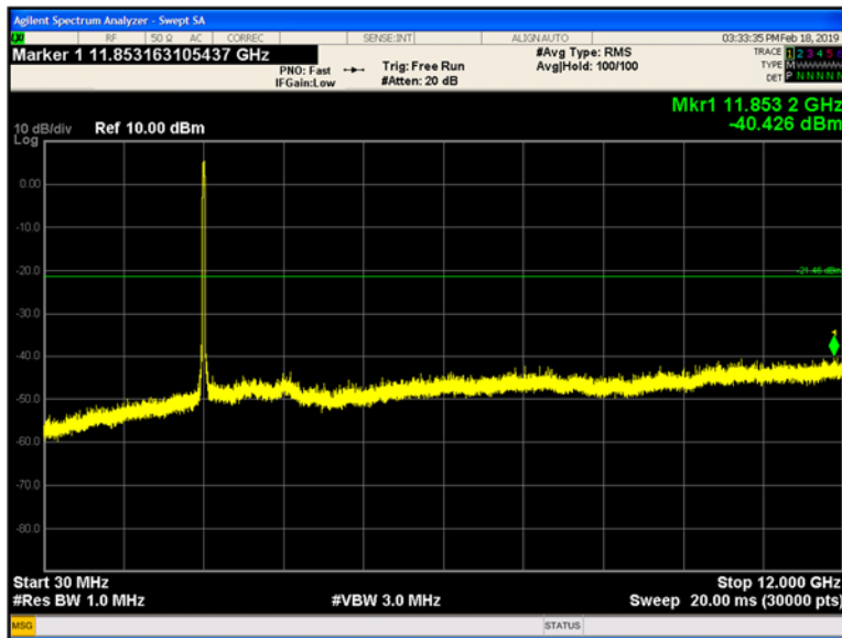
Plot 9-175 Chain A Conducted Spurious Emissions 30 MHz - 12 GHz 802.11n40 - Ch.3 (2422 MHz)
