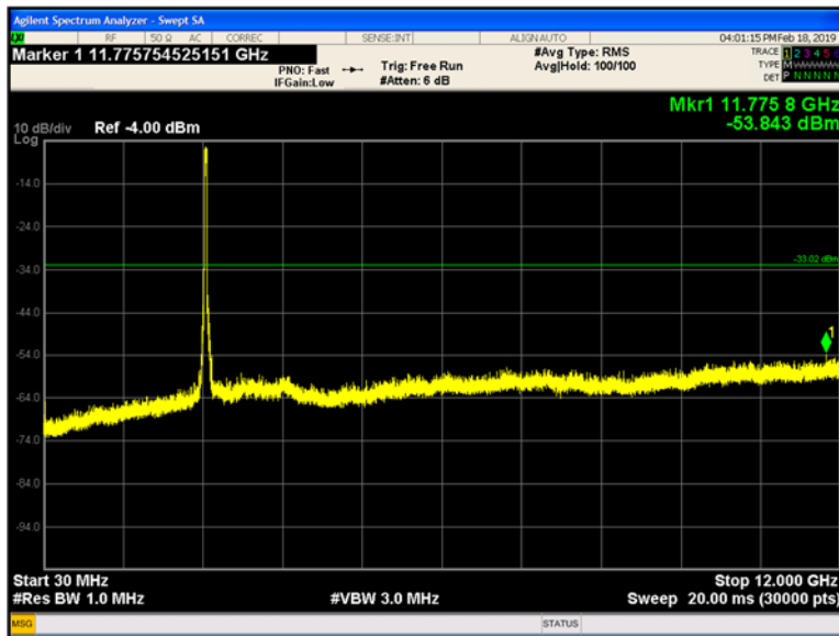
Plot 9-187 Chain A Conducted Spurious Emissions 30 MHz - 12 GHz 802.11n40 - Ch.11 (2462 MHz)
