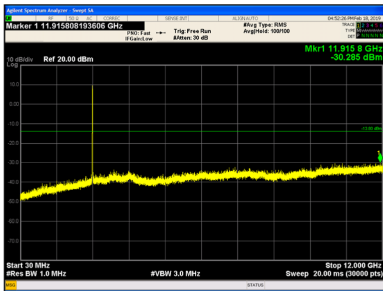
Plot 9-190 Chain B Conducted Spurious Emissions 30 MHz - 12 GHz 802.11b - Ch.1 (2412 MHz)
