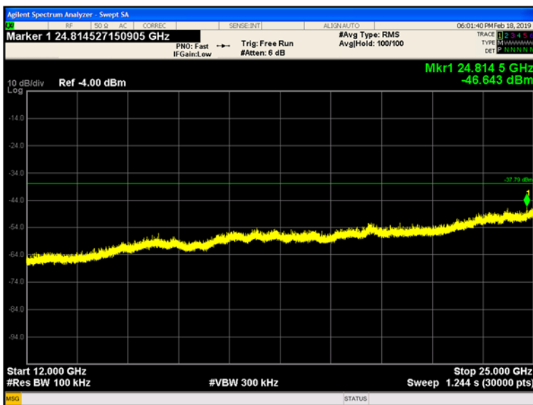
Plot 9-218 Chain B Conducted Spurious Emissions 12 - 25 GHz 802.11g - Ch.13 (2472 MHz)
