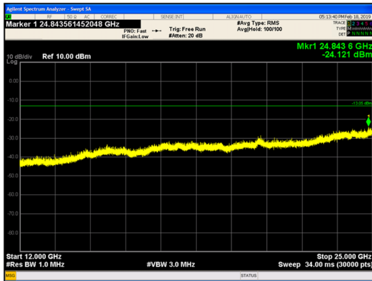
Plot 9-197 Chain B Conducted Spurious Emissions 12 - 25 GHz 802.11b - Ch.11 (2462 MHz)
