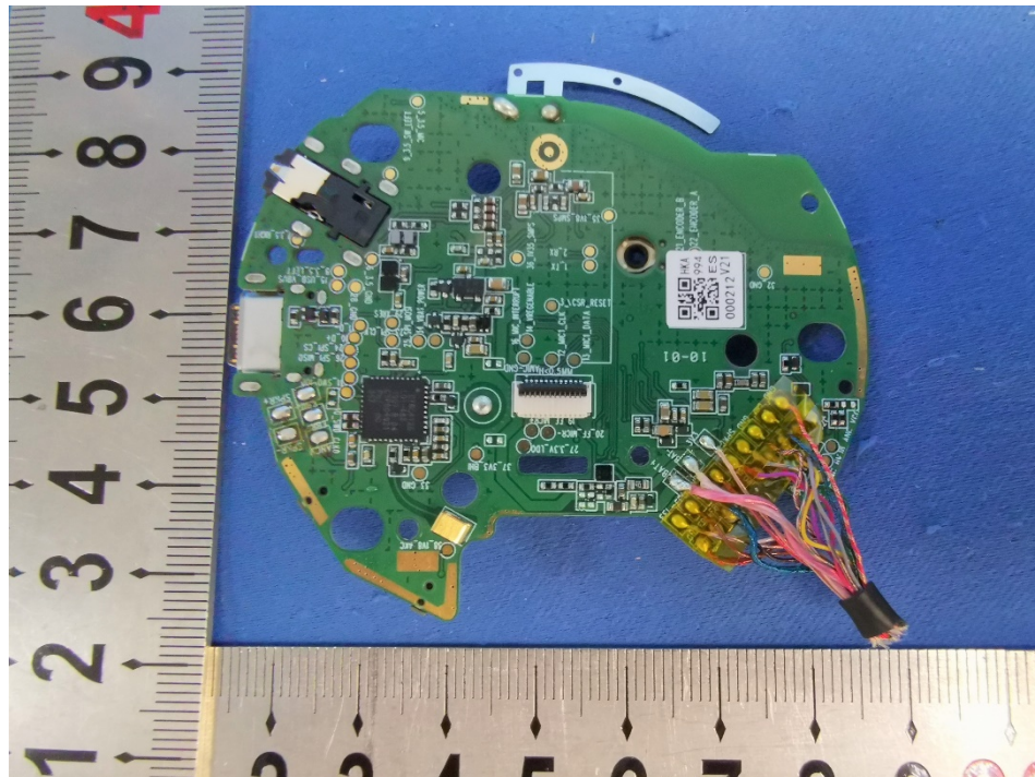
Right PCB – bottom side
