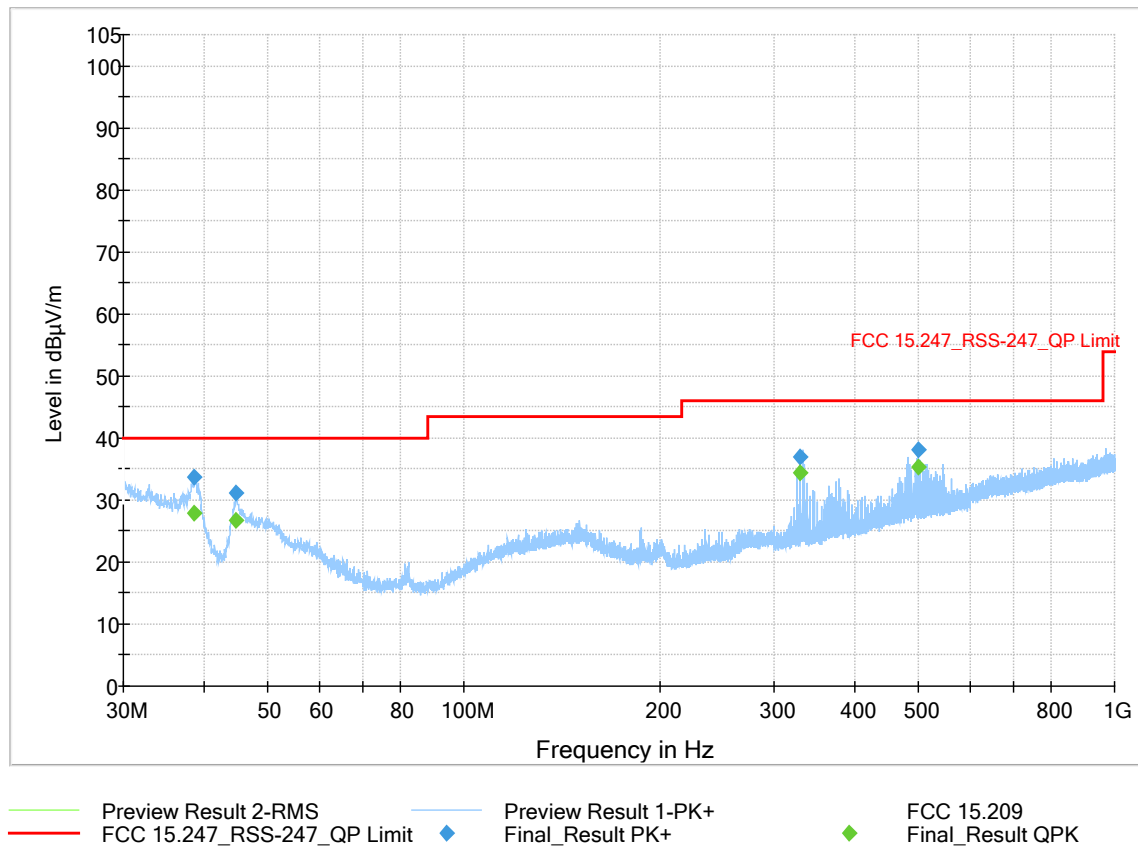
Figure 9-30 Radiated Spurious Emissions (30MHz - 1GHz) – Ambient emissions, Radio OFF
