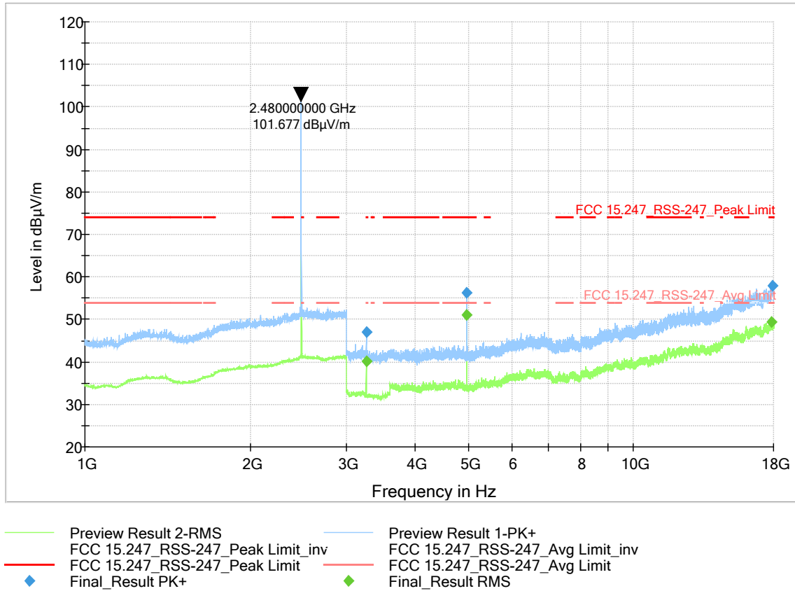
Figure 9-34 Radiated Spurious Emissions 1-18 GHz (Ch. 39)
