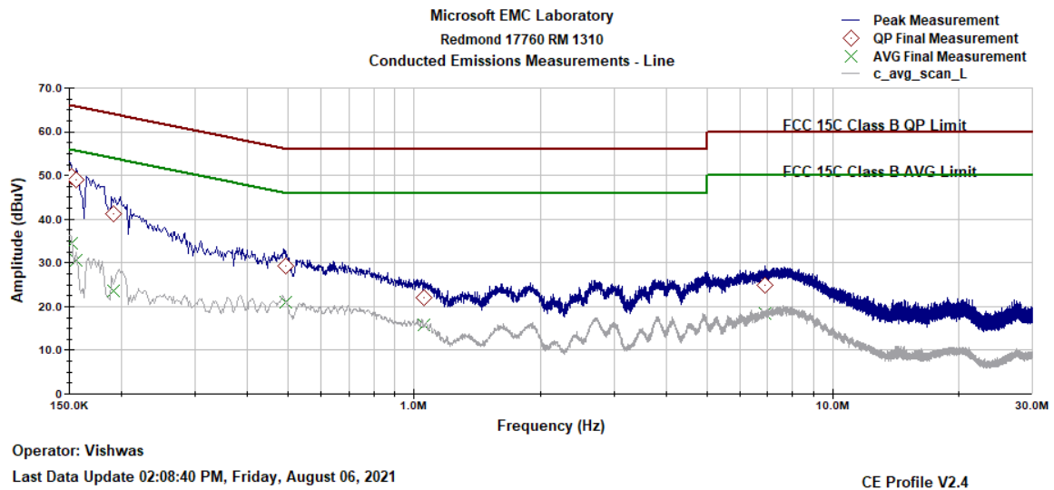
Figure 9-37 AC Line Conducted Emissions- Line (150 kHz- 30 MHz)
