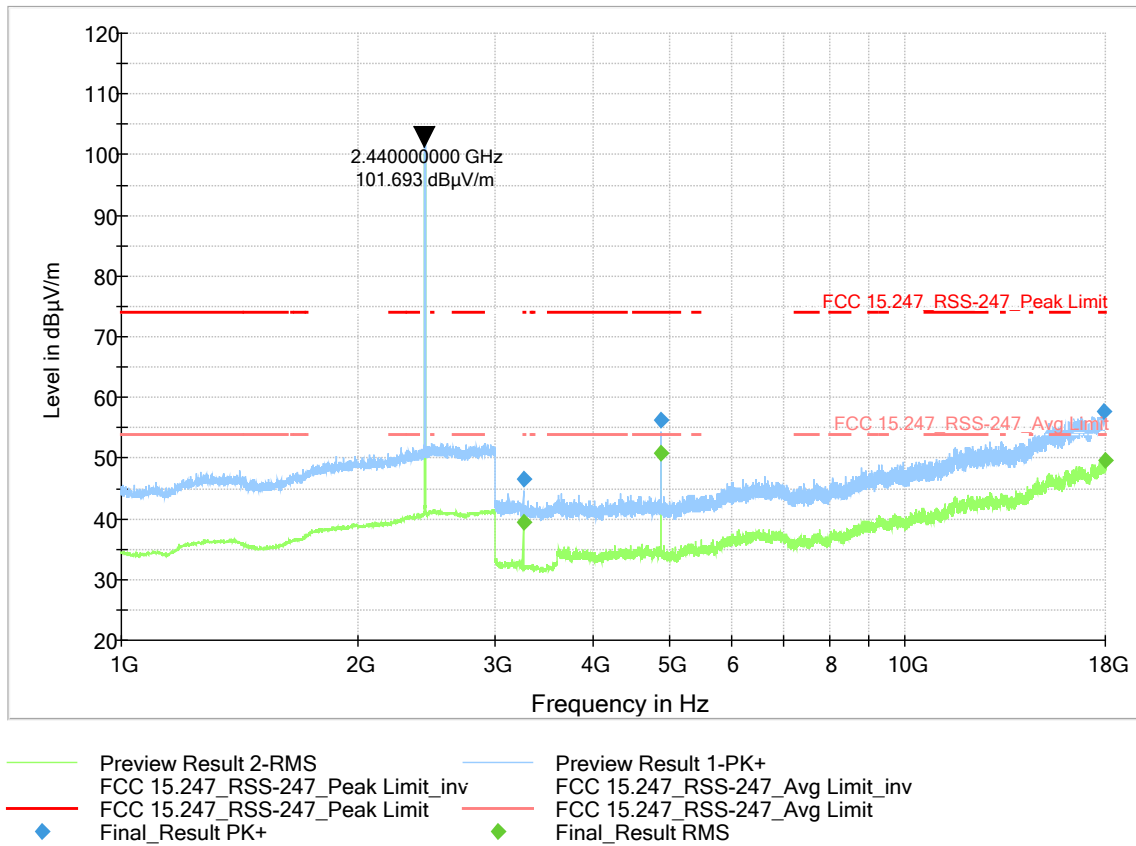
Figure 9-33 Radiated Spurious Emissions 1-18 GHz (Ch. 19)
