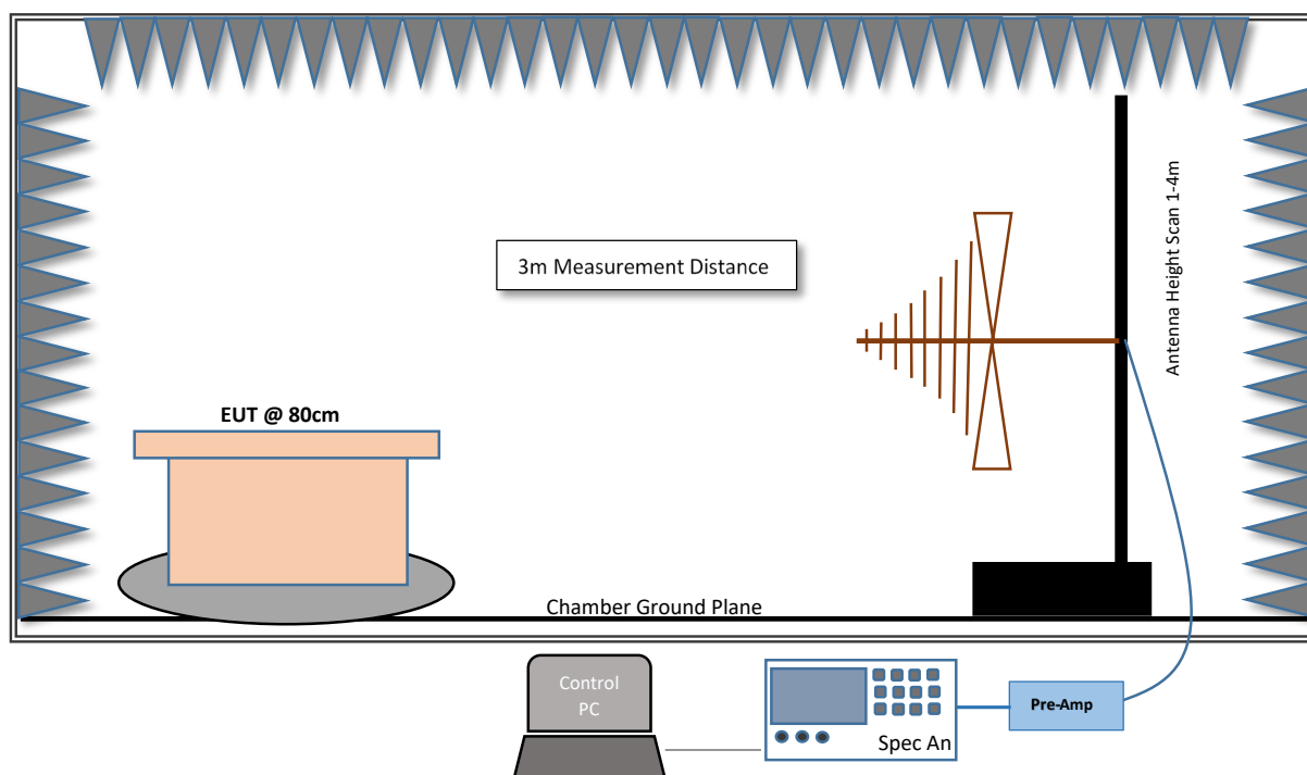
Fig.4. Test Setup for Radiated measurements in 30MHz- 1GHz Range
