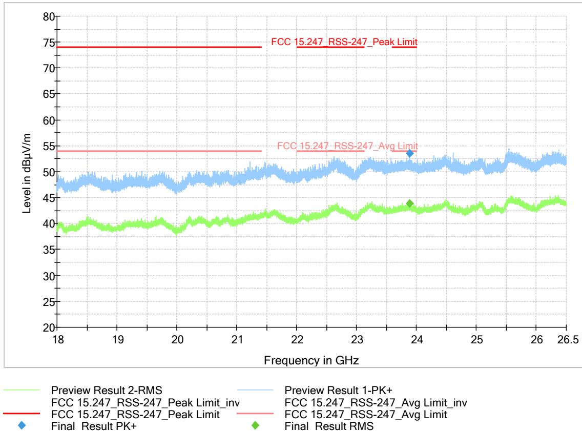
Figure 9-35 Radiated Spurious Emissions (Ch. 19) (18 – 26.5 GHz)
