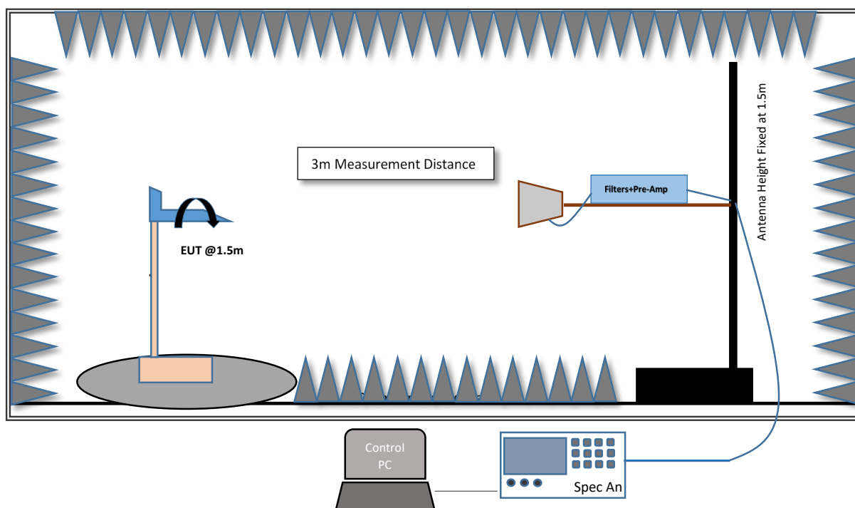
Fig.5. Test Setup for Radiated measurements in 1GHz- 18GHz Range
