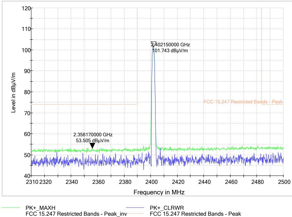
Figure 9-25 Radiated Restricted Band Edge (Ch. 0) Peak
