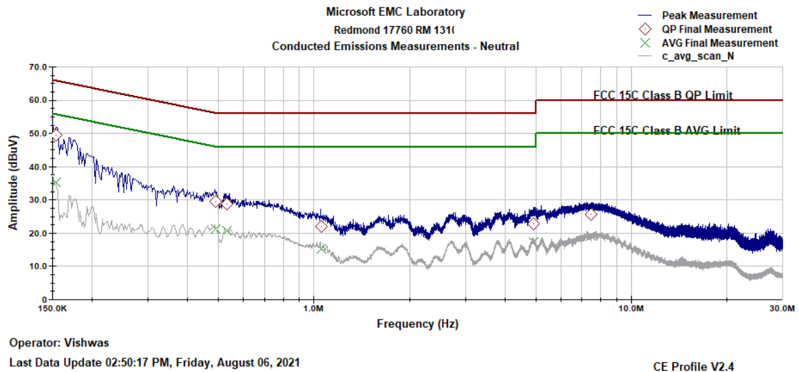
Figure 9-36 AC Line Conducted Emissions- Neutral (150 kHz- 30 MHz)
