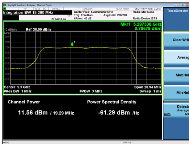
Plot 9-175. Maximum Conducted Output Power and PSD Chain A 802.11a (Ch. 60)
