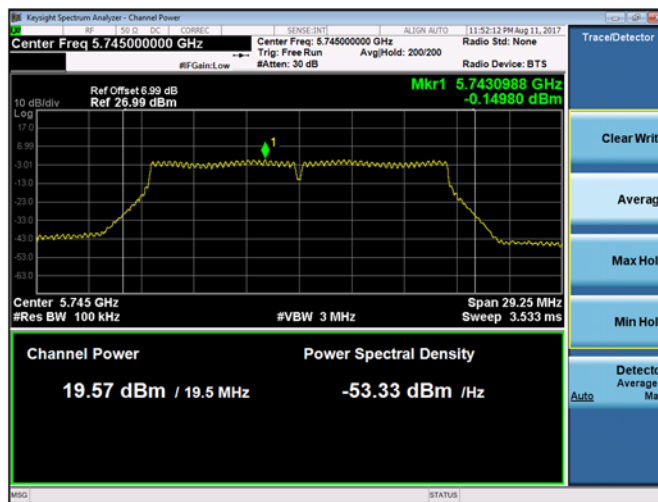
Plot 9-184. Maximum Power Spectral Density Chain A 802.11a (Ch. 149)
