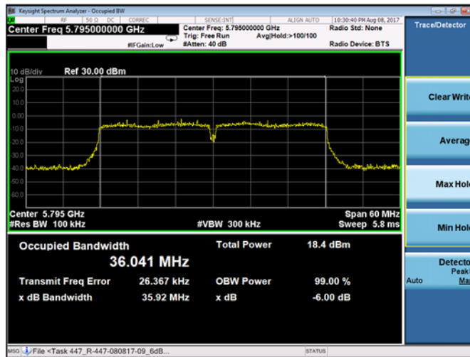
Plot 9-165. 6-dB Bandwidth Chain B 802.11ac VHT40 (Ch. 159)
