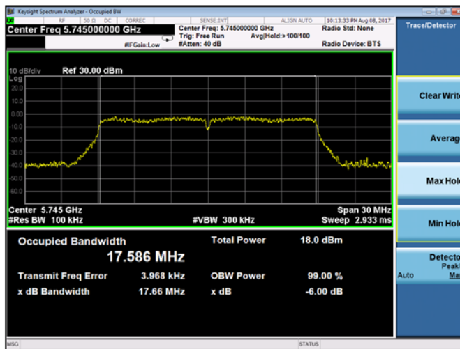
Plot 9-140. 6-dB Bandwidth Chain A 802.11n HT20 (Ch. 149)
