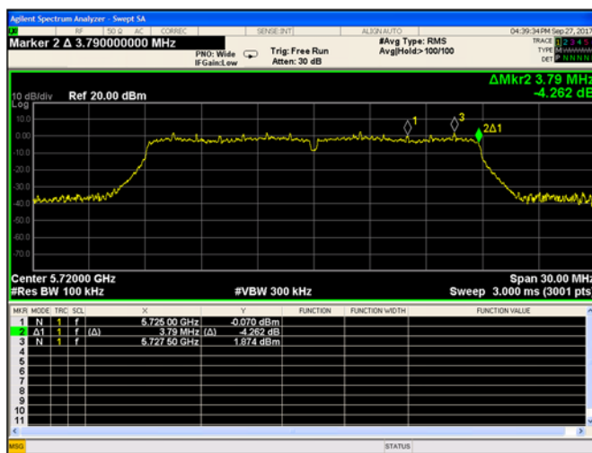
Plot 9-139. 6-dB Bandwidth Chain A 802.11n HT20 (Ch. 144)
