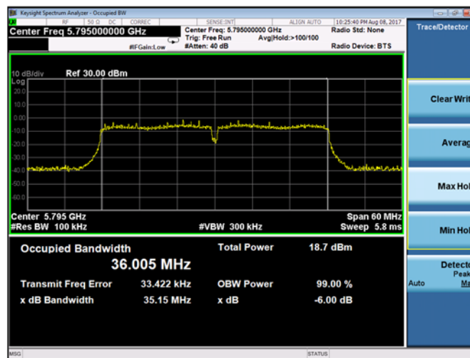
Plot 9-151. 6-dB Bandwidth Chain B 802.11n HT40 (Ch. 159)
