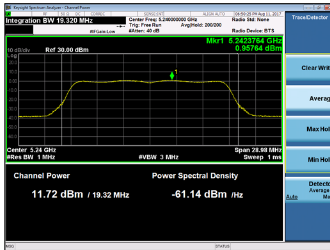
Plot 9-190. Maximum Conducted Output Power and PSD Chain B 802.11a (Ch. 48)
