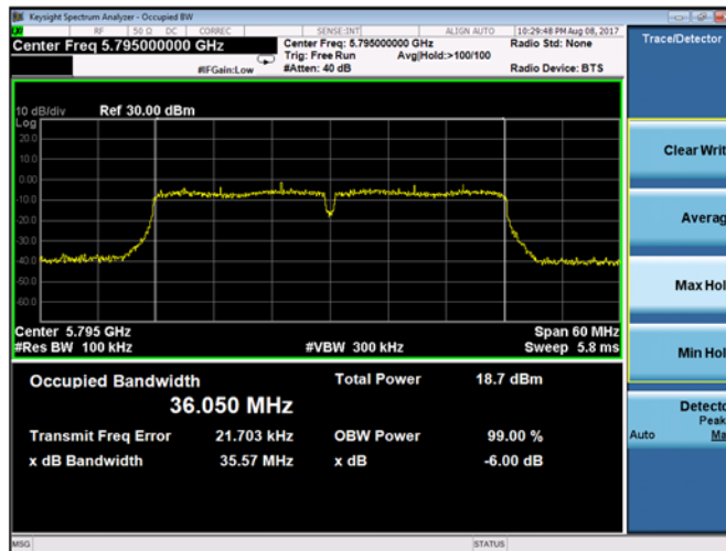
Plot 9-162. 6-dB Bandwidth Chain A 802.11ac VHT40 (Ch. 159)
