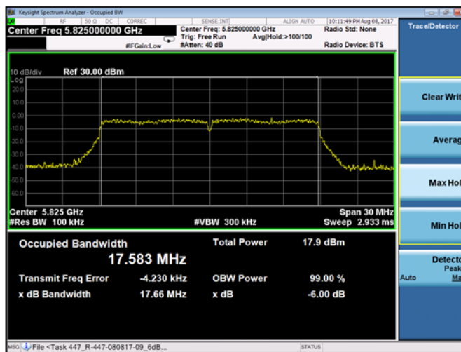
Plot 9-142. 6-dB Bandwidth Chain A 802.11n HT20 (Ch. 165)
