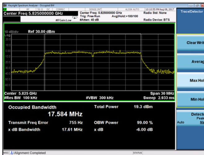
Plot 9-146. 6-dB Bandwidth Chain B 802.11n HT20 (Ch. 165)
