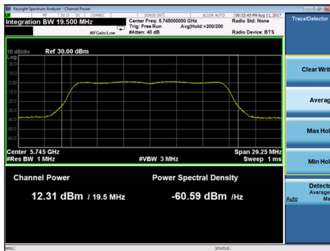
Plot 9-181. Maximum Conducted Output Power Chain A 802.11a (Ch. 149)
