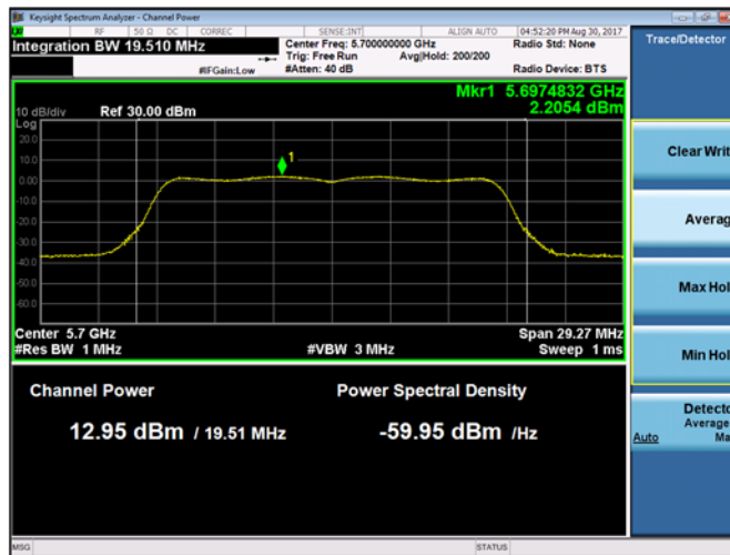
Plot 9-196. Maximum Conducted Output Power and PSD Chain B 802.11a (Ch. 140)
