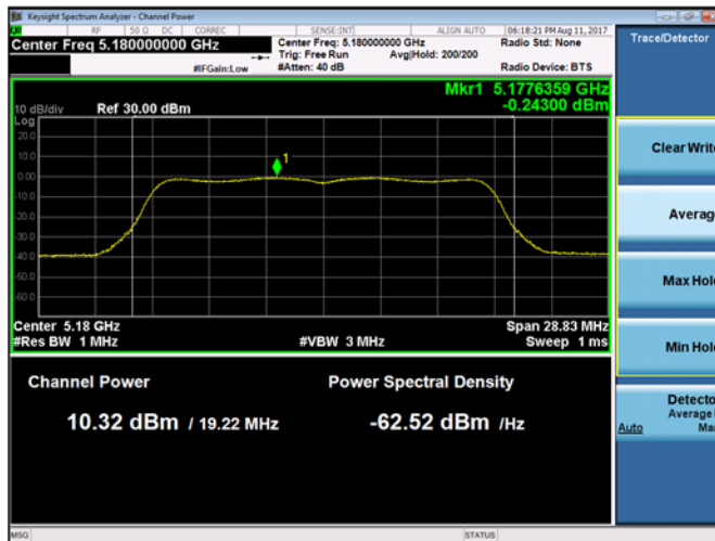
Plot 9-171. Maximum Conducted Output Power and PSD Chain A 802.11a (Ch. 36)
