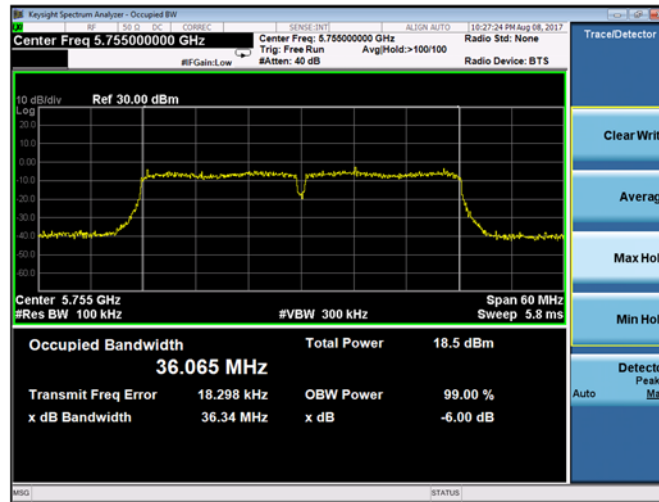
Plot 9-147. 6-dB Bandwidth Chain A 802.11n HT40 (Ch. 151)
