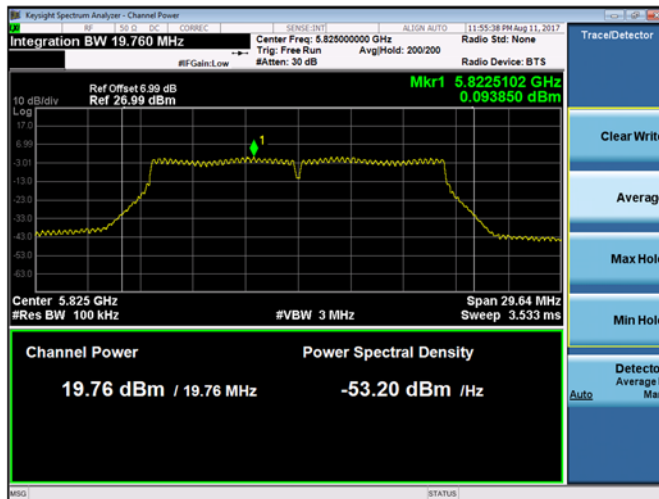
Plot 9-186. Maximum Power Spectral Density Chain A 802.11a (Ch. 165)
