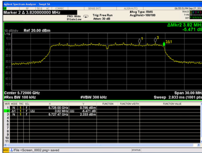
Plot 9-156. 6-dB Bandwidth Chain A 802.11ac VHT20 (Ch. 144)
