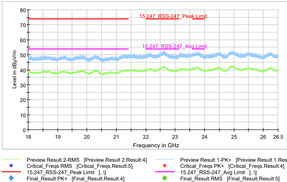
Plot 9-35. Radiated Spurious Emissions (Ch. 0) (18 – 26.5 GHz)
