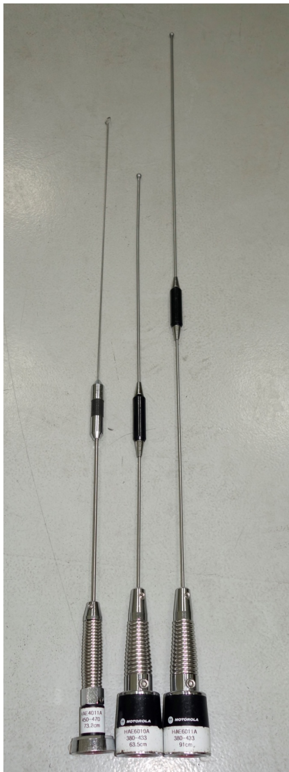
UHF1 Antenna kit numbers, from left to right HAE4011A, HAE6010A, HAE6011A
