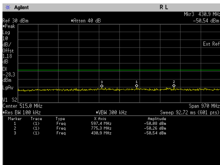
Conducted Emissions. 802.11g, Frequency 2412 MHz Emission Level, 30 MHz -> 1 GHz
