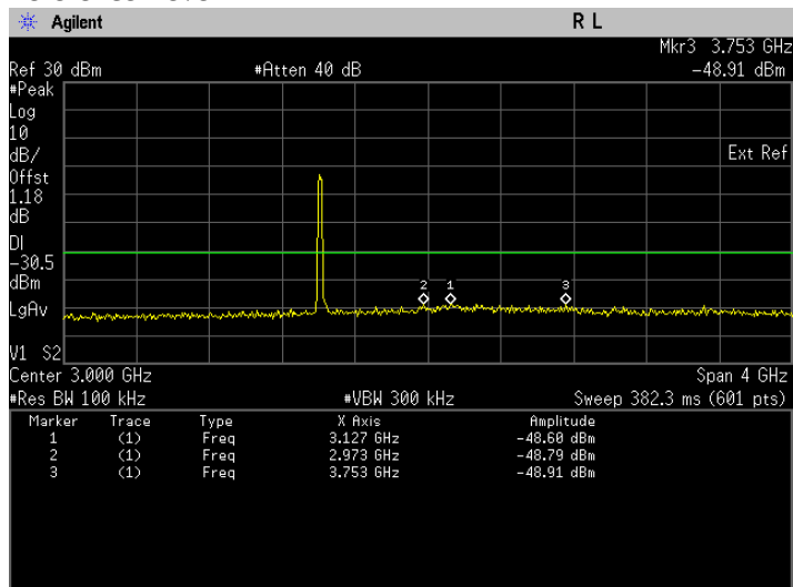
Conducted Emissions. 802.11n, Frequency 2412 MHz Emission Level, 1 GHz -> 5 GHz
