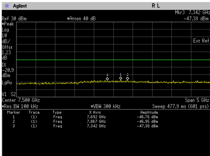
Conducted Emissions. 802.11b, Frequency 2462 MHz Emission Level, 5 GHz -> 10 GHz
