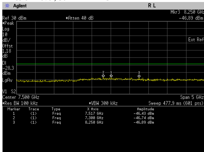
Conducted Emissions. 802.11g, Frequency 2412 MHz Emission Level, 5 GHz -> 10 GHz
