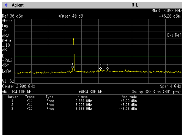
Conducted Emissions. 802.11g, Frequency 2412 MHz Emission Level, 1 GHz -> 5 GHz
