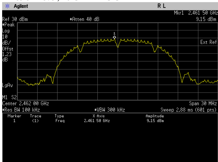
Conducted Emissions. 802.11b, Frequency 2462 MHz Reference Level
