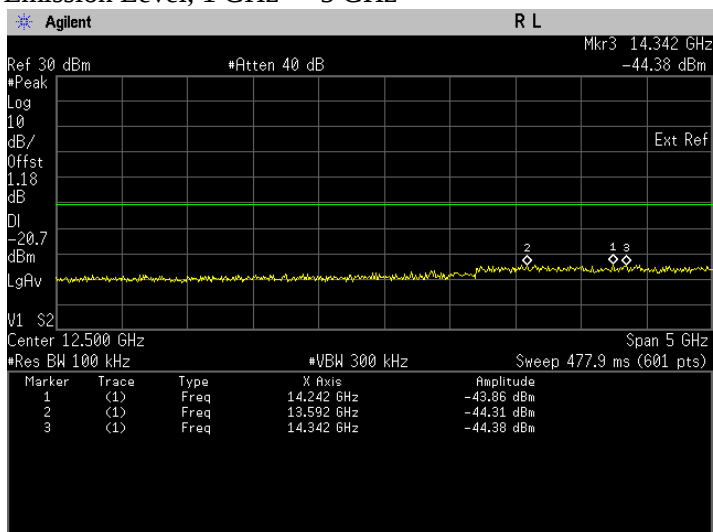
Conducted Emissions. 802.11b, Frequency 2412 MHz Emission Level, 10 GHz -> 15 GHz
