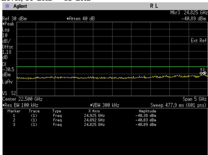
Conducted Emissions. 802.11n, Frequency 2412 MHz Emission Level, 20 GHz -> 25 GHz
