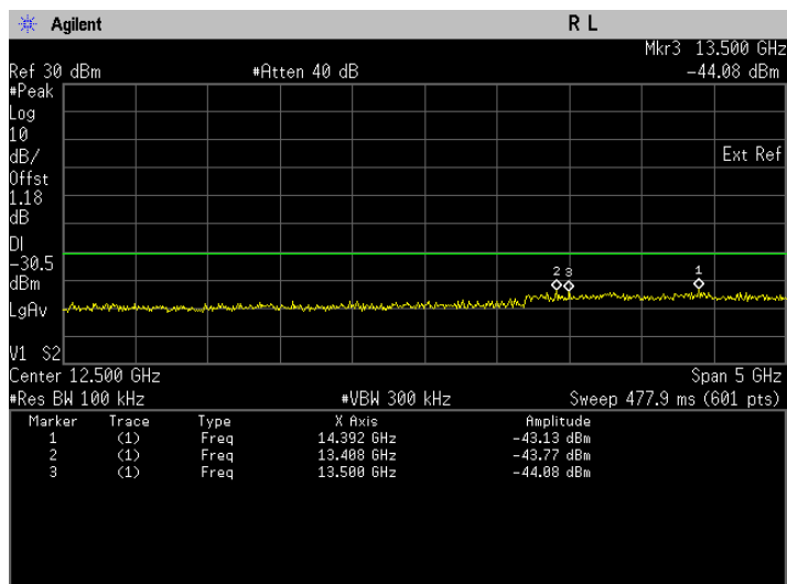
Conducted Emissions. 802.11n, Frequency 2412 Emission Level, 10 GHz -> 15 GHz
