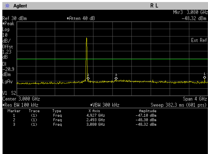
Conducted Emissions. 802.11b, Frequency 2462 MHz Emission Level, 1 GHz -> 5 GHz
