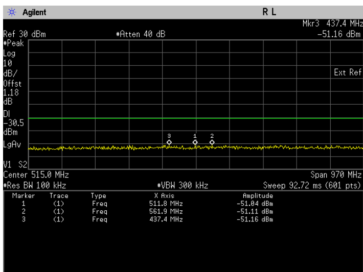
Conducted Emissions. 802.11n, Frequency 2412 MHz Emission Level, 30 MHz -> 1 GHz
