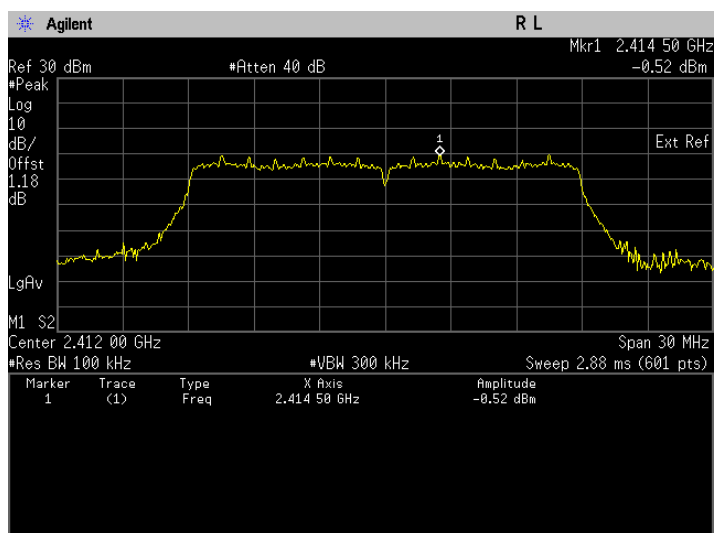
Conducted Emissions. 802.11n, Frequency 2412 MHz Reference Level
