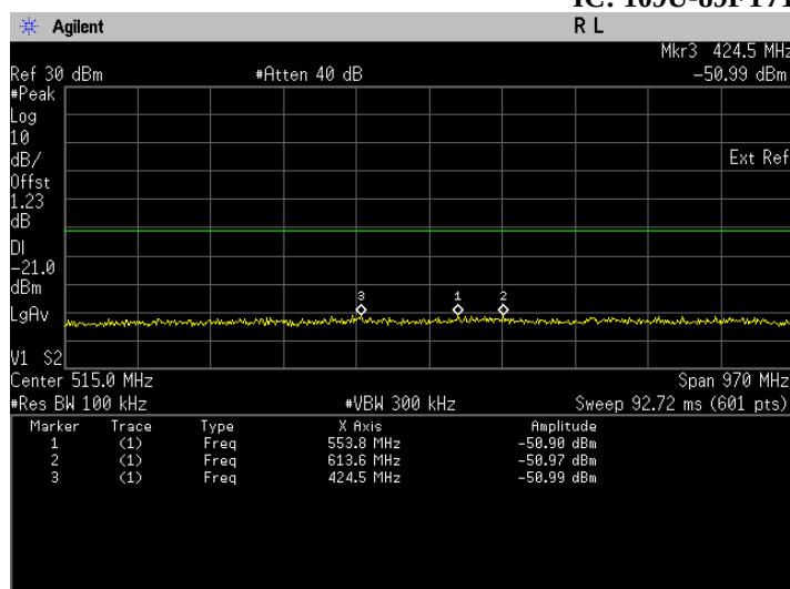
Conducted Emissions. Bluetooth LE, Frequency 2480 MHz Emission Level, 30 MHz -> 1 GHz
