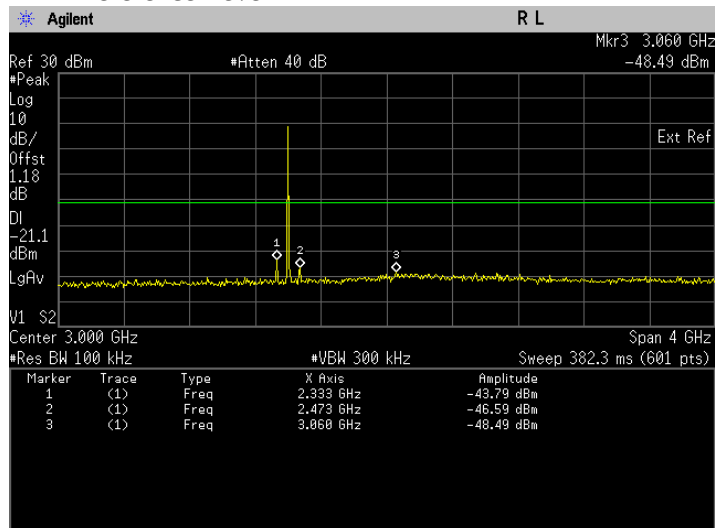
Conducted Emissions. Bluetooth LE, Frequency 2402 MHz Emission Level, 1 GHz -> 5 GHz
