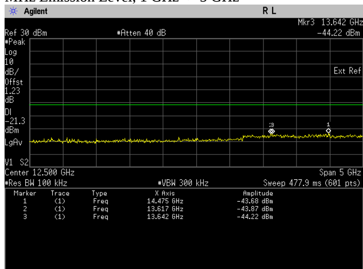
Conducted Emissions. Bluetooth LE, Frequency 2480 MHz Emission Level, 10 GHz -> 15 GHz
