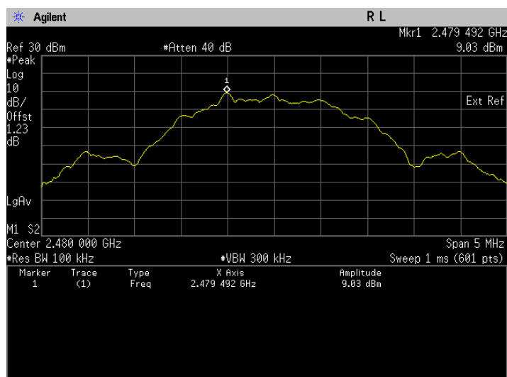
Conducted Emissions. Bluetooth LE, Frequency 2480 MHz Reference Level
