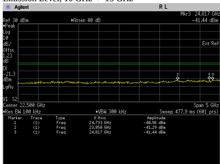
Conducted Emissions. Bluetooth LE, Frequency 2480 MHz Emission Level, 20 GHz -> 25 GHz
