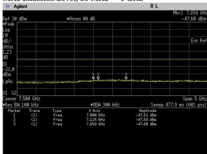
Conducted Emissions. Bluetooth LE, Frequency 2480 MHz Emission Level, 5 GHz -> 10 GHz
