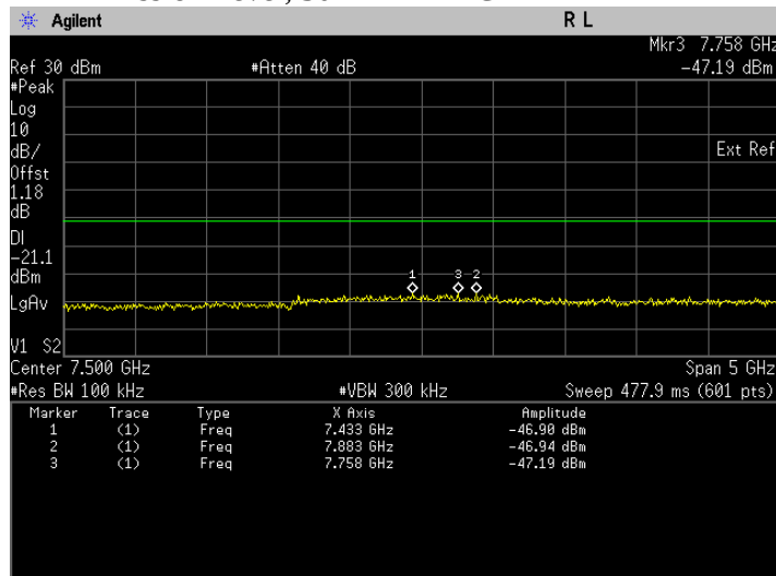
Conducted Emissions. Bluetooth LE, Frequency 2402 MHz Emission Level, 5 GHz -> 10 GHz
