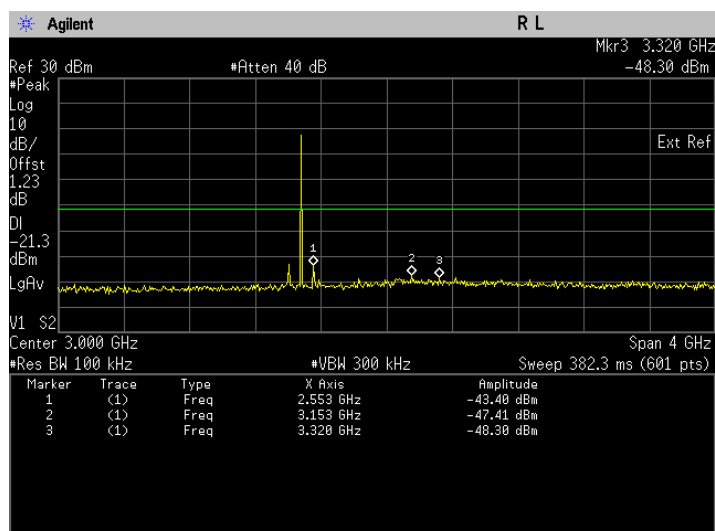
Conducted Emissions. Bluetooth LE, Frequency 2480 MHz Emission Level, 1 GHz -> 5 GHz
