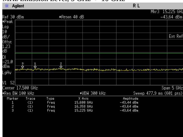
Conducted Emissions. Bluetooth LE, Frequency 2480 MHz Emission Level, 15 GHz -> 20 GHz
