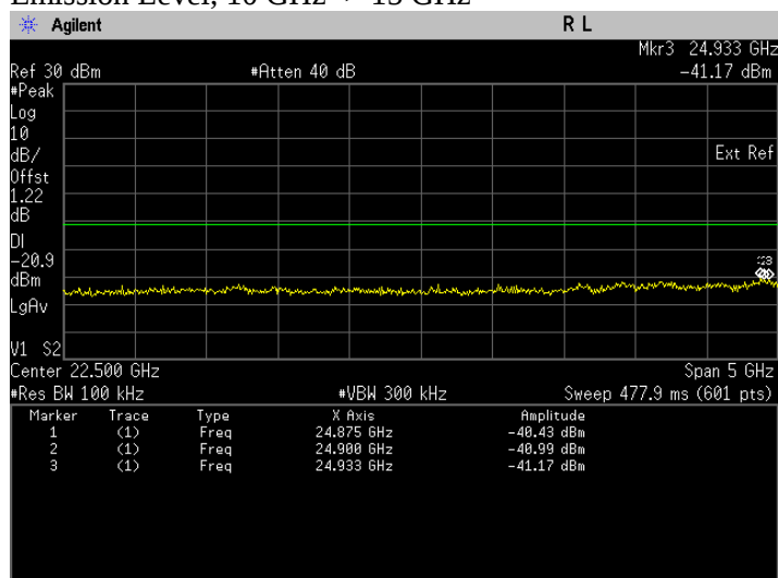
Conducted Emissions. Bluetooth LE, Frequency 2440 MHz Emission Level, 20 GHz -> 25 GHz
