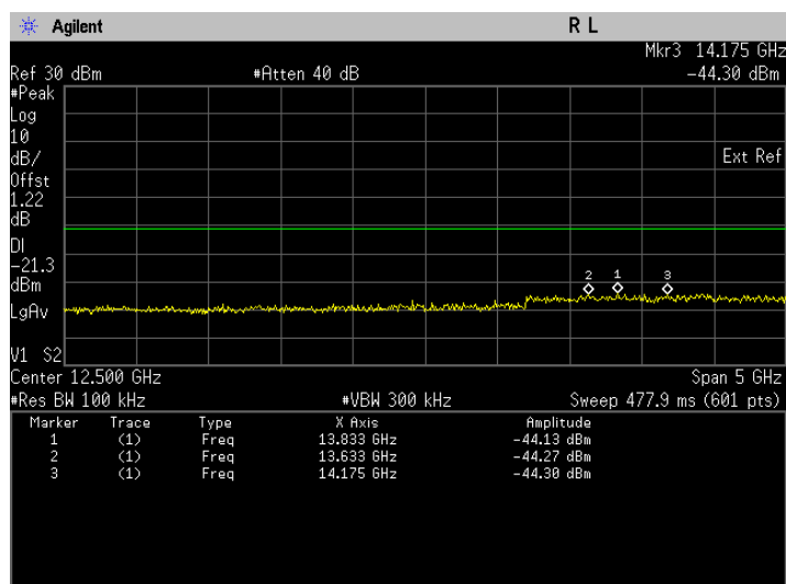
Conducted Emissions. Bluetooth LE, Frequency 2440 Emission Level, 10 GHz -> 15 GHz
