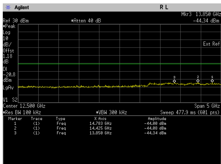
Conducted Emissions. Bluetooth LE, Frequency 2402 Emission Level, 10 GHz -> 15 GHz
