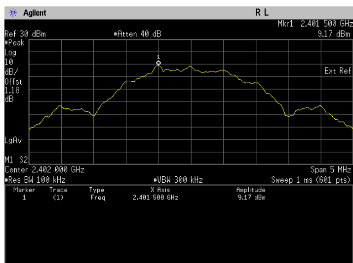
Conducted Emissions. Bluetooth LE, Frequency 2402 MHz Reference Level
