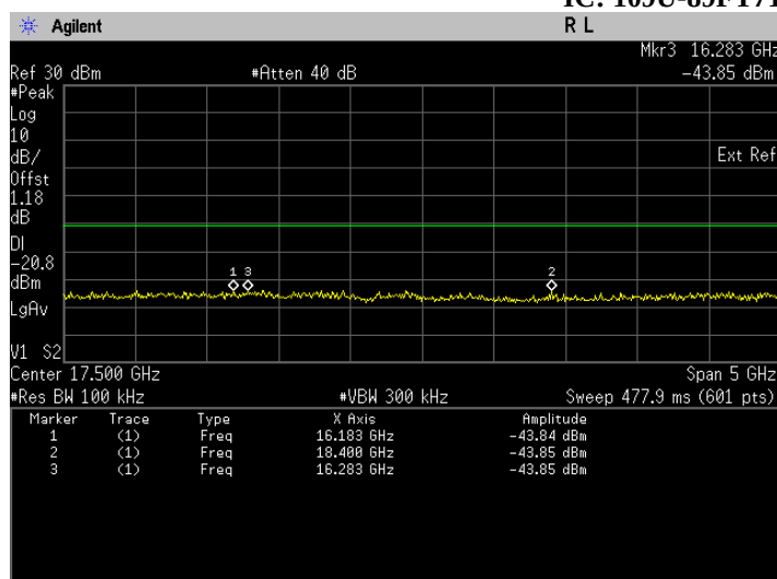
Conducted Emissions. Bluetooth LE, Frequency 2402 MHz Emission Level, 15 GHz -> 20 GHz
