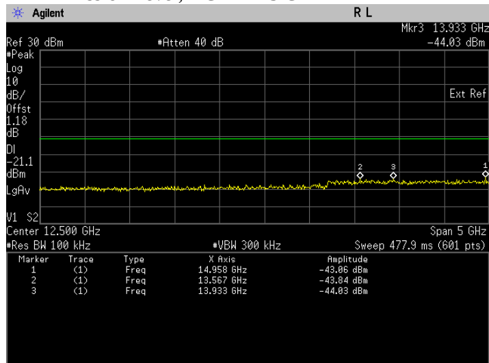
Conducted Emissions. Bluetooth LE, Frequency 2402 MHz Emission Level, 10 GHz -> 15 GHz
