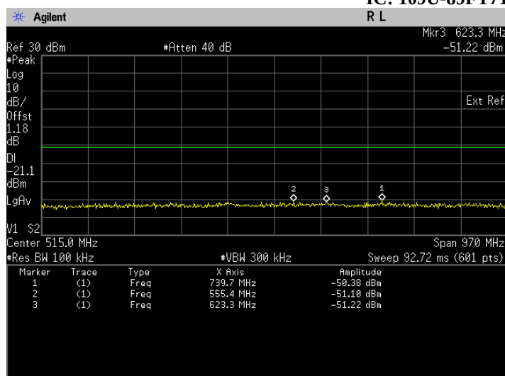
Conducted Emissions. Bluetooth LE, Frequency 2402 MHz Emission Level, 30 MHz -> 1 GHz
