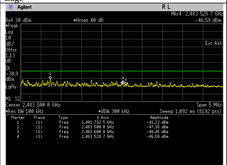
Band Edge(Average). 802.11g Frequency 2462 MHz Band Edge
