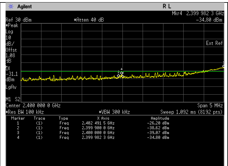
Band Edge(Average). 802.11g Frequency 2412 MHz Band Edge
