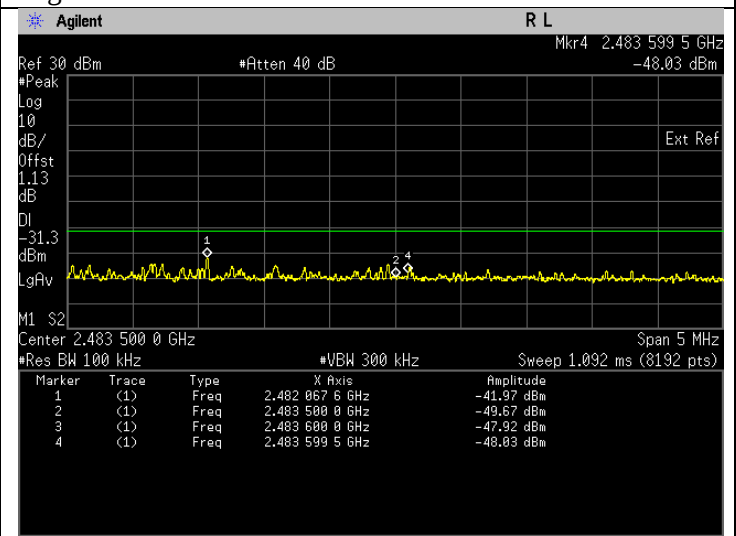
Band Edge(Average). 802.11n Frequency 2462 MHz Band Edge
