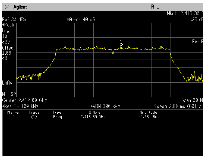
Conducted Emissions(Average). 802.11n, Frequency 2412 MHz Reference Level
