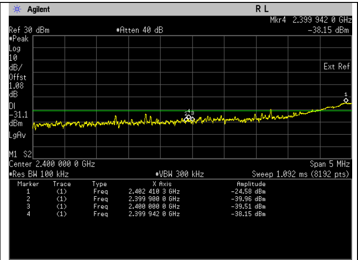
Band Edge(Average). 802.11n Frequency 2412 MHz Band Edge
