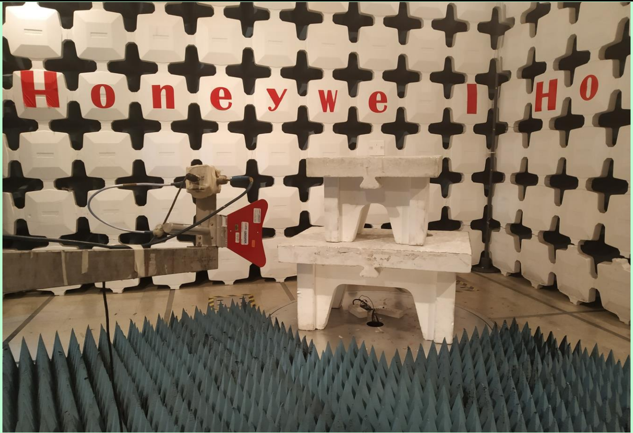
Radiated Emission Setup –1 GHz to 10 GHz [Horizontal Polarization]
