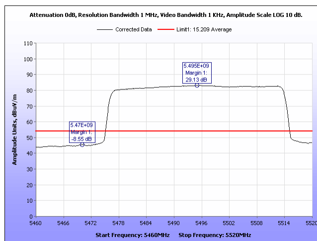
Plot 537. Radiated Band Edge, Average 8 Omni, 40M, 5495, Port 1
