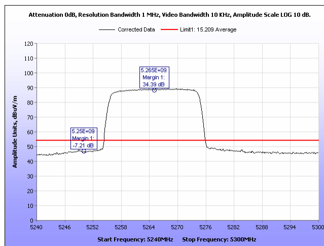
Plot 675. Radiated Band Edge, Average 90 Sector, 20MHz, 5265MHz, Port 1
