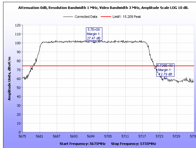
Plot 878. Radiated Band Edge, Peak 2 Panel, 40MHz, 5700MHz, Port 1
