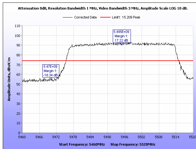
Plot 562. Radiated Band Edge, Peak 8 Omni, 40M, 5495, Port 2
