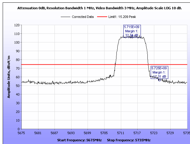
Plot 714. Radiated Band Edge, Peak 90 Sector, 10MHz, 5715MHz, Port 2
