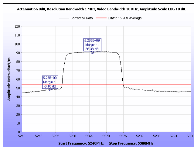
Plot 833. Radiated Band Edge, Average 2 Panel, 20MHz, 5265MHz, Port 2
