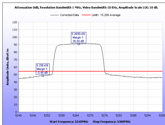
Plot 832. Radiated Band Edge, Average 2 Panel, 20MHz, 5265MHz, Port 1
