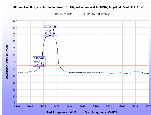
Plot 840. Radiated Band Edge, Average 2 Panel, 5MHz, 5475MHz, Port 1
