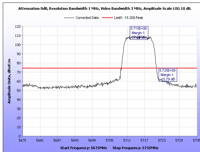
Plot 871. Radiated Band Edge, Peak 2 Panel, 10MHz, 5715MHz, Port 2
