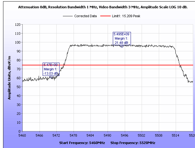
Plot 877. Radiated Band Edge, Peak 2 Panel, 40MHz, 5495MHz, Port 2
