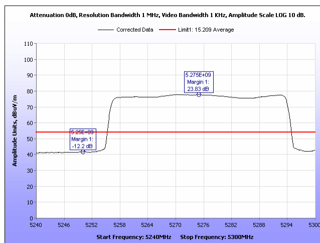
Plot 522. Radiated Band Edge, Average 8 Omni, 40M, 5275, Port 2
