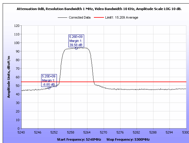
Plot 828. Radiated Band Edge, Average 2 Panel, 10MHz, 5260MHz, Port 1
