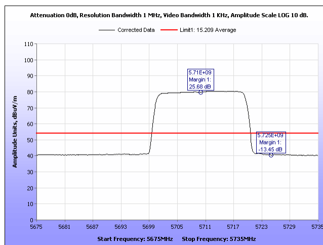
Plot 536. Radiated Band Edge, Average 8 Omni, 20M, 5710, Port 2
