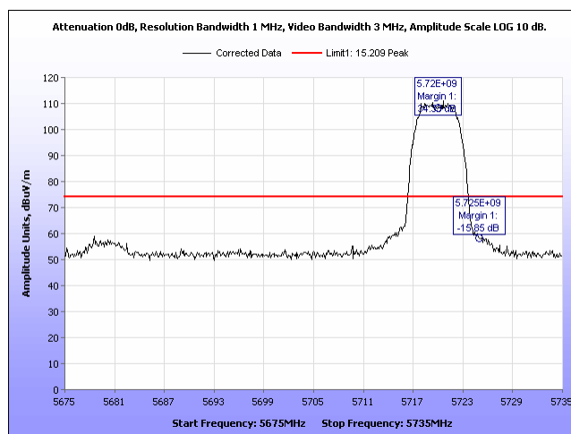
Plot 710 Radiated Band Edge, Peak 90 Sector, 5MHz, 5720MHz, Port 2
