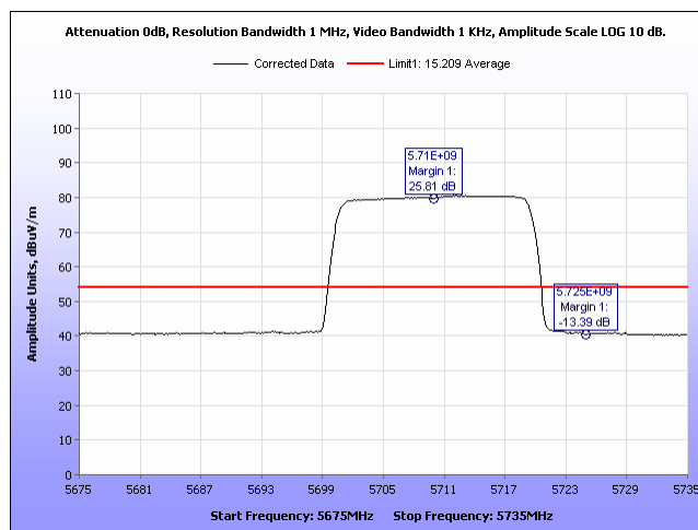
Plot 535. Radiated Band Edge, Average 8 Omni, 20M, 5710, Port 1
