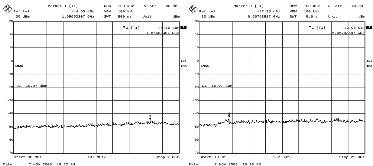
Plot 4-6. Out of band emissions around 2462MHz (OFDM, 18Mbps)
