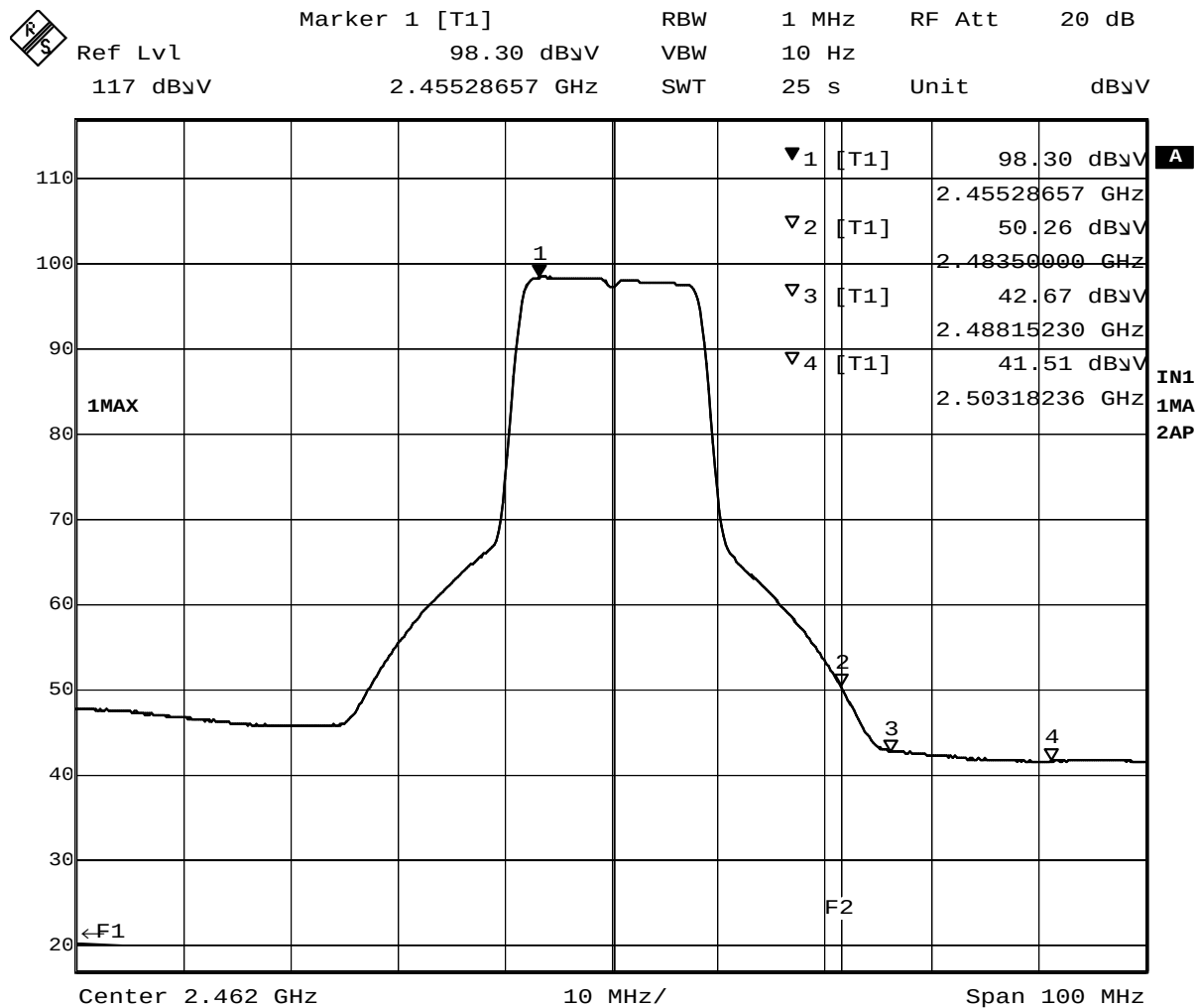
Plot 8-8 Ch.11 2462MHz TX, OFDM 18Mbps (Average)
