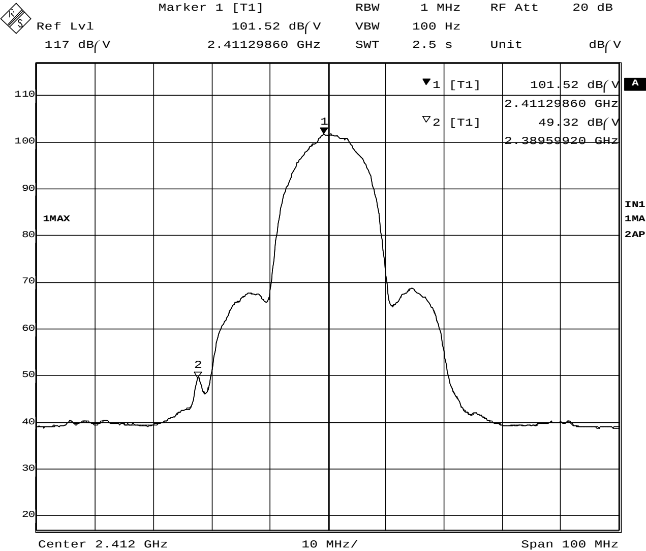
Plot 7-2-2 Ch.1 2412MHz TX11Mb/s (Average)
