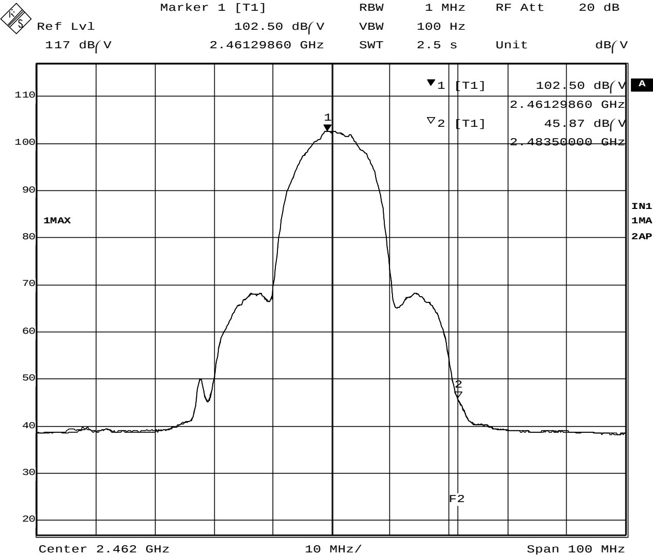
Plot 7-2-4 Ch.11 2462MHz TX 11Mb/s (Average)
