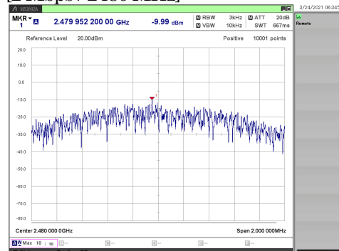
[2 Mbps / 2480 MHz]
