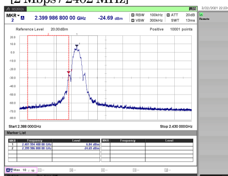
[2 Mbps / 2402 MHz]
