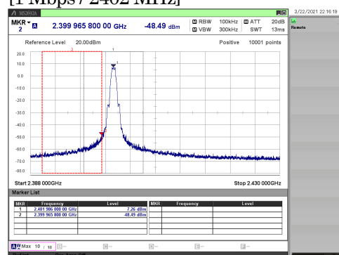
[1 Mbps / 2402 MHz]
