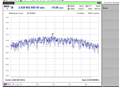
[2 Mbps / 2440 MHz]
