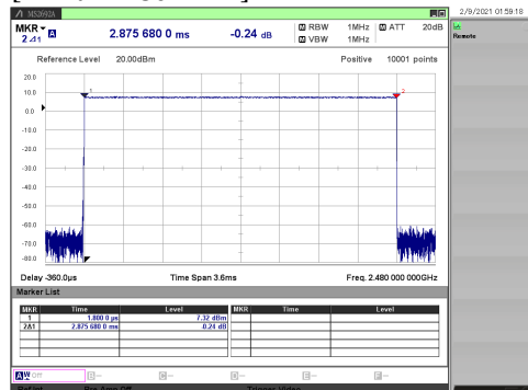
[BDR / 2480 MHz]
