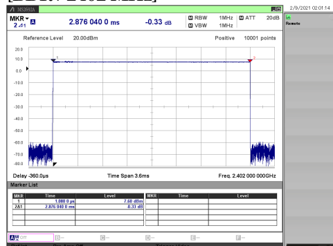
[BDR / 2402 MHz]
