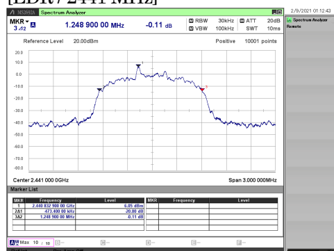
[EDR / 2441 MHz]
