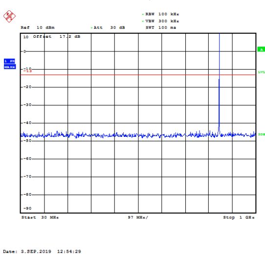
GSM 850 CH-High 30MHz ~ 1GHz
