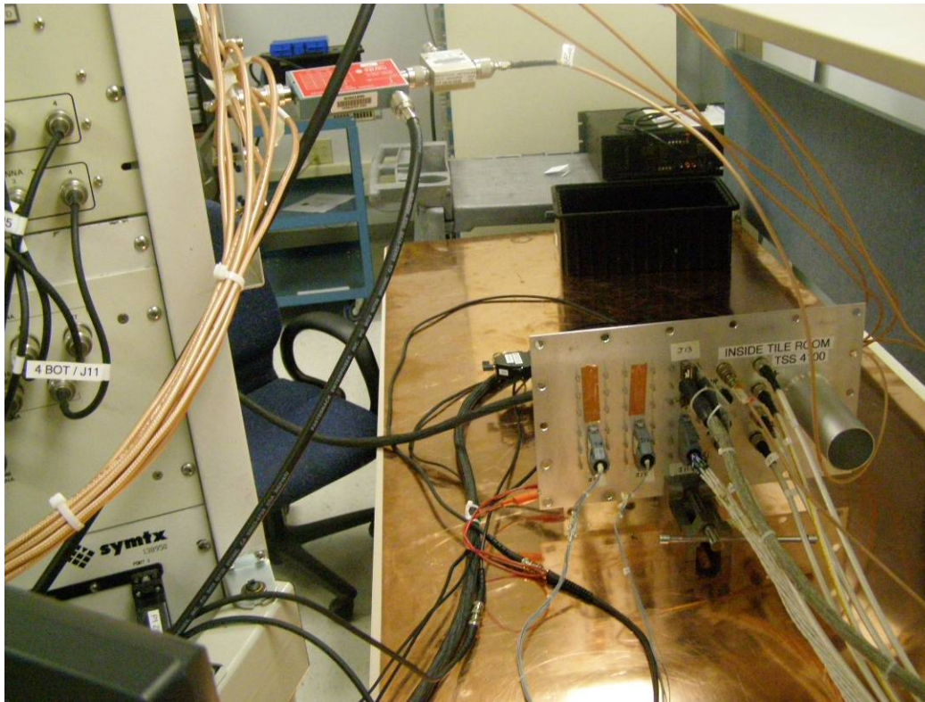
Figure 4. Power Input EMI Harness
