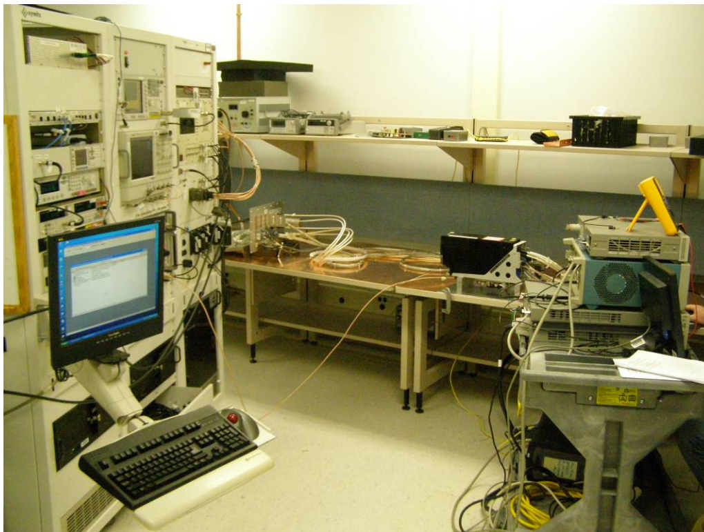
Figure 3. Power Input Overall Setup
