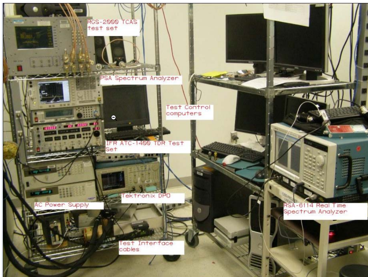
Figure 1. Production Interim Test Station Setup
