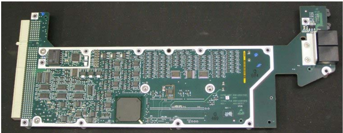
Figure 13 – System I/O Circuit Card CPN 828-1930-002 Top View
