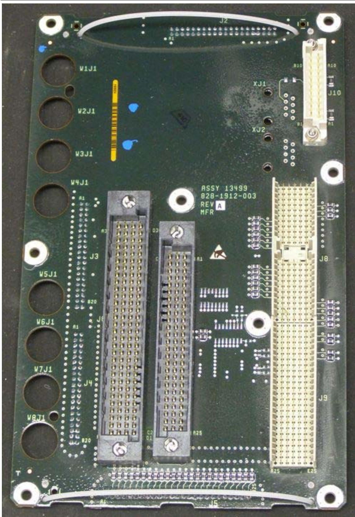
Figure 1 – Backplane Circuit Card CPN 828-1912-003 Top Side
