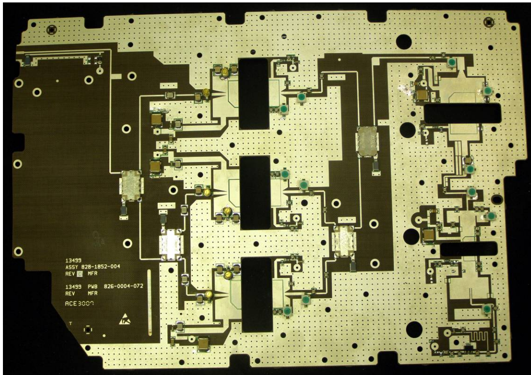
Figure 19 – Linear PA PWB CPN 828-1852-004 Top View (Power devices not populated)
