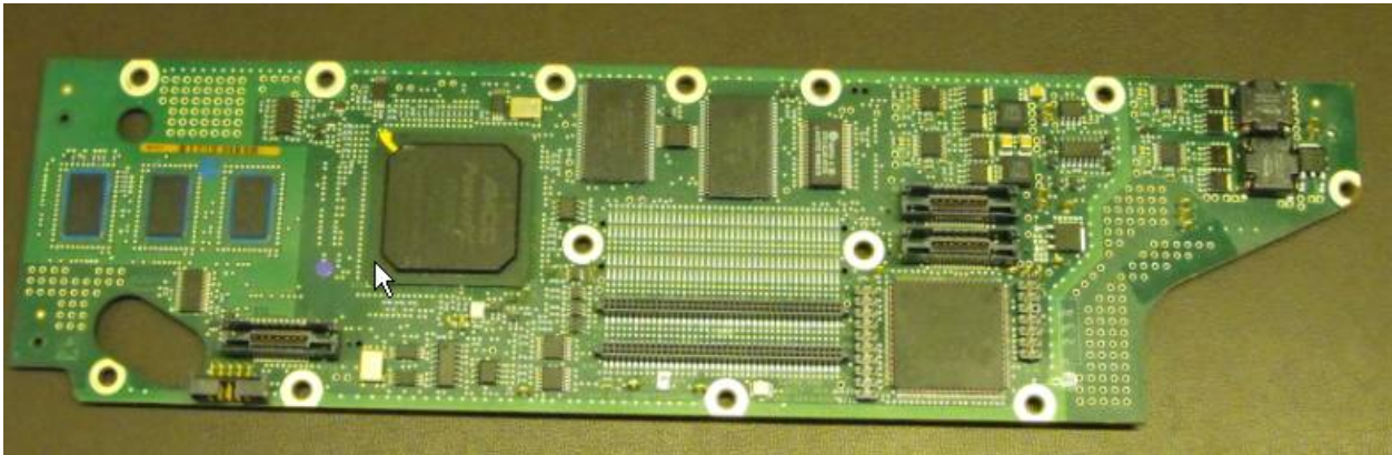
Figure 15 - System Processor Circuit Card CPN 828-1931-002 Top View
