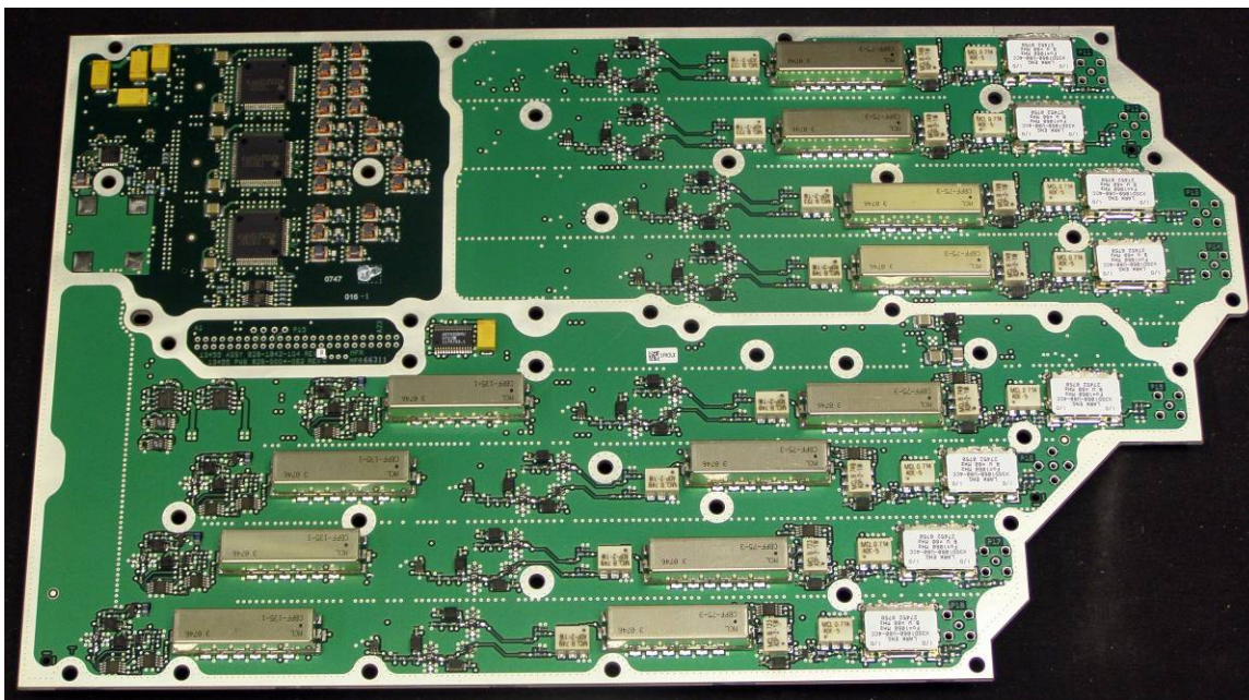
Figure 23 – Receiver PWB CPN 828-1842-104 Top View
