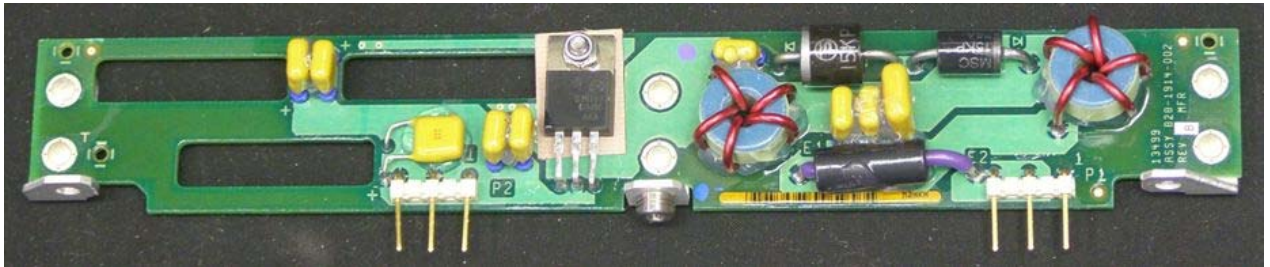
Figure 5 – Power Filter PWB CPN 828-1914-002 Top Side
