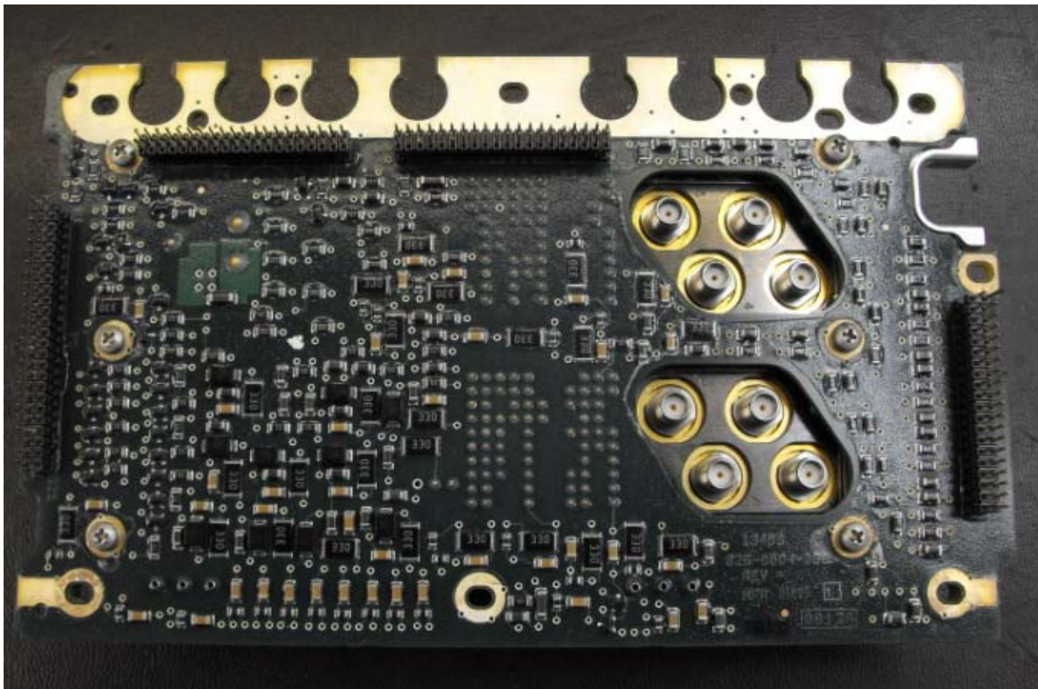
Figure 4 – Rear Interconnect Filter PWB Bottom Side
