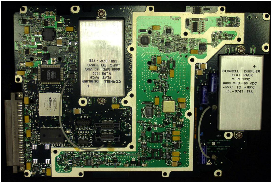
Figure 17 – Modulator PWB CPN 828-1851-005 Top View
