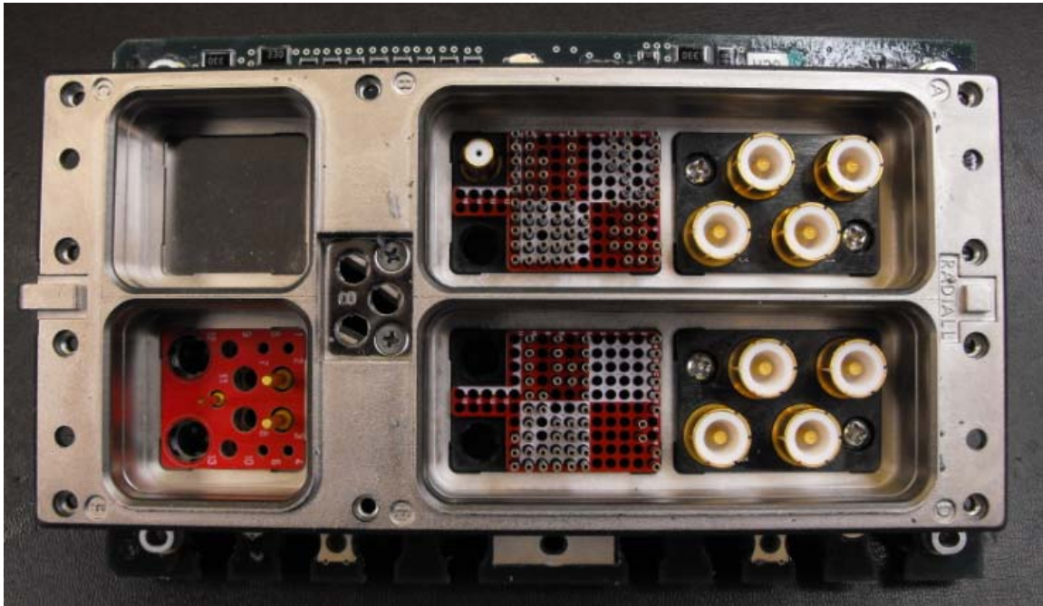
Figure 3 – Rear Interconnect Filter PWB CPN 828-1911-002 Top Side
