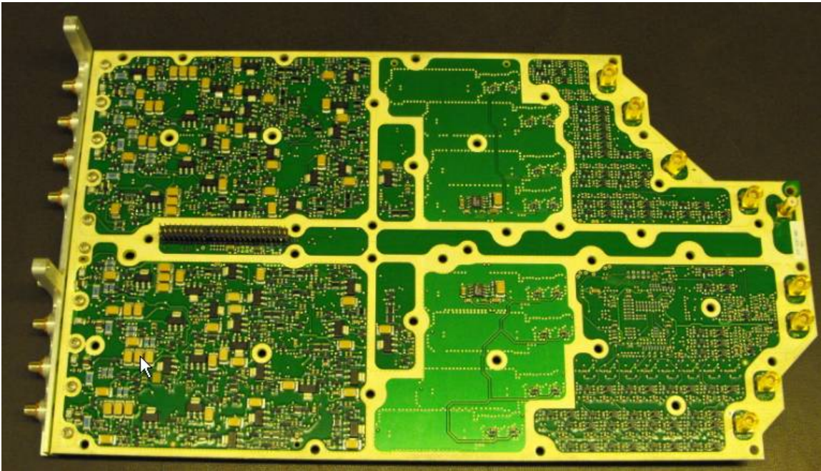
Figure 26 – RF Switch PWB Bottom View
