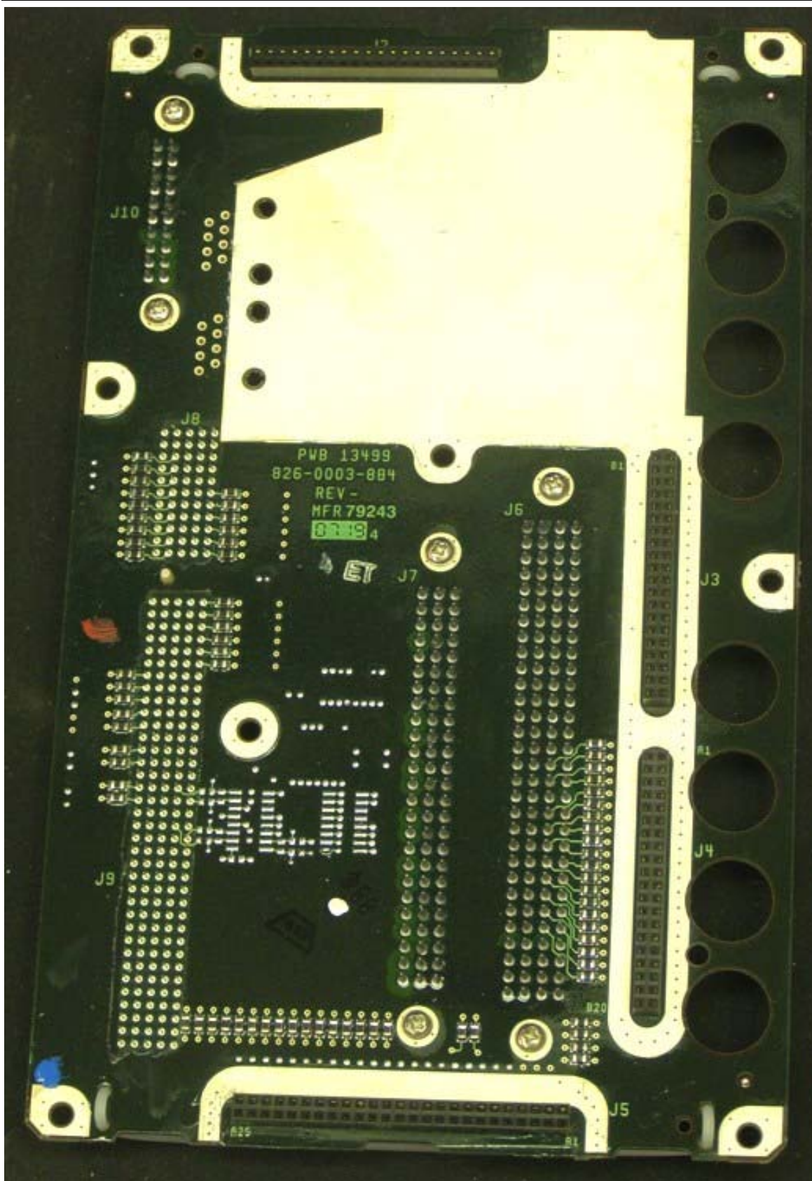
Figure 2 – Backplane Circuit Card Bottom Side
