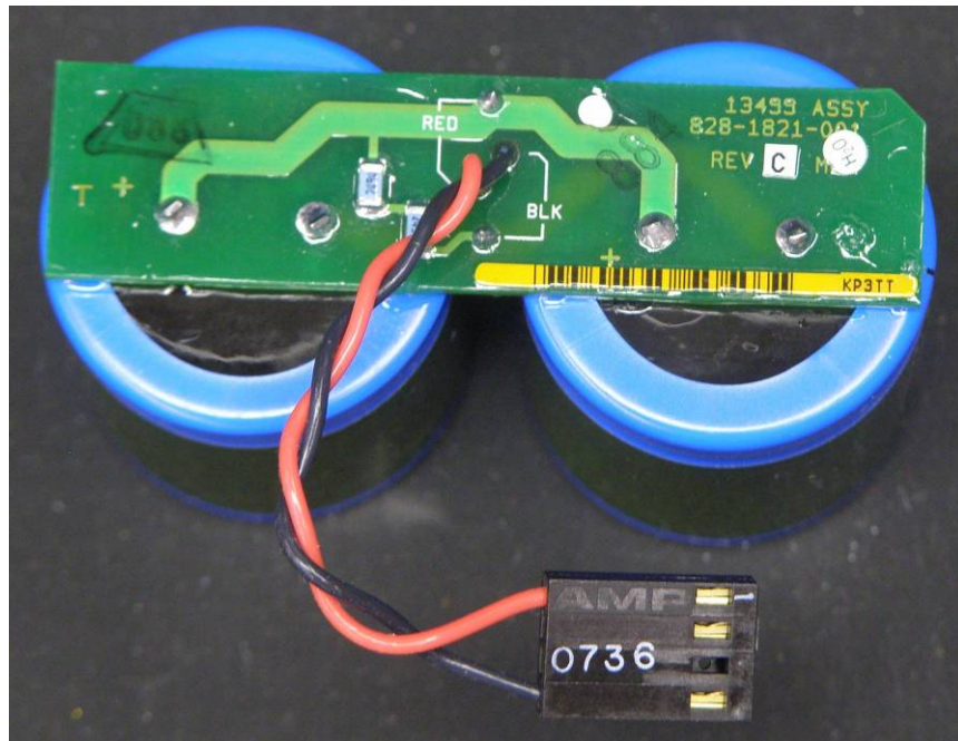
Figure 11 – Power Storage Assembly CPN 828-1821-001
