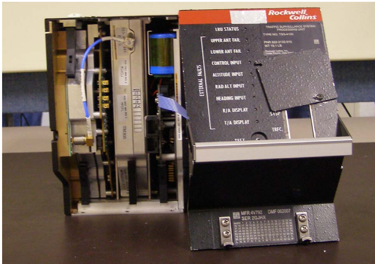
Figure 6 - Front View, Face Plate Removed
