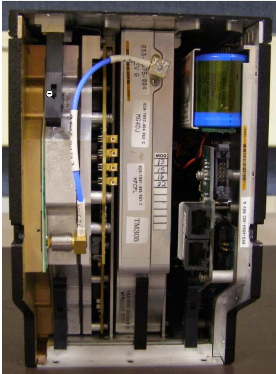
Figure 7 - Front View Assembly Detail
