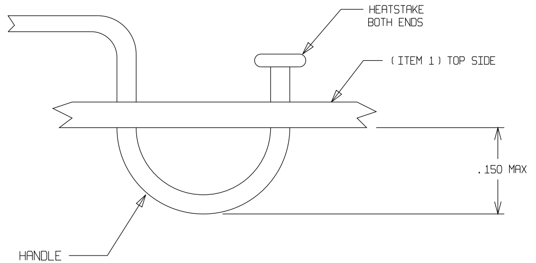
DETAIL J 2 PLACES
