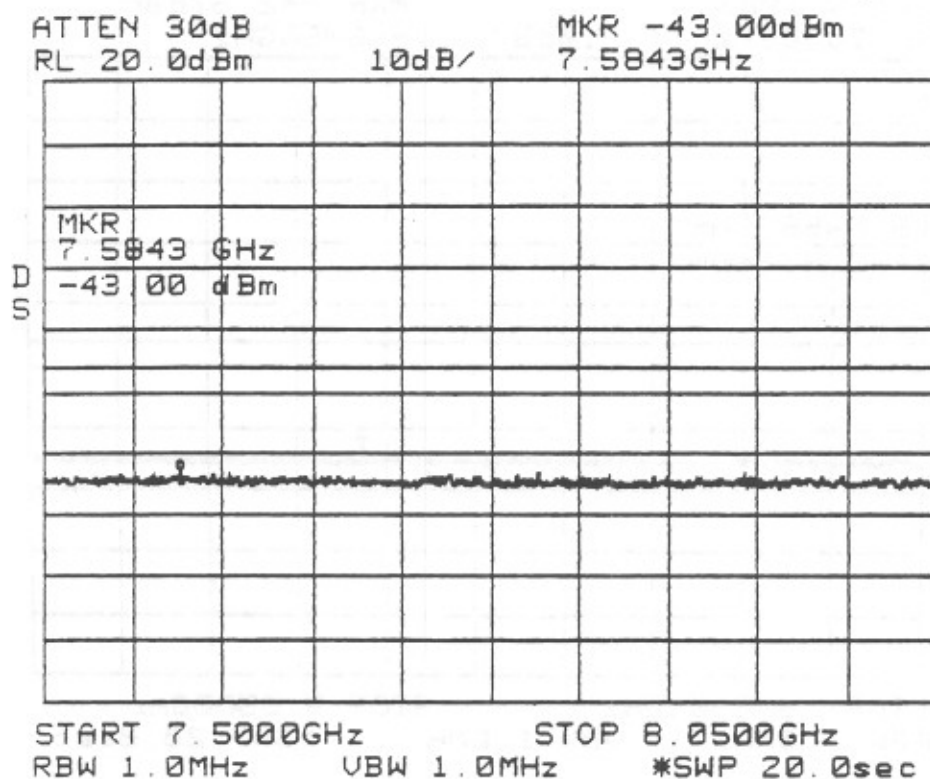
Figure 3-30 Spurious Emissions At The Antenna Port, 7,500 to 8,050 MHz
