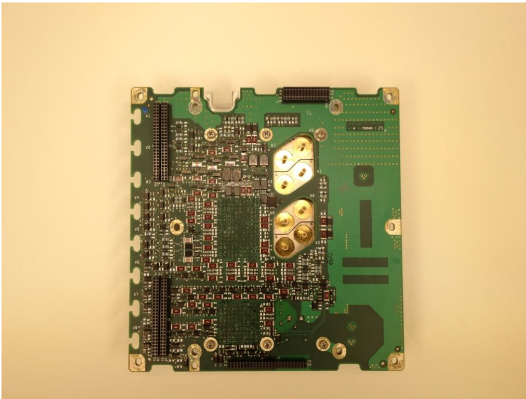
Figure I-12 – TTR-2100 Filter Assembly – Bottom
