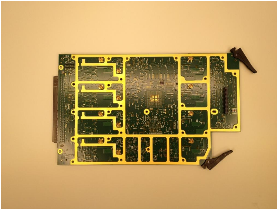
Figure I-3 – TTR-2100 Transceiver Assembly – Bottom
