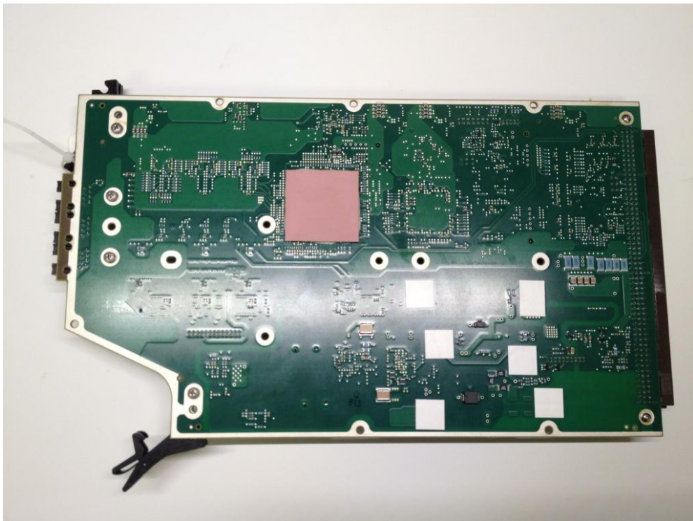
Figure I-9 – TTR-2100 DSP/Power Supply Assembly – Bottom
