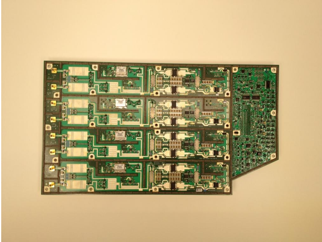
Figure I-4 – TTR-2100 Power Amplifier Assembly – Top
