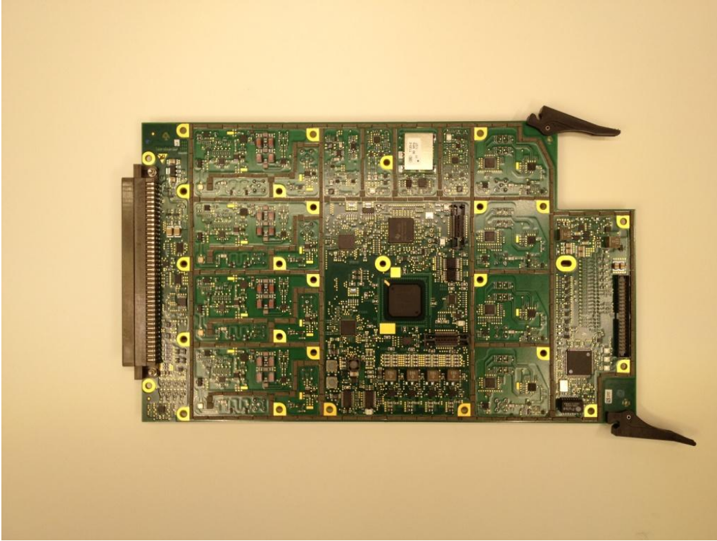
Figure I-2 – TTR-2100 Transceiver Assembly – Top
