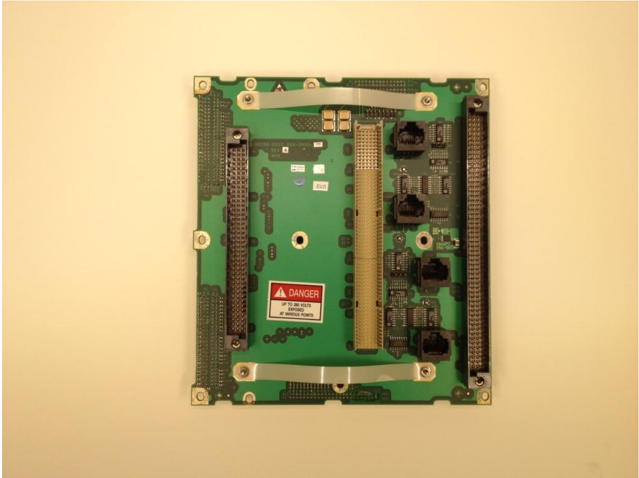
Figure I-10 – TTR-2100 Backplane Assembly – Top
