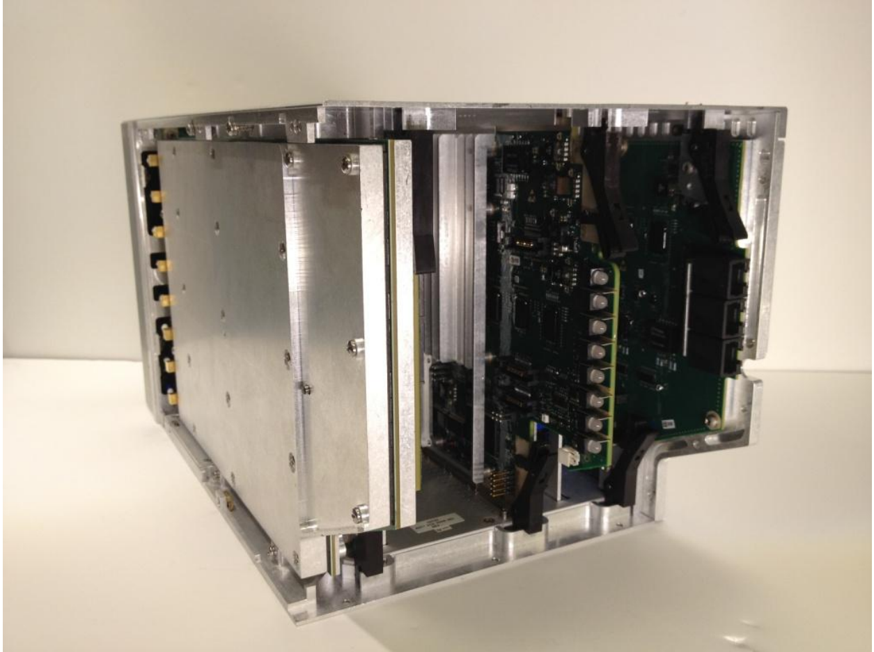
Figure I-1 – TTR-2100 Top Level Chassis
