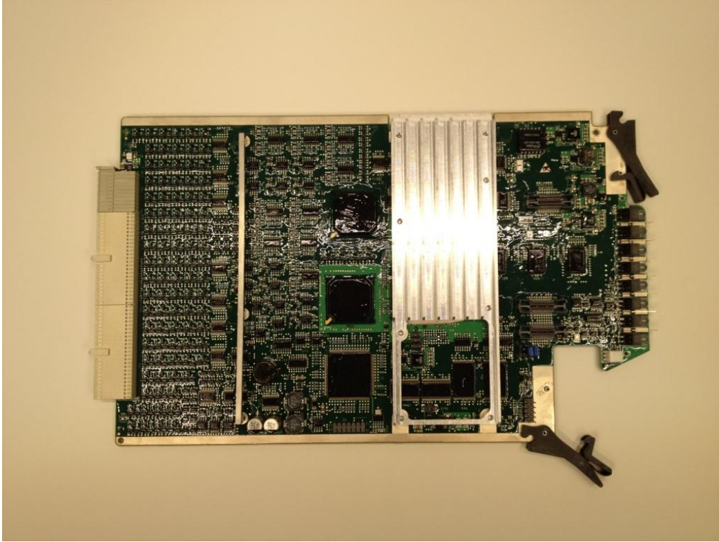
Figure I-6 – TTR-2100 System I/O Processor Assembly – Top
