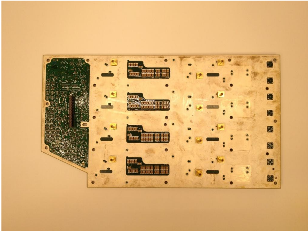
Figure I-5 – TTR-2100 Power Amplifier Assembly – Bottom
