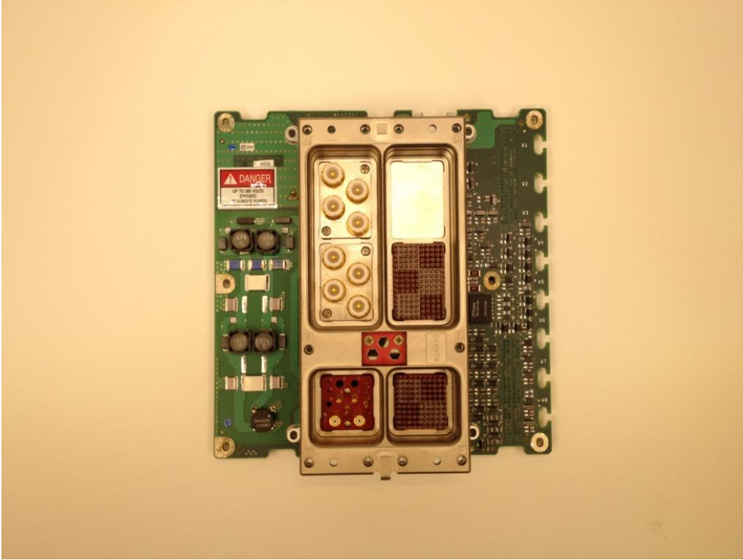
Figure I-11 – TTR-2100 Filter Assembly – Top
