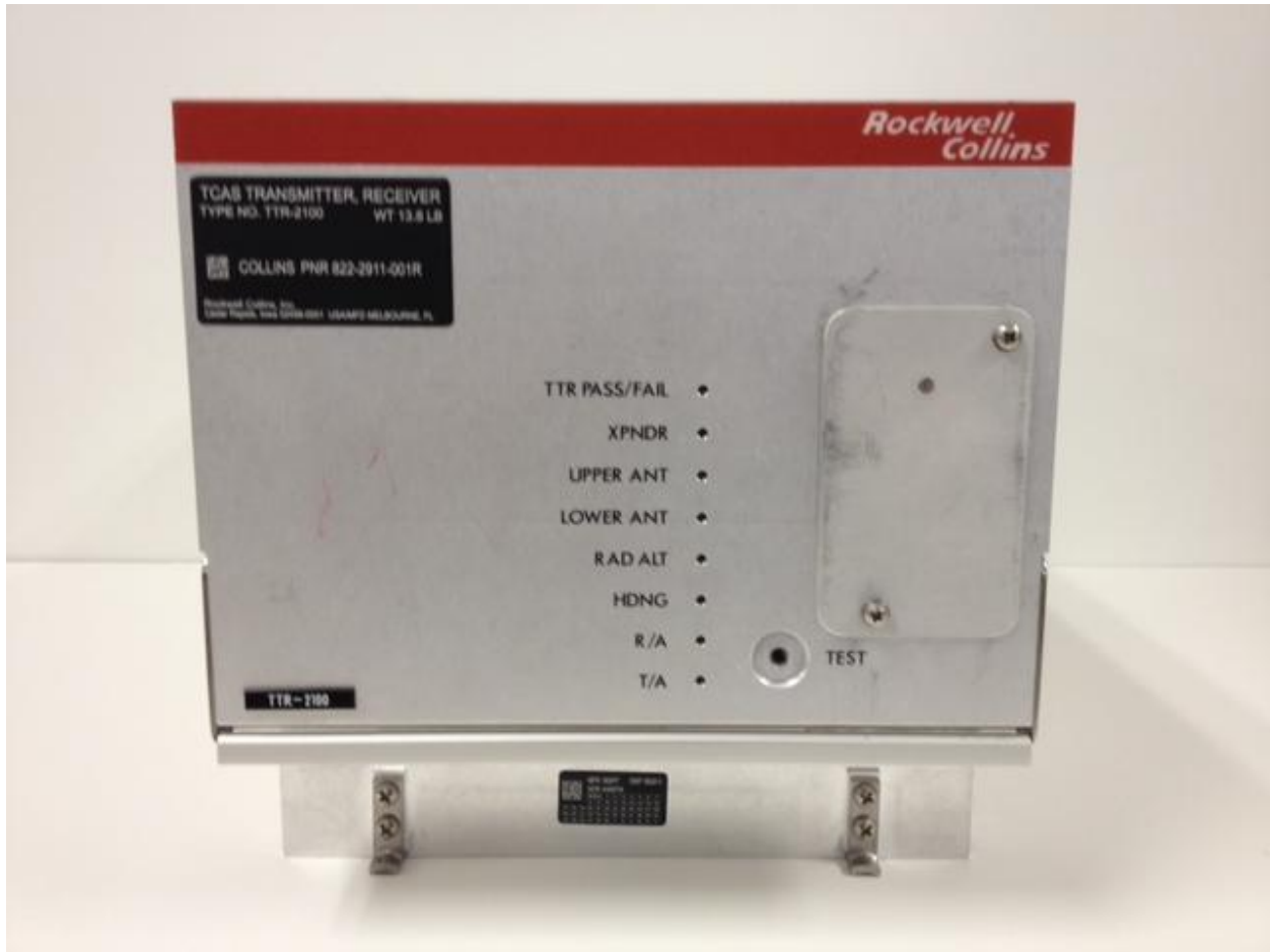
Figure C-1 – TTR-2100 External Photograph – Front
