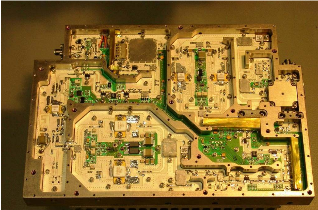
Figure 5 Top View of RF Module main board assembly
