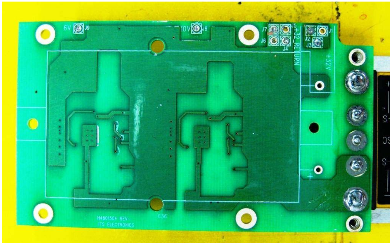
Figure 26 Bottom View of Vicor Output board
