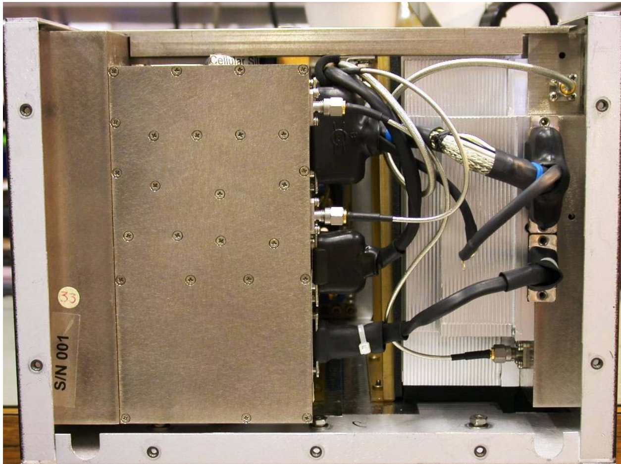
Figure 2 Integrated HPA Front View with Top and Front Panels removed
