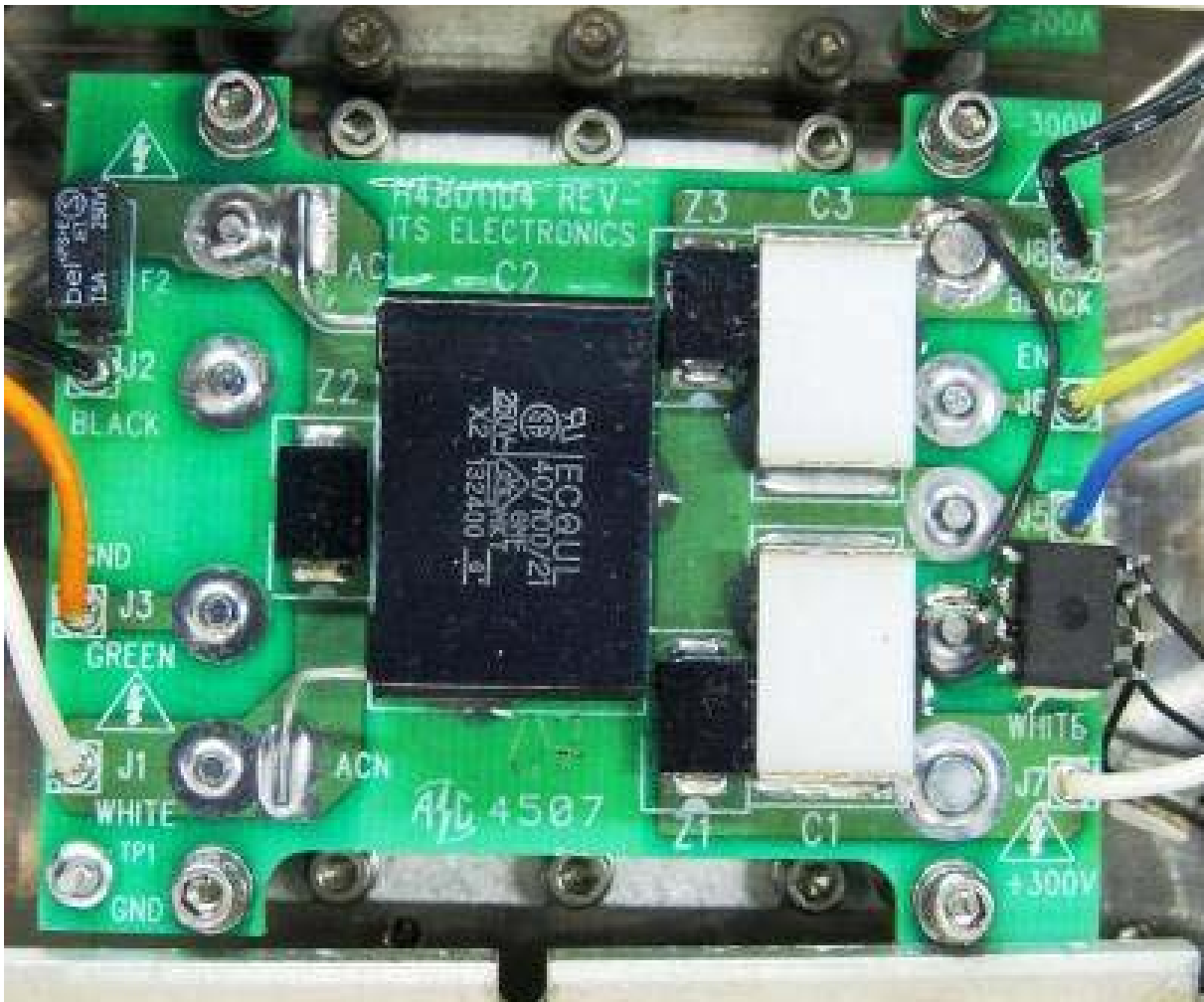
Figure 19 Top view of filter board
