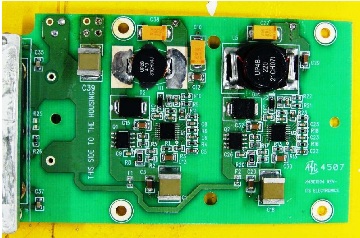
Figure 25 Top View of Vicor Output board
