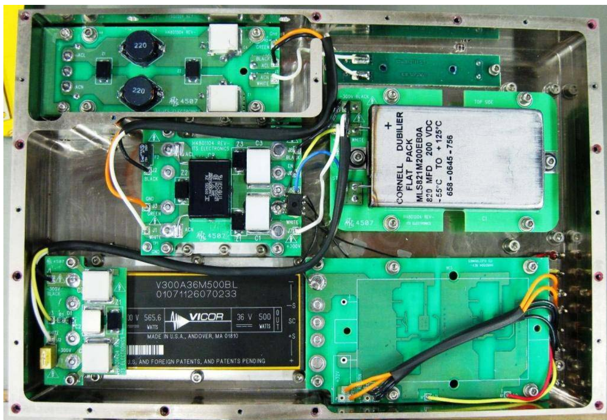
Figure 16 Top view of power supply subassembly
