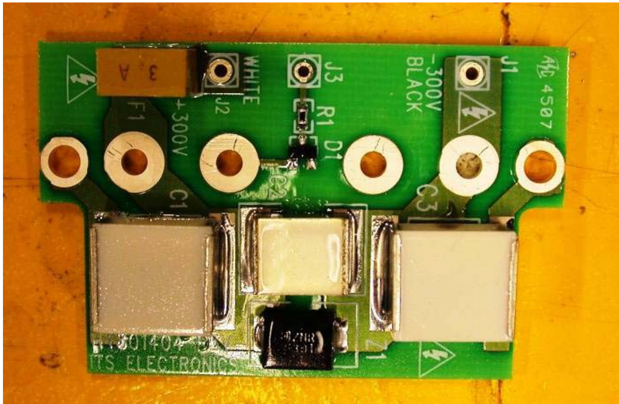
Figure 23 Top view of Vicor input board
