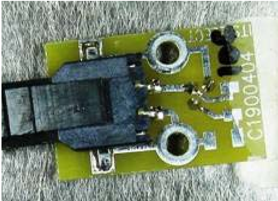
Figure 11 Bottom view of temperature sensor board
