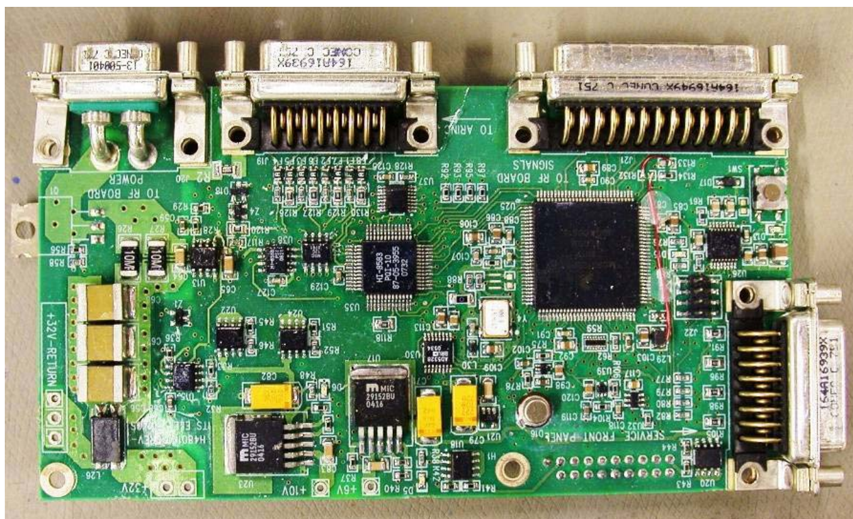
Figure 14 Top view of controller board
