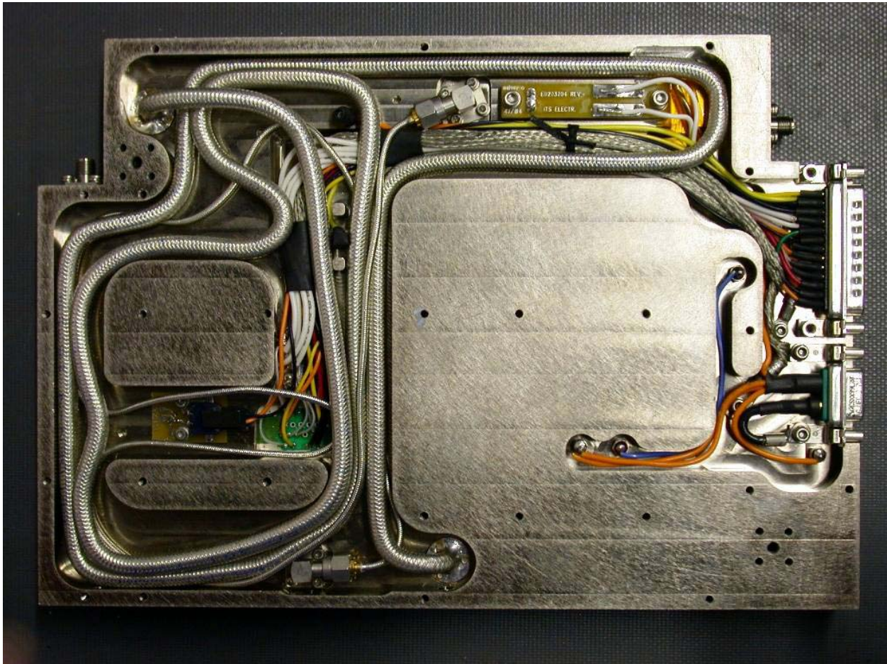
Figure 7 Bottom view of RF module assembly with heatsink removed
