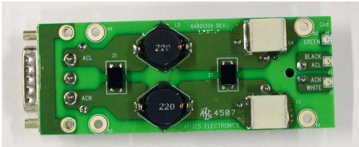
Figure 17 Top view of input AC filter board
