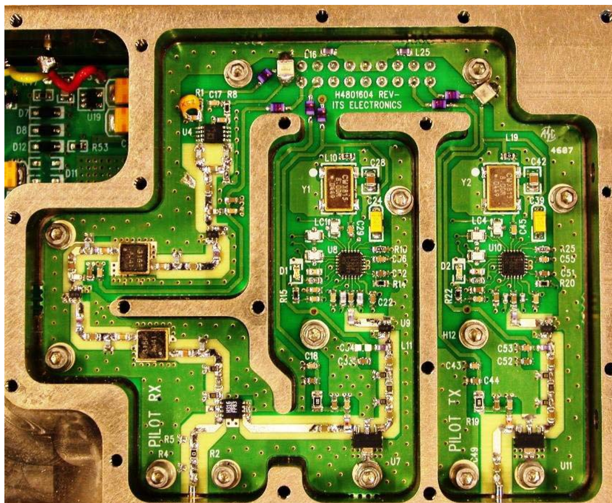
Figure 12 Top view of pilot tone transceiver board
