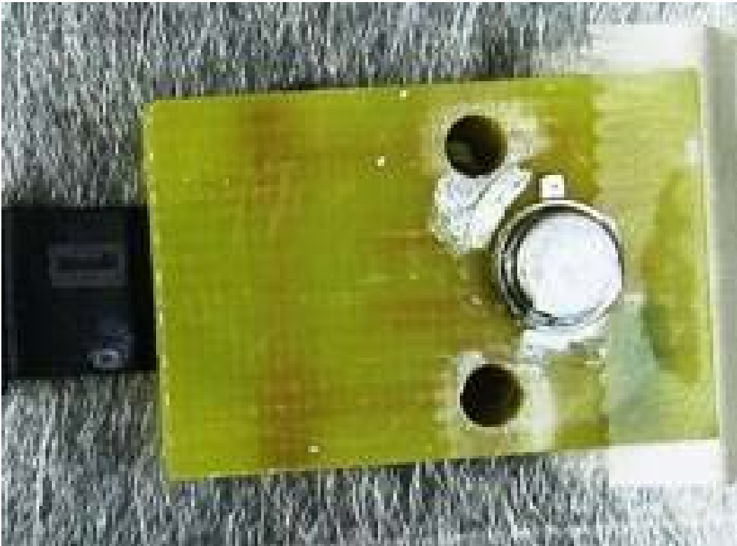
Figure 10 Top view of temperature sensor board
