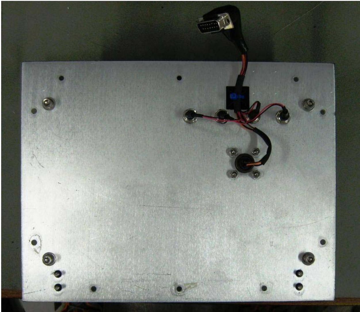
Figure 3 Front Panel inner side
