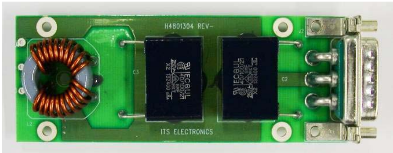
Figure 18 Bottom view of input AC filter board
