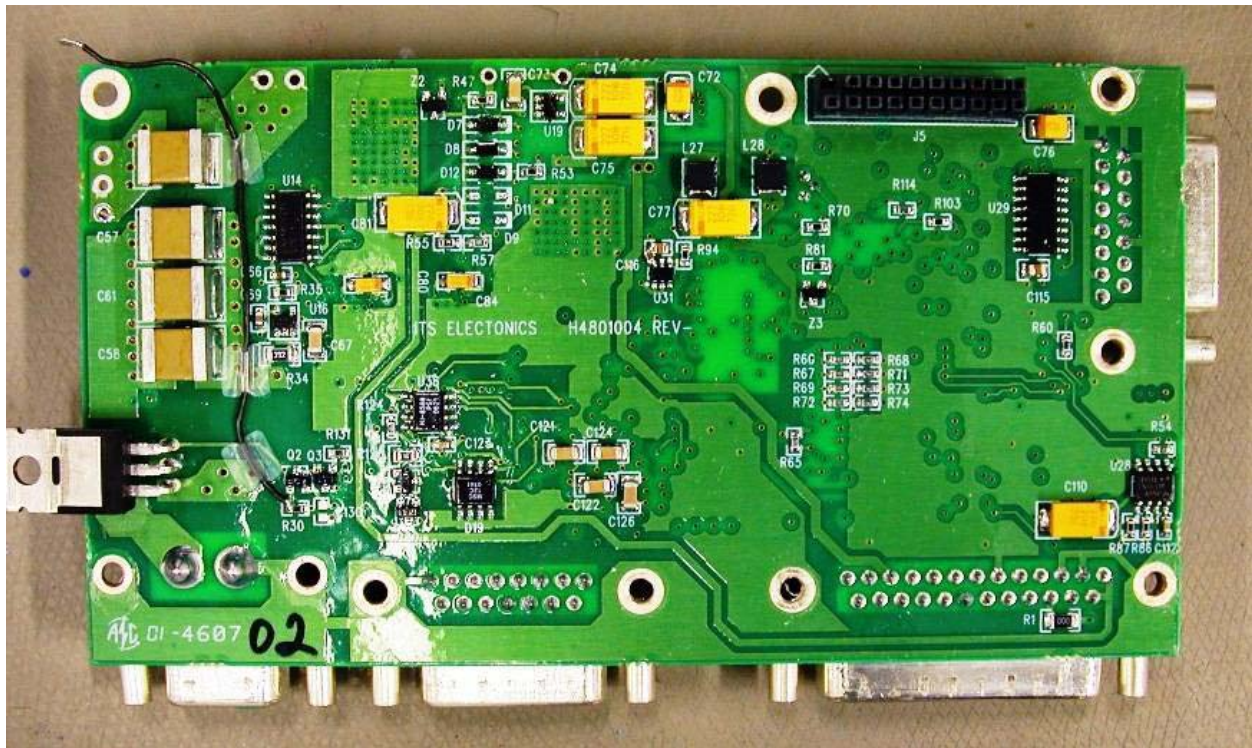
Figure 15 Bottom view of controller board
