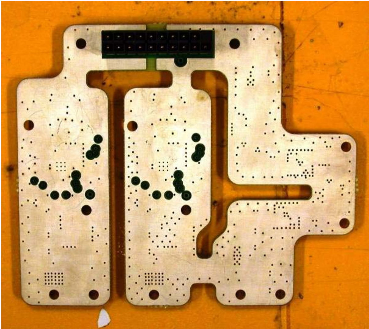
Figure 13 Bottom view of pilot tone transceiver board
