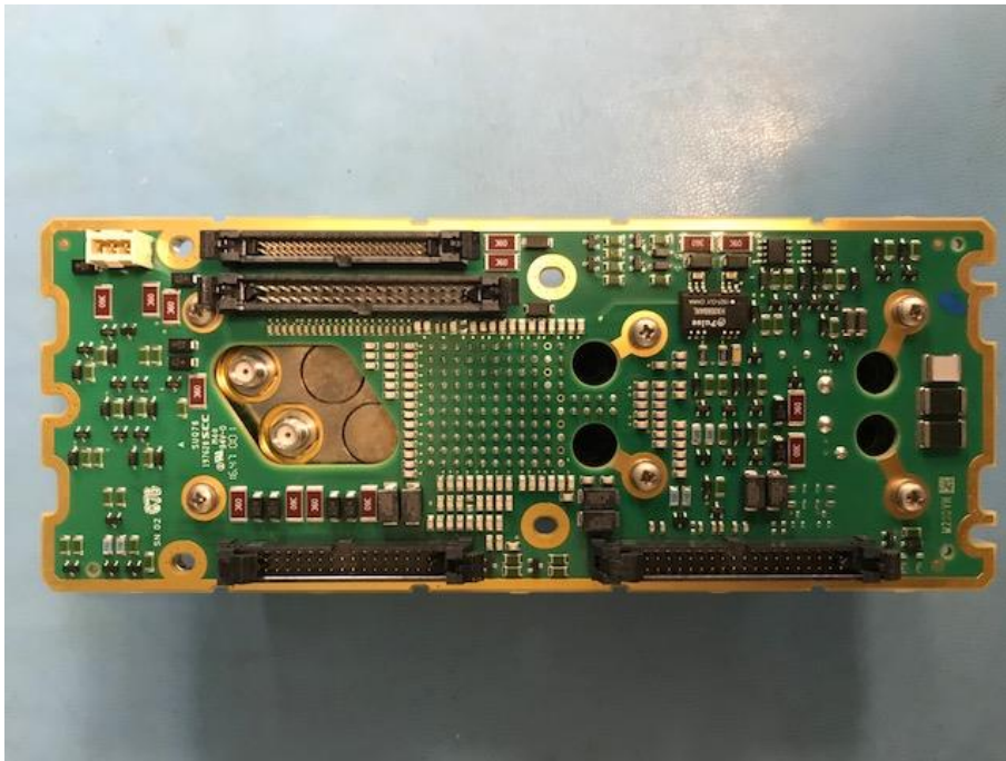
Image 6- Backplane Card Front
