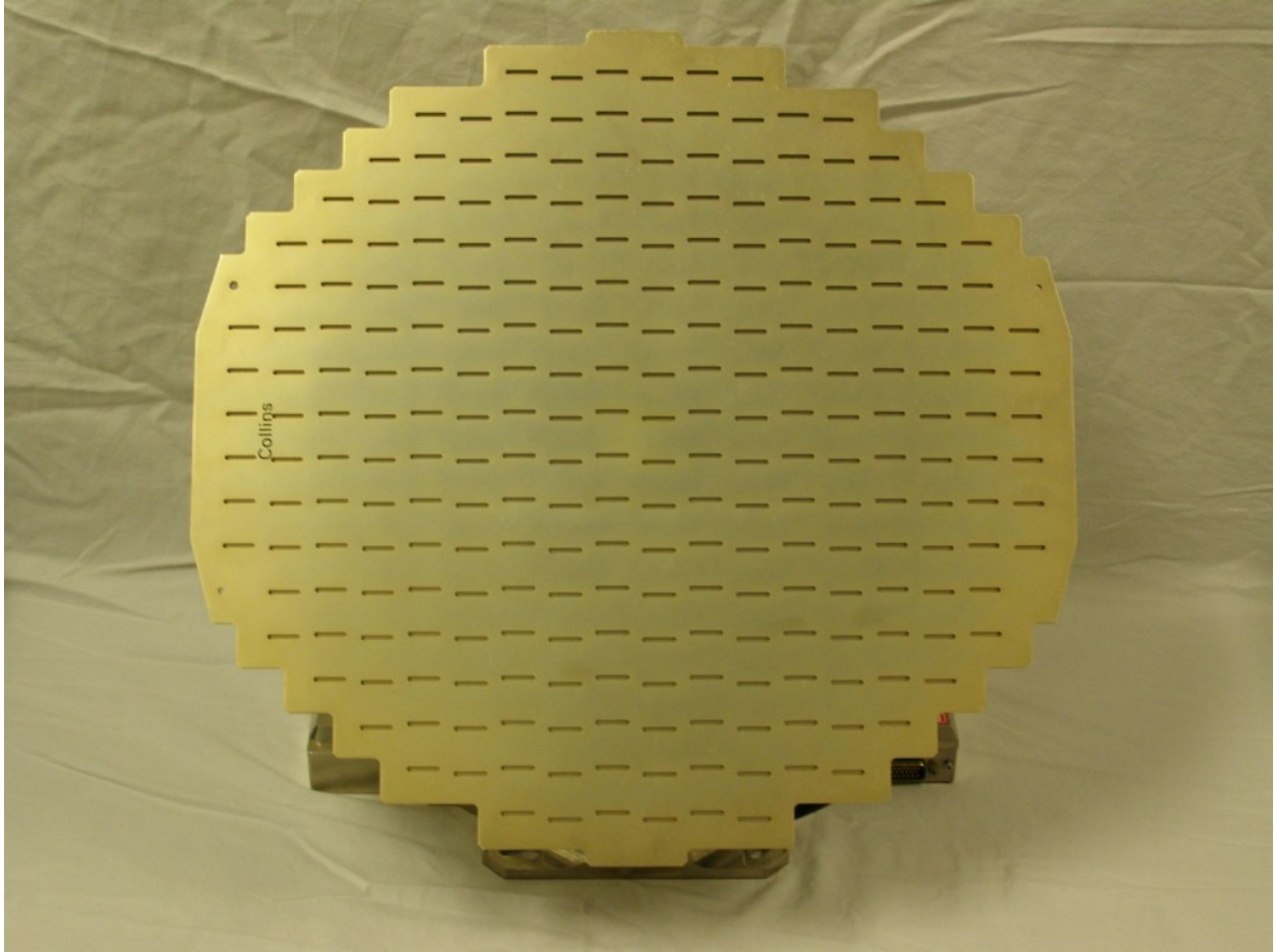
Figure C-3 – RTA-4218 External Photograph – Antenna
