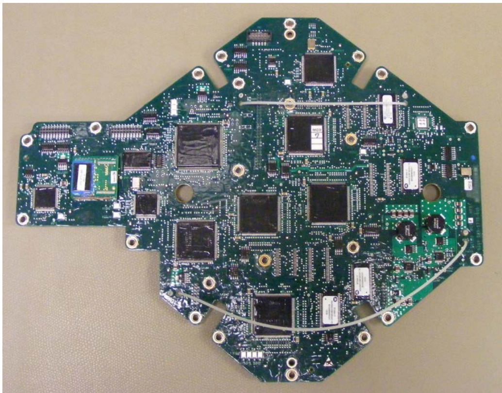
Figure I-4 – System Processor - Top
