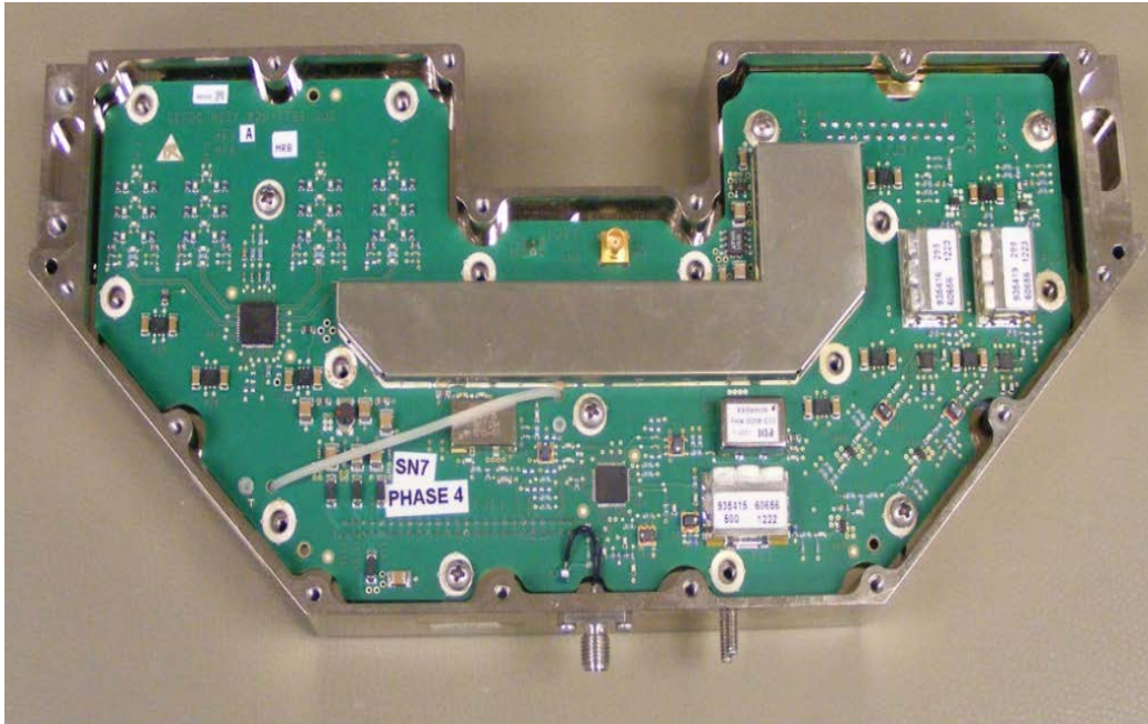
Figure I-3 – Digital Receiver/ Frequency Source Chassis 2
