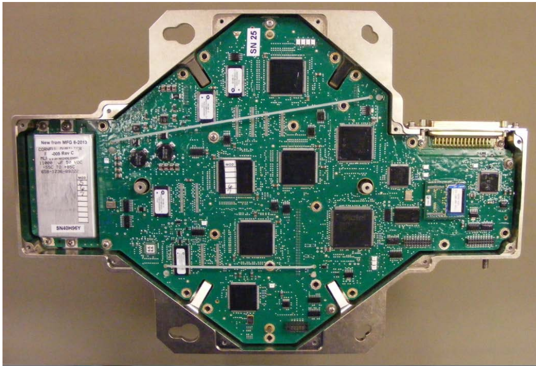
Figure I-1 – Base Assembly View
