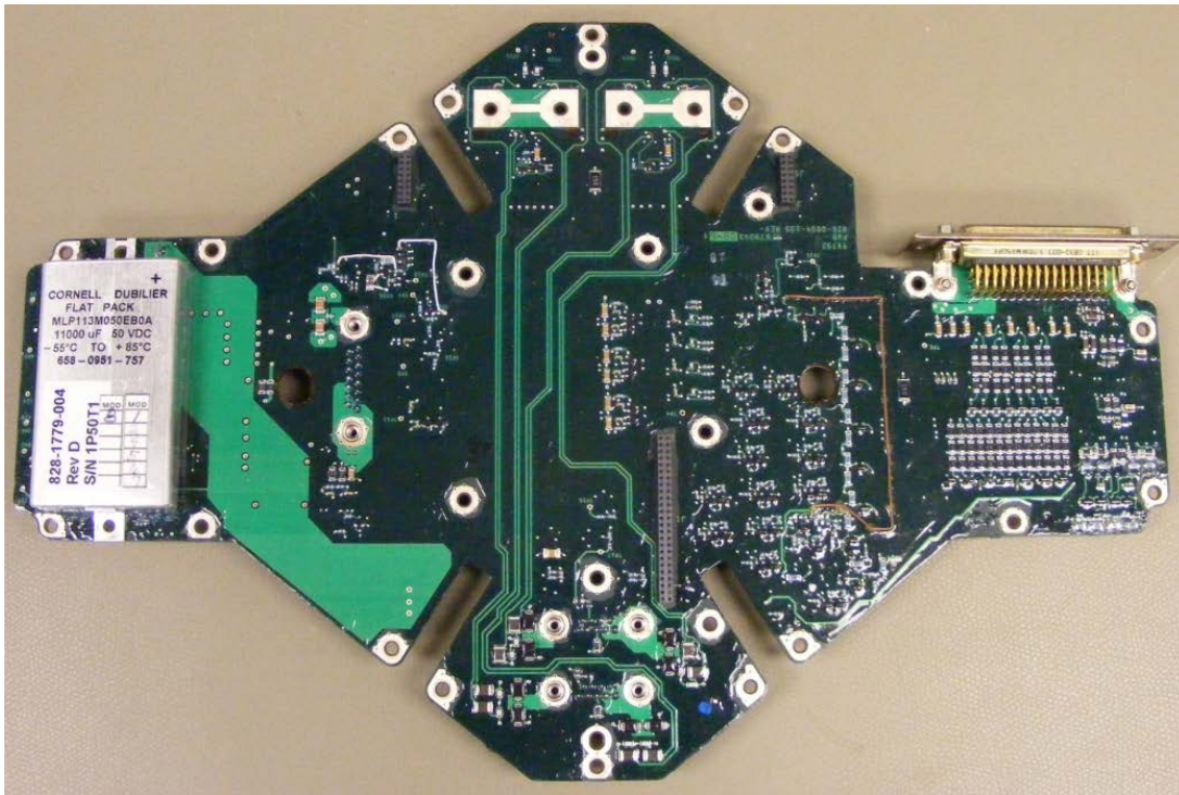
Figure I-7 – Power Supply – Bottom
