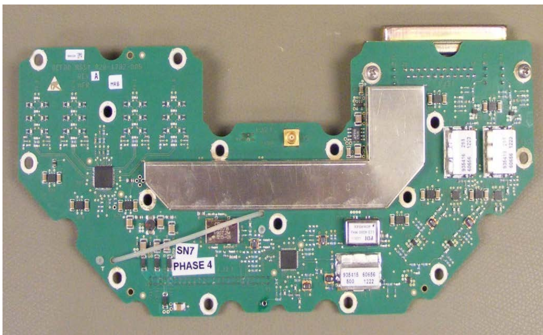
Figure I-10 –Frequency Source - Top
