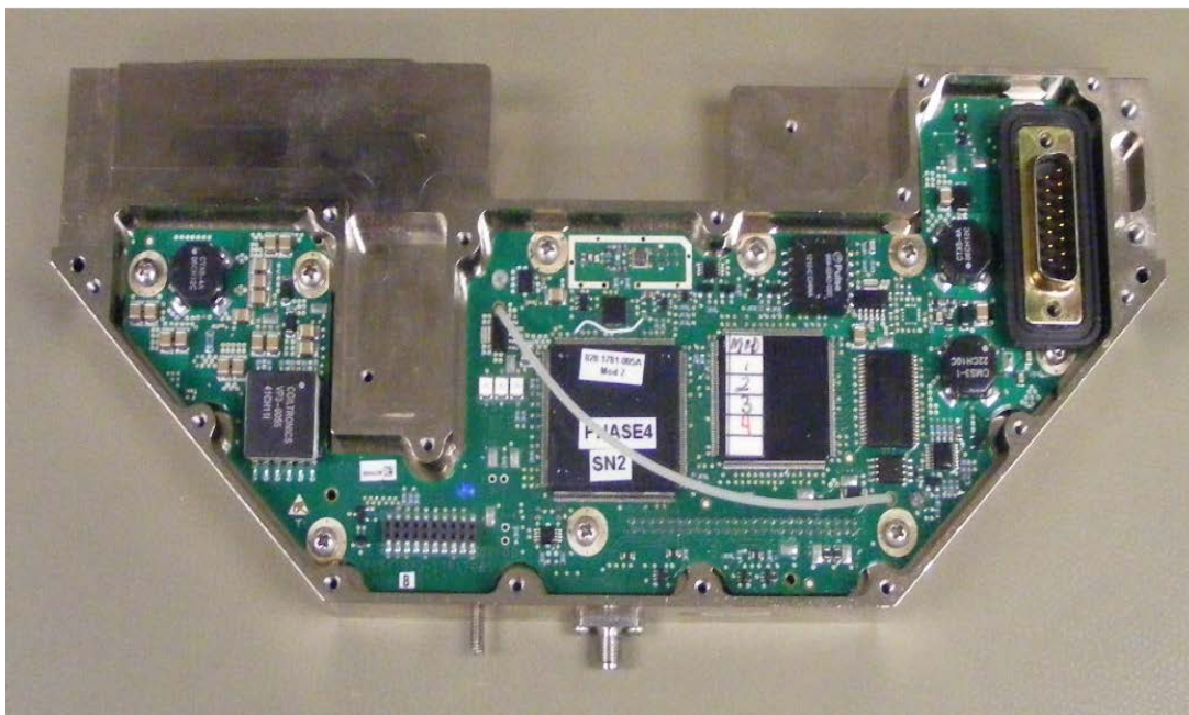
Figure I-2 – Digital Receiver/ Frequency Source Chassis 1
