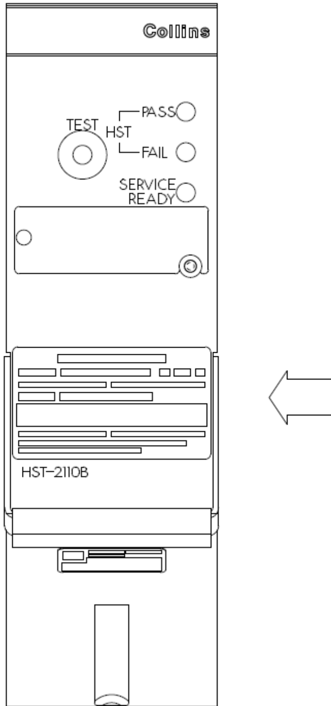
Figure 2 - HST-2110B Front Panel showing nameplate location
